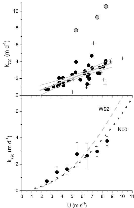
Fig. 6. Wind speed dependence of computed gas transfer coefficient normalized to Sc=720 . Top panel – best quality 1-h k values (closed circles) and lower quality k values (plus signs). The solid gray lines are a linear fit to the data with 95% confidence bands. Bottom panel – k values binned in 1 \text{ m s}^{-1} intervals. Error bars are \pm 1 s.e. Gas transfer parameterizations of Wanninkhof (1992; W92 dashed gray line), and Nightingale et al. (2000a; N00, dotted black line), normalized to Sc=720 are also shown. Gray closed circles indicate outlier points discussed in text.
