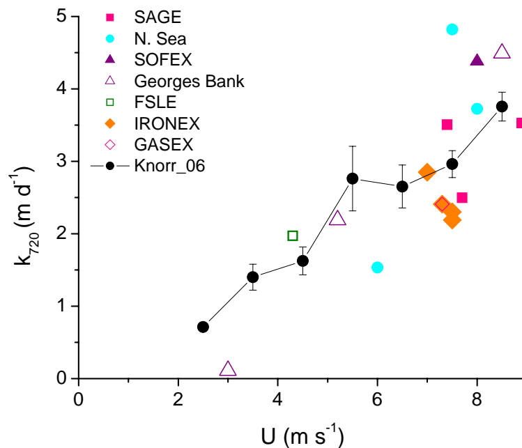
Fig. 9. Comparison between k_{720} for DMS measured in this study and those measured by various dual tracer experiments. The Knorr_06 data has been binned by wind speed and error bars represent \pm 1 s.e. All the data has been normalized to a Sc=720 .
