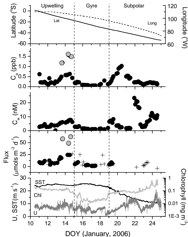
Fig. 4. Time series of shipboard data. From top: (a) Cruise track latitude (solid) and longitude (dashed), (b) DMS atmospheric mixing ratio, (c) DMS oceanic concentration, (d) DMS air/sea flux, in which closed circle represent the highest quality data used to compute k and plus signs are other fluxes discussed in text, (e) Sea surface temperature (solid black), chlorophyll concentration (solid light grey), and horizontal wind speed (solid dark grey). The vertical dashed lines indicate the upwelling, gyre, and subpolar front regions of the cruise. Grey closed circles indicate outlier points discussed in text.
