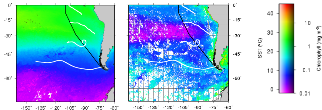
Fig. 3. The cruise track superimposed on Modis data. Left panel – SST ( ^{\circ}\text{C} ). Right panel – chlorophyll ( \text{mg m}^{-3} ). Solid white lines are 5 day surface air mass back trajectories.
