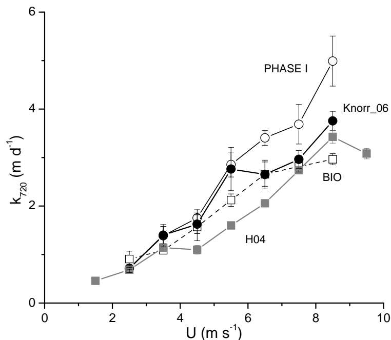
Fig. 7. Wind speed dependence of computed gas transfer coefficients from this work (solid black circles), the PHASE I (open circles) cruise, H04 (solid grey squares), and the BIO cruise (open squares), normalized to Sc=720 . All cruises binned by wind speed. Error bars represent the standard error of the mean (if error bars are not visible they are the size of the symbol).
