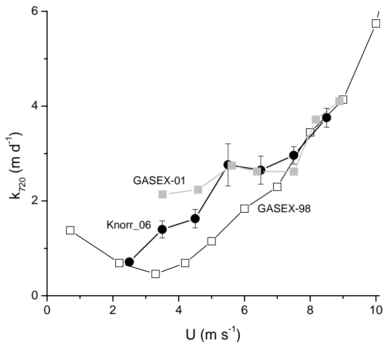
Fig. 8. Wind speed dependence of computed gas transfer coefficients from this work (solid black circles), the GASEX-98 (McGillis et al., 2001) cruise (open squares), and the GASEX-01 (McGillis et al., 2004) cruise (grey closed squares), normalized to Sc=720 . All cruises binned by wind speed. Error bars represent \pm 1 s.e.
