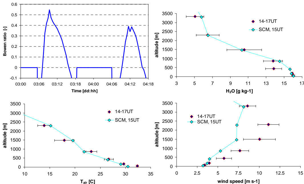
Fig. 2. Evaluation of micro- and PBL meteorology. Figure 2a shows the simulated Bowen ratio for 3–4 October with a daytime average over land of \sim 0.13 . Figure 2b shows the comparison of the simulated versus observed water vapor profiles ( \text{g kg}^{-1} ) over land up to 3.5 km altitude. The observed water vapor reflects the average and standard deviation of all measurements collected between 4.5 and 5.5^\circ N and 52 – 56^\circ W for 14:00–17:00 UT. The simulated profile refers to 3 October at 15:00 UT (12:00 LT). Figures 2c and d, as Fig. 2b but for air temperature and wind speed, respectively.
