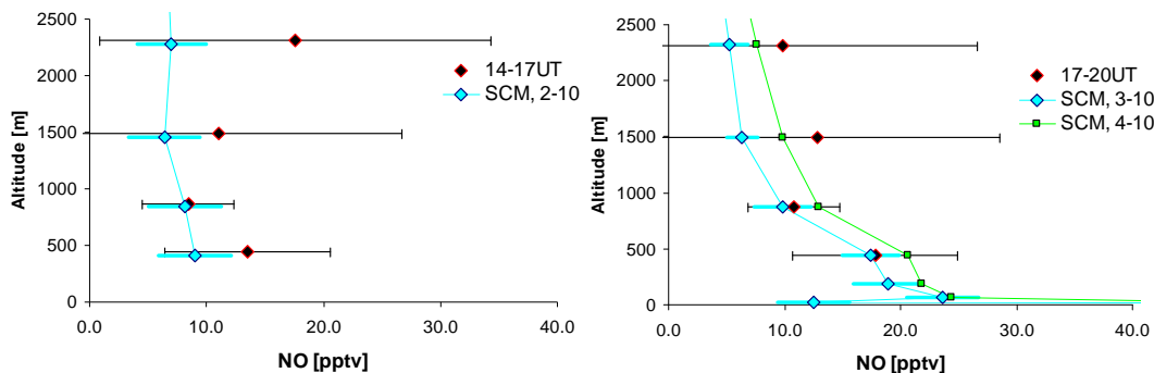
Fig. 5. Simulated and observed NO mixing ratio (pptv) profiles over the ocean from about 440–2500 m altitude, on 2 October 14:00–17:00 UT (a) and over land, 17:00–20:00 UT for 3–4 October (b) also including the mixing ratios below 440 m including the canopy mixing ratios which actually reach a maximum up to \sim 200 pptv in the canopy-soil layer.
