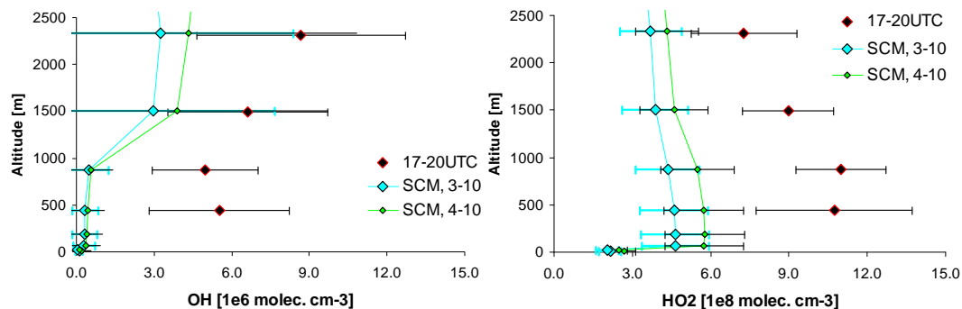
Fig. 17. Simulated and observed OH (a) and HO 2 (b) concentration ( 10^6 and 10^8 molecules \text{cm}^{-3} , respectively) profiles over land, 17:00–20:00 UT for 3–4 October also including concentrations below 440 m.
