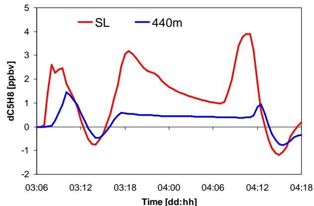
Fig. 13. Difference in C_5H_8 mixing ratios (ppbv) in the surface layer (SL) and the middle of the PBL ( \sim 440 m) for the same integrated emission fluxes simulated with the G95 and MEGAN implementation in the SCM.
