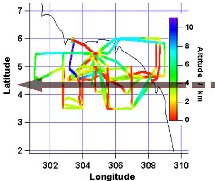
Fig. 1. Transect along which the SCM has been advected by a wind speed of 6.5 \text{ m s}^{-1} for a reference height of 1250 m, from 45^\circ to 60^\circ W along 4.5^\circ N. The duration of the simulation is 3 days using a time step of 60 s, which represents a distance per time step of \sim 300 m. Also shown are the measurement flight tracks with the colors indicating altitude.
