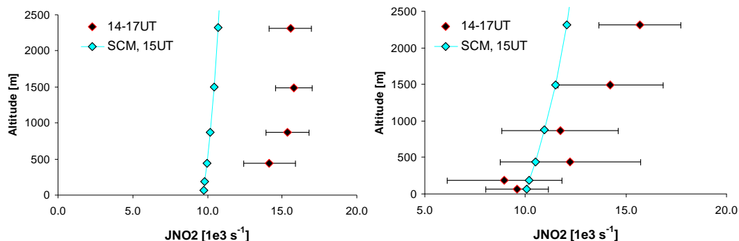
Fig. 6. Simulated and observed \text{NO}_2 photolysis rates ( 10^3 \text{ s}^{-1} ) profiles over the ocean (a) and over land (b) up to 2500 m altitude. The observations reflect the average and standard deviation of the 14:00–17:00 UT observations whereas the simulated profiles reflect the 15:00 UT (12:00 LT) profile.
