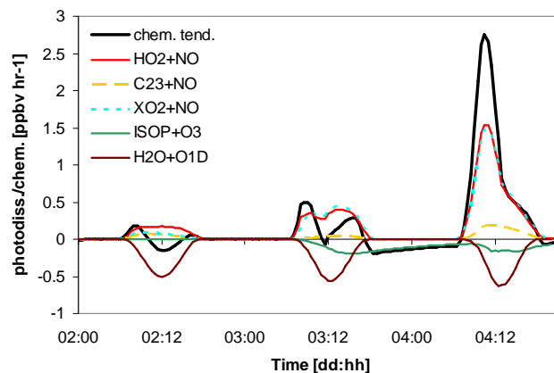
Fig. 10. Simulated \text{O}_3 surface layer chemical tendency and the different production and destruction terms ( \text{ppbv h}^{-1} ) from 2–4 October. Only the reactions with a tendency >5\% of the difference between the minimum and maximum net chemical tendency are shown. C23 in the legend refers to peroxy acetyl radical ( \text{CH}_3\text{C}(\text{O})\text{OO} ) whereas XO2 represents the NO to \text{NO}_2 operator in the chemistry scheme.
