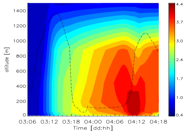
Fig. 16. Simulated HCHO mixing ratios (ppbv) over land on 3–4 October, up to 1500 m. The black dashed line denotes the diagnostic PBL height.
