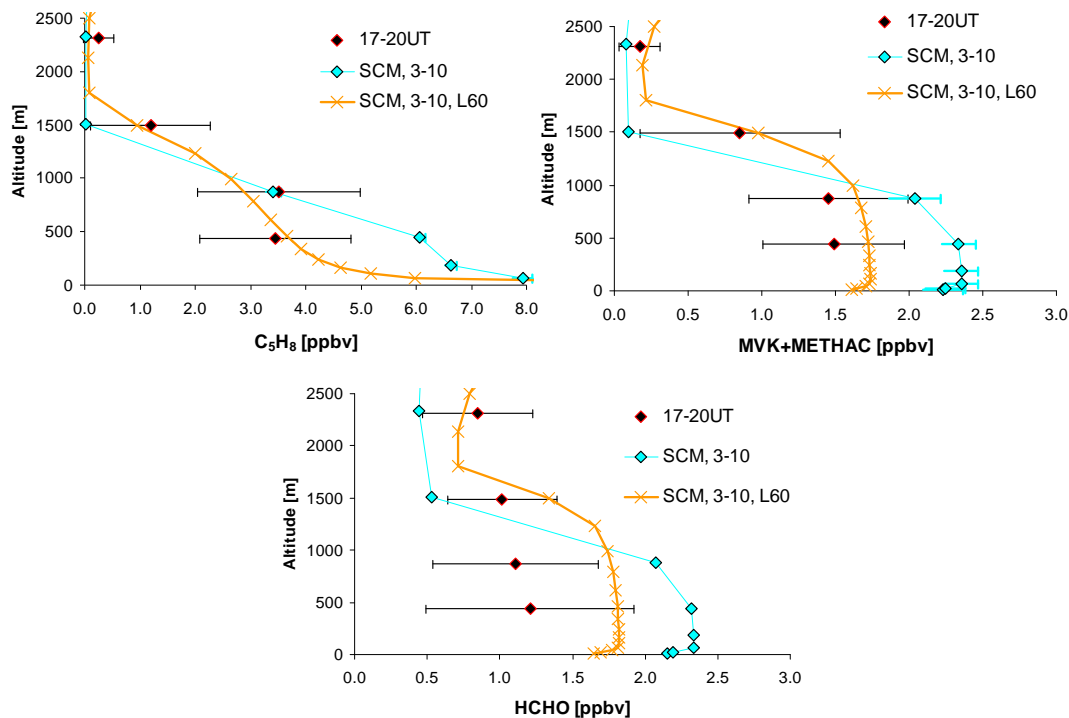
Fig. 19. Simulated and observed C_5H_8 (a) MVK+MACR (b) and HCHO (c) mixing ratio profiles over land, 17:00–20:00 UT for 3 October, showing the simulated mixing ratios for the default L19 and the L60 model resolution.
