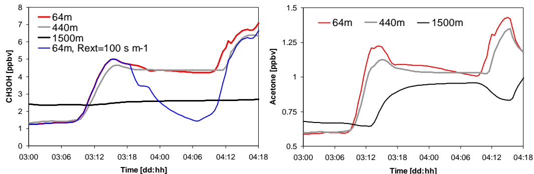
Fig. 4. Simulated CH 3 OH and acetone mixing ratios (ppbv) for 3–4 October over land for the compensation point approach with the thick red, grey and black line showing the mixing ratios in the SL, at ~440 m and around the top of the CBL, respectively. The blue line in Fig. 4a shows the simulated SL mixing ratio of CH 3 OH for an enhanced nocturnal removal efficiency using R_{\text{ext}}=100 \text{ s m}^{-1} .
