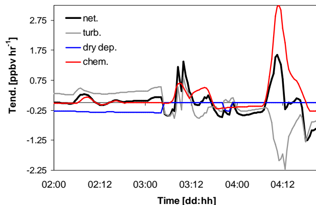
Fig. 9. Simulated surface layer net- and process tendencies ( \text{ppbv h}^{-1} ) that control the perturbations in surface layer \text{O}_3 mixing ratios from 2–4 October. “turb” refers to the turbulent transport tendency, “dry dep” to dry deposition tendency, which equals zero over land since there the dry deposition acts upon the in-canopy and not the surface layer concentrations, and “chem” refers to the chemical production/destruction tendency.
