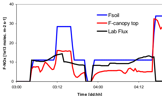
Fig. 7. Simulated soil NO (blue) and canopy-top NO x flux (red) ( 10^{13} molecules m^{-2} s^{-1} ), indicating the fraction of the soil NO emissions that is actually released to the atmosphere. The zero fluxes during the night of 3–4 October indicate the passage of the column over lake Brokopondo. Also shown are soil NO emission fluxes (black) based on laboratory measurements of the emissions from Suriname forest soil samples constrained with the simulated soil temperature and moisture.
