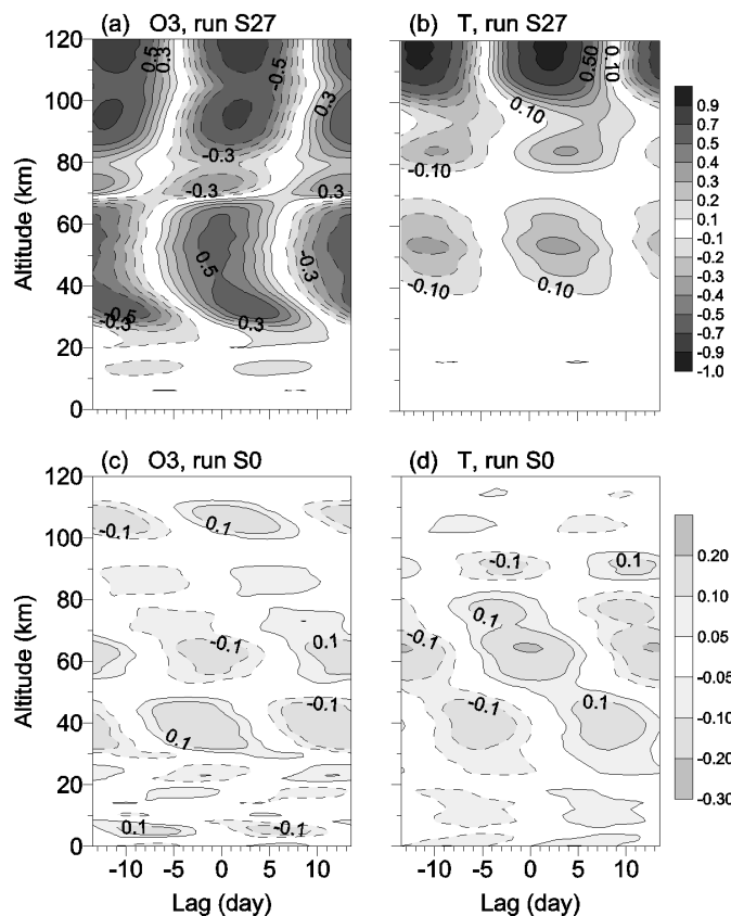
Fig. 2. Correlation coefficients between (a) ozone and (b) temperature near-27-day variations and the 27-day sinusoidal solar forcing for the tropical belt 20^{\circ}\text{S} – 20^{\circ}\text{N} . (a, b) Simulation with applied 27-day forcing, (c, d) simulation without 27-day forcing. All shown correlation coefficients are statistically significant at the 95% level.
