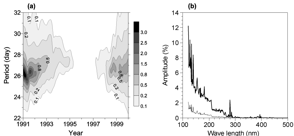
Fig. 1. (a) Spectral density of the solar flux at 205 nm as a function of time calculated using 2-year running windows. Units: (\text{mW}/(\text{m}^2 \text{nm}))^2 \text{ day} . (b) Mean amplitudes of the 27-day (thick curve) and 13.5-day (thin curve) harmonics of the solar extraterrestrial flux as a function of wave length, computed for the period January to June 1990 relative to the mean fluxes for this period.
