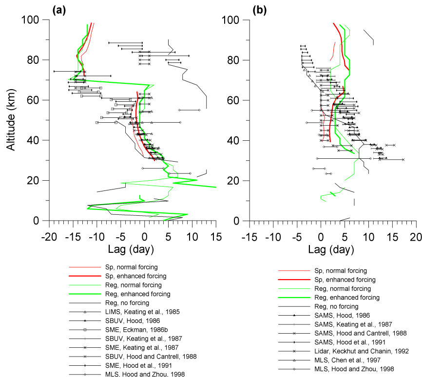
Fig. 13. Comparison of the time lags of the (a) ozone and (b) temperature responses calculated by the model for 20^{\circ}\text{S} – 20^{\circ}\text{N} (color and black curves) with observations in the tropical region (horizontal bars). Red curves correspond to the lags derived by the cross-spectral analysis, green curves correspond to the lags derived by the linear correlation analysis for the cases of standard (thin red and green curves) and enhanced (thick red and green curves) forcing. Black curves correspond to the lags of the “response” obtained by the linear correlation method for the case without 27-day forcing.
