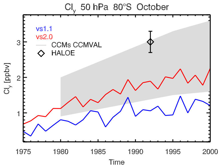
Fig. 12. Time series of total inorganic chlorine Cl_y in October at 50 hPa and 80° S for SOCOL versions vs1.1 (blue line) and vs2.0 (red line). Estimates of Cl_y from HALOE HCl measurements in 1992. The grey area indicates the range of all CCMs participating at CCMVal except SOCOL. Adapted from Fig. 12b from Eyring et al. (2006).
