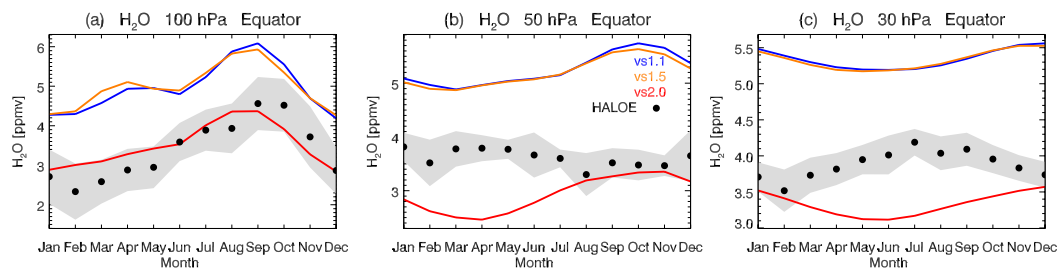
Fig. 10. Seasonal variations of \text{H}_2\text{O} mixing ratios (in ppmv) at Equator averaged over 1990–1999. (a) at 100 hPa, (b) at 50 hPa, and (c) at 30 hPa. The different colours indicate the different model versions as indicated in the centre panel. Black bullets: HALOE observations; grey area: HALOE \pm 1 standard deviation ( \sigma ) about the climatological zonal mean.
