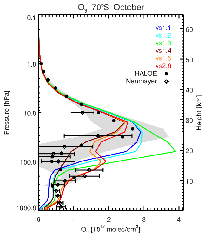
Fig. 8. Profile of zonal mean ozone number densities in 10^{12} molecules/ cm^3 at 70^\circ S in October averaged over 1990–1999. Different colours indicate the different model versions as indicated in the upper right corner. Black bullets: HALOE observations; grey area: HALOE \pm 1 standard deviation ( \sigma ) about the climatological zonal mean. Black diamonds: balloon measurements at the German Neumayer station (Antarctica) with bars indicating \pm 1 standard deviation ( \sigma ) about the climatological mean.
