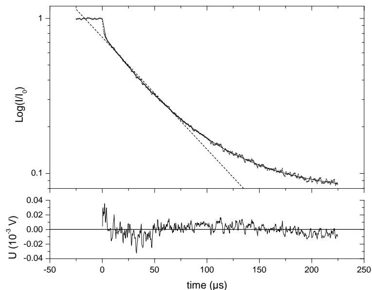
Fig. 2. Ring-down signal averaged from 1000 cycles. Small dots: measurement data. Solid line: multi-exponential fit (0–225 μs). Dashed line: single-exponential fit (5–75 μs). Lower panel: fit residual of multi-exponential fit. Note non-linear decay of \text{Log}(I/I_0) .
