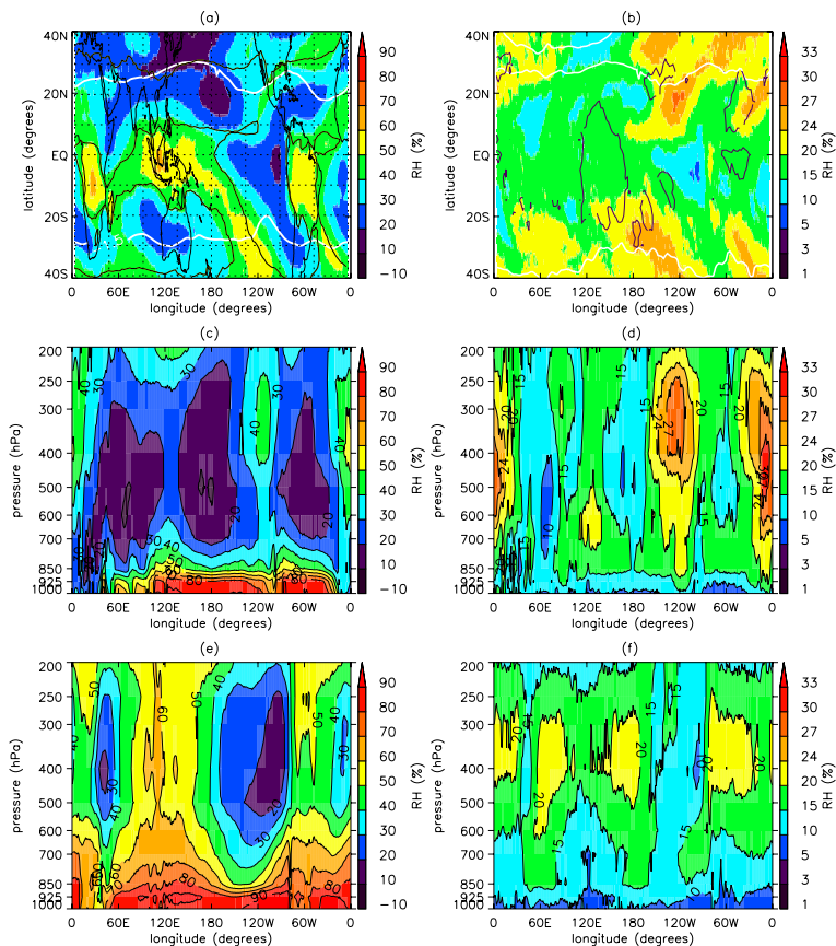
Fig. 1. Climatological distributions of RH. Maps of (a) mean and (b) standard deviation at 250 hPa. Vertical cross sections of (c) mean and (d) standard deviation for average over 15.5^{\circ} N to 25.5^{\circ} N, and (e) mean and (f) standard deviation for average over 5.5^{\circ} S to 5.5^{\circ} N. In (a) white curves are PV = \pm 1.5 PVU contours and black curves are OLR = 240 W/m^2 contours, whereas in (b) white curves are PV = 1.5 PVU contours and black curves are OLR = 70 W/m^2 contours.
