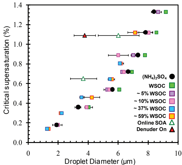
Fig. 8. Droplet sizes of WSOC CCN with s_c equal to the instrument supersaturation (square symbols). Data is obtained from Experiments 1, 2, and 3. Corresponding droplet sizes for (\text{NH}_4)_2\text{SO}_4 (black circles) and SOA CCN (triangles) are also shown.
