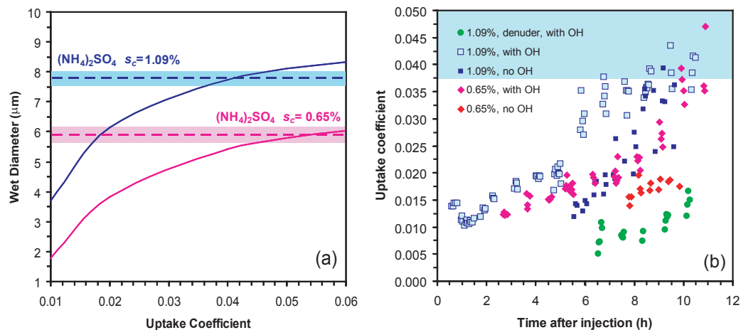
Fig. 10. CFSTGC growth kinetics simulations for data collected during Experiments 1 and 2. (a) Simulated droplet wet diameter at the exit of the CFSTGC as a function of \alpha for CCN with s_c = 1.09\% (blue) and 0.65\% (magenta). The size of activated calibration (\text{NH}_4)_2\text{SO}_4 is also shown for comparison. (b) Inferred water vapor uptake coefficient for the growth kinetic data of Fig. 8. For comparison, the range of inferred \alpha for (\text{NH}_4)_2\text{SO}_4 is shown in the blue shaded area.
