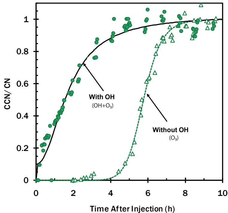
Fig. 3. CCN activity of 100 nm \beta -caryophyllene SOA formed in the presence of OH (circles) and without OH (triangles). Measurements are obtained with the CFSTGC at 1.09% supersaturation from Experiments 1 and 2.
