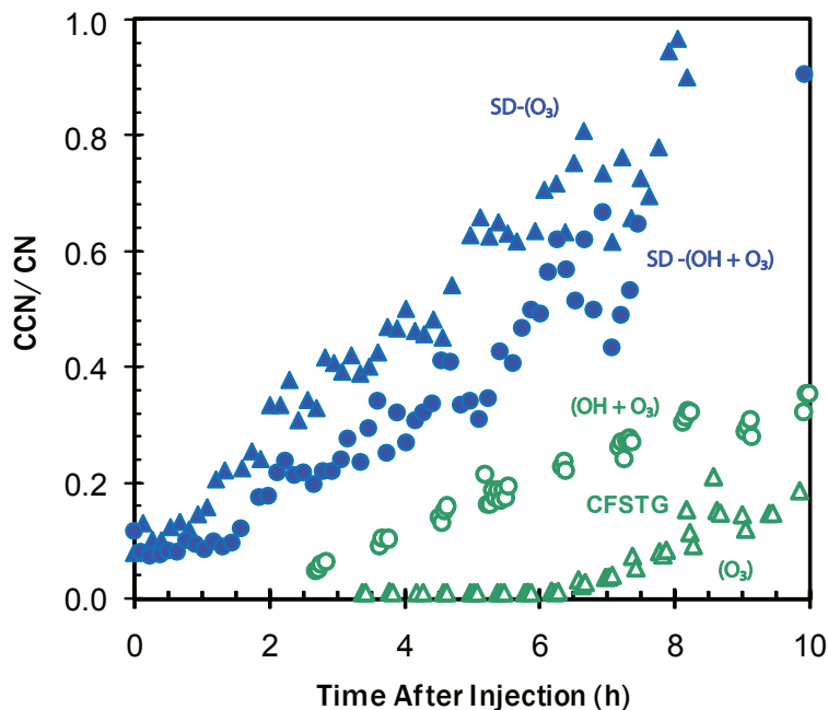
Fig. 2. CCN activity (at \sim 0.6\% supersaturation) of 100 nm \beta -caryophyllene SOA formed in the presence of OH (circles) and without OH (triangles). Data from the CFSTGC and SD CCN counters are presented from Experiments 1 and 2.
