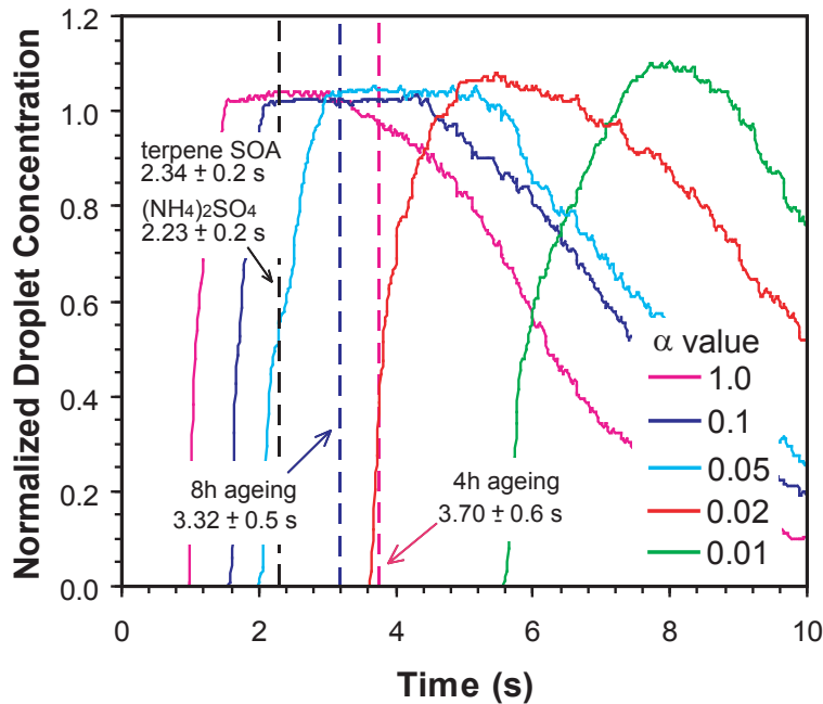
Fig. 9. Simulated droplet concentration within the viewvolume of the SD CCN Counter as a function of time and water vapor uptake coefficient. Peak supersaturation in the counter is 0.6%, and initially is filled with monodisperse ( d=100 nm) \beta -caryophyllene SOA composed of 10% WSOC (with the composition shown in Table 3).
