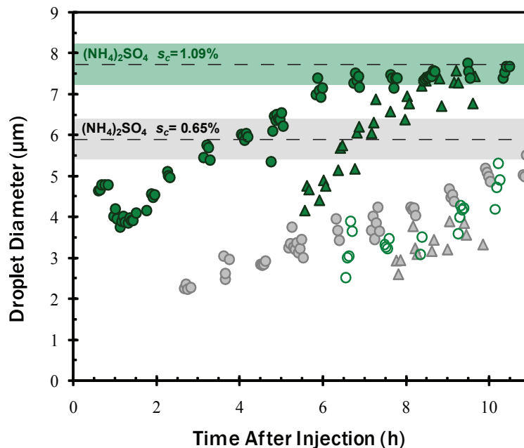
Fig. 7. Droplet diameters of activated SOA particles with s_c equal to the instrument supersaturation, for Experiments 1 (circles) and 2 (triangles). Results are shown for particles with s_c=1.09\% (closed and open) and 0.65\% (grey) supersaturation. Aerosol passed through the thermodenuder is shown with open circles. The shaded green and grey bands represent the average droplet size of calibration (\text{NH}_4)_2\text{SO}_4 with critical supersaturation of 1.09\% ( 7.7 \pm 0.25 \mu\text{m} ) and 0.65\% ( 5.9 \pm 0.25 \mu\text{m} ), respectively.
