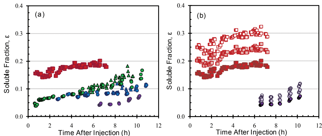
Fig. 6. Inferred soluble fraction as a function of aging for Experiments 1, 2, 4 and 5. Square symbols represent SD measurements; circles and triangles represent CFSTGC measurements for SOA formed in the presence and absence of OH, respectively. (a) \epsilon inferred assuming \sigma=66 \text{ mN m}^{-1} and M_o=156 \text{ g mol}^{-1} for SD measurements at 0.6% (red squares), CFSTGC measurements at 1.09% (green symbols), 0.65% (blue symbols), and, for aerosol passed through the thermodenuder and exposed to 1.09% supersaturation (purple symbols). (b) Sensitivity of \epsilon to \sigma and M_o for data obtained with the SD and (squares) and CFSTGC (circles): \sigma=66 \text{ mN m}^{-1} , M_o=156 \text{ g mol}^{-1} (darkest closed symbols), \sigma=72 \text{ mN m}^{-1} , M_o=156 \text{ g mol}^{-1} (lightly shaded symbols), and, \sigma=66 \text{ mN m}^{-1} , M_o=250 \text{ g mol}^{-1} (open symbols).
