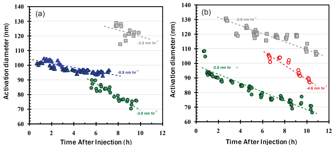
Fig. 4. Activation diameter as a function of time. (a) SOA formed without OH in Experiments 1 (CFSTGC at s_c=0.65\% : grey squares; s_c=1.09\% : green circles), 4 and 5 (SD at s_c=0.6\% : blue triangles). (b) SOA formed with OH in Experiment 2. CFSTGC measurements at s_c=0.65\% (grey squares), and s_c=1.09\% (green circles) are shown. Open red circles correspond to aerosol passed through the thermodenuder prior to exposure to 1.09\% supersaturation in the CFSTGC.
