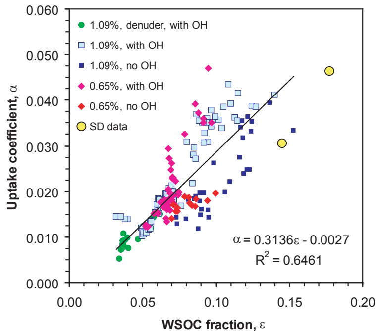
Fig. 11. Inferred \alpha as a function of \varepsilon for all the datasets obtained with the SD (yellow circles) and CFSTGC (all other symbols).
