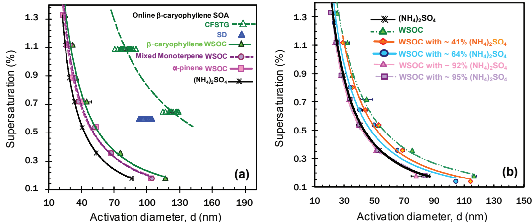
Fig. 5. CCN Activity of WSOC from \beta -caryophyllene SOA collected in Experiment 3. (a) SOA and (\text{NH}_4)_2\text{SO}_4 data are presented for comparison. WSOC from mixed monoterpene and \alpha -pinene hydrocarbon pre-cursors (Engelhart et al., 2008) are also shown. (b) WSOC from \beta -caryophyllene SOA, mixed with (\text{NH}_4)_2\text{SO}_4 .
