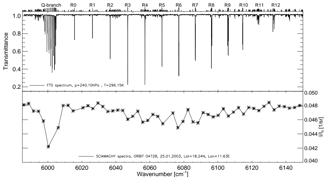
Fig. 1. Example of a recorded FTS methane transmission spectrum at 240.1 hPa and a SCIAMACHY reflectance spectrum over the Sahara. On top of the plot, a stick spectrum of methane in logarithmic scale is depicted to indicate line positions and strengths. In addition, the attribution to Q and R-branch transitions in the 2\nu_3 band is given. Please note that the SCIAMACHY spectrum is not absolute-radiometric calibrated, so only relative variations should be considered. The major absorber in the SCIAMACHY spectrum is \text{CH}_4 but smaller absorptions by \text{CO}_2 and \text{H}_2\text{O} are also present.
