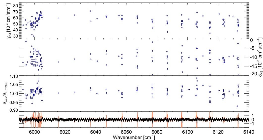
Fig. 5. N_2 -broadening coefficients (upper panel), pressure shifts (middle panel) and ratio of present line intensities compared to HITRAN (lower panel, mean ratio = 1.013) retrieved in the Q-branch and R-branch. The lowest panel again depicts fitting residuals (black line) and residuals assuming HITRAN parameters (red) for the 900 hPa spectra.
