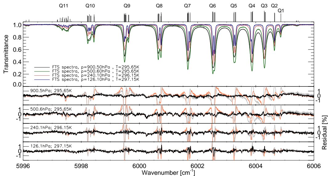
Fig. 2. Fit results of the multi-spectra inversion for the Q branch. The upper panel depicts the N_2 broadened FTS spectra. The lower panels show the fitting residuals for each FTS spectrum separately in black (measured-modelled times 100). The red lines indicate residuals if no changes to the HITRAN database were applied. The gray lines show residuals using the HITRAN database but replacing broadening coefficients with results by Pine (1992, 1997) in the fundamental.
