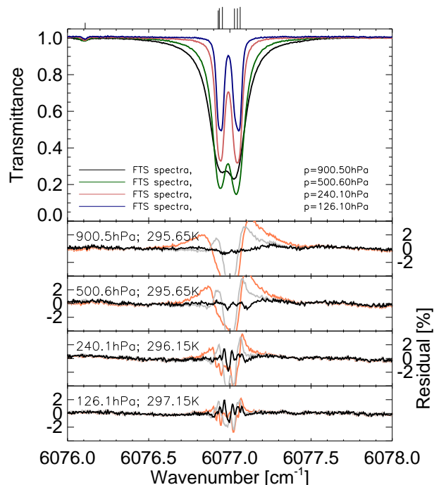
Fig. 4. As in Figs. 2 and 3 but for the R6 manifold with six strong transitions. The sum of the measured intensities in the manifold is greater by only 1.2% compared to the Margolis (1988) values. In contrast, the average of measured widths is 19% smaller than the average of default widths applied in HITRAN. The residuals seen in the fit of the lowest pressure spectrum could arise from combined inaccuracies of the retrieved positions, relative strengths, widths, the presence of weak transitions not included in the database or effects of non-Voigt line-shapes.
