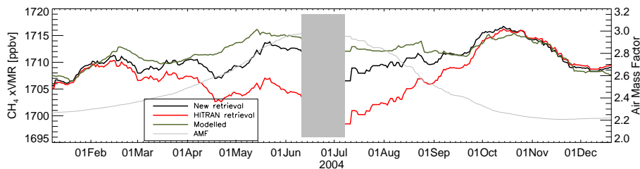
Fig. 9. Timeseries of SCIAMACHY methane column averaged mixing ratios over Australia in 2004. Concurrent CO 2 retrievals have been used as proxy for the light path (Frankenberg et al., 2005a, 2006), using CarbonTracker by NOAA for model CO 2 profiles to minimise the impact of CO 2 variations. The air mass factor is shown in gray and a decontamination period ( \pm 10 days) of the satellite is overlaid as grey box. Time series data have been smoothed with a 30-day running time-average (box filter) and spatially averaged over the entire Australian continent between -20 and -30 degree latitude.
