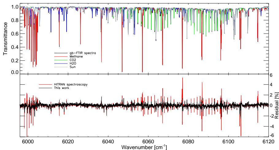
Fig. 7. Spectral fit of a ground based FTIR measurement in Bremen, Germany, measured with 45 cm optical path difference at 63.51^\circ SZA on 3 July 2006. The upper panel shows the spectrum and the contributions of the individual gases as well as the sun. The lower panel depicts the fit residuals (Measured-modelled) for the spectroscopic parameters from this study and HITRAN, respectively.
