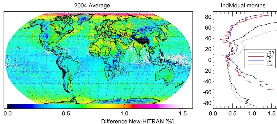
Fig. 8. Impact of spectroscopy on methane retrievals by SCIAMACHY onboard ENVISAT. The left panel shows the differences averaged over the year 2004 (New spectroscopy – HITRAN spectroscopy) on a 1 by 1 degree grid. The right panel shows the mean latitudinal differences for individual months.
