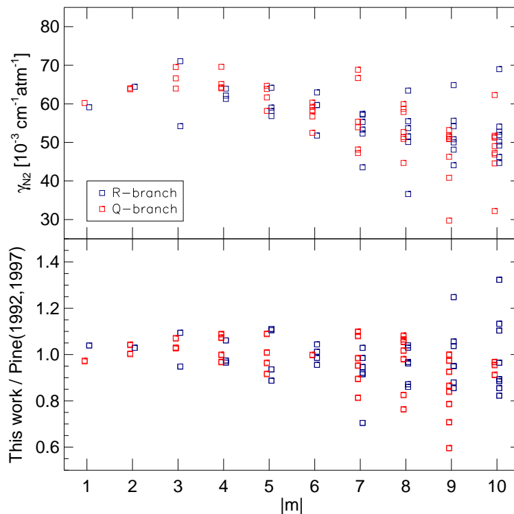
Fig. 6. Measured N_2 -broadening coefficients retrieved in the Q and R branch as a function of |m| , where |m| is the lower state J for Q transitions and the upper state J for R branch lines. For easier identification, Q and R branches are slightly shifted. The lower panels depicts the difference of the retrievals as compared to Pine (1992, 1997).
