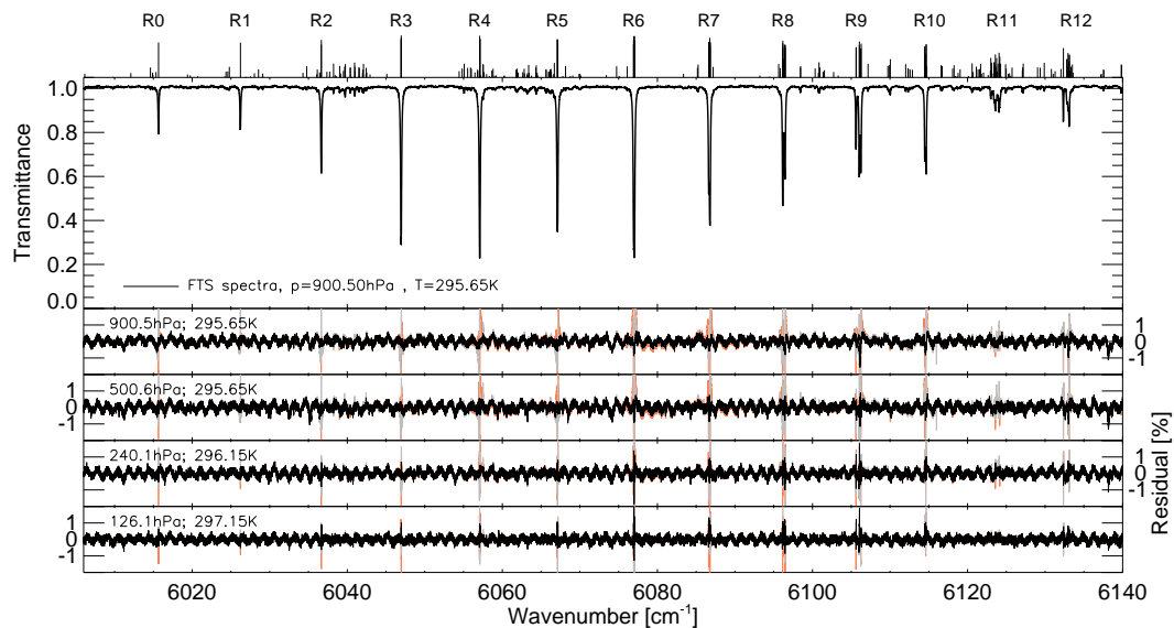
Fig. 3. As in Fig. 2 but for the R-branch.
