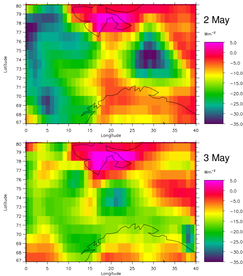
Fig. 9. Radiative forcing of the episode relative to an aerosol situation in the spring with \text{AOD}=0.05 .
