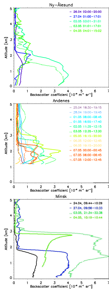
Fig. 8. Height profiles of backscatter coefficients of aerosols from ground based observations at the sites in Ny-Ålesund, Andenes (ALOMAR), and Minsk during spring 2006.
