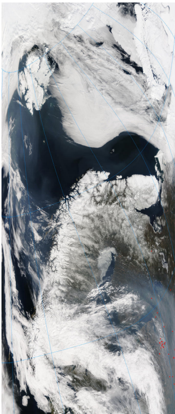
Fig. 2. The plume is clearly seen in the MODIS pictures of northeast Europe and Northern Scandinavia. The red dots in Eastern Europe indicate fires.
