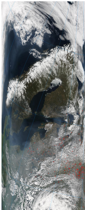
Fig. 2. The plume is clearly seen in the MODIS pictures of northeast Europe and Northern Scandinavia. The red dots in Eastern Europe indicate fires.
