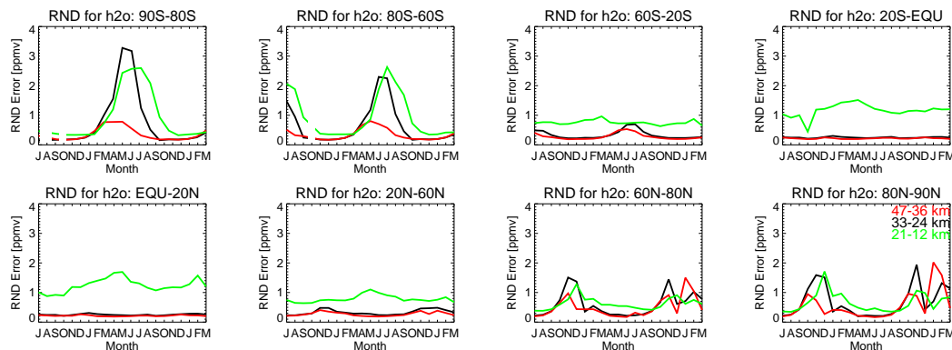
Fig. 1. Time series of the precision derived from MIPAS L2 data for \text{H}_2\text{O} [ppmv] from July 2002 to March 2004, split in eight latitude bands. The red line shows the precision averaged between 47 km and 36 km tangent heights, the black line between 33 km and 24 km and the green line between 21 km and 12 km. The gaps in the southern hemisphere in July–August 2002 and October 2002 are caused by missing Antarctic L2 profiles.
