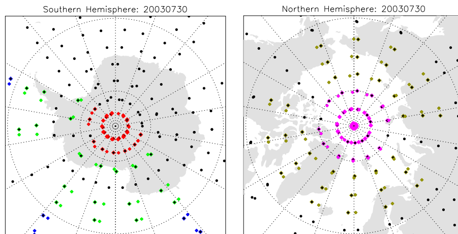
Fig. 5. Locations of the ESA L2 profiles of MIPAS for 30 July 2003. Colored points represent positions where orbital tangent tracks intersect when two observations are made of the same atmosphere 6 h apart (red for South Pole and magenta for North Pole) and 12 h apart (green, blue and yellow). The black orbit intersections in the South Pole regions come from observations made more than 12 h apart.
