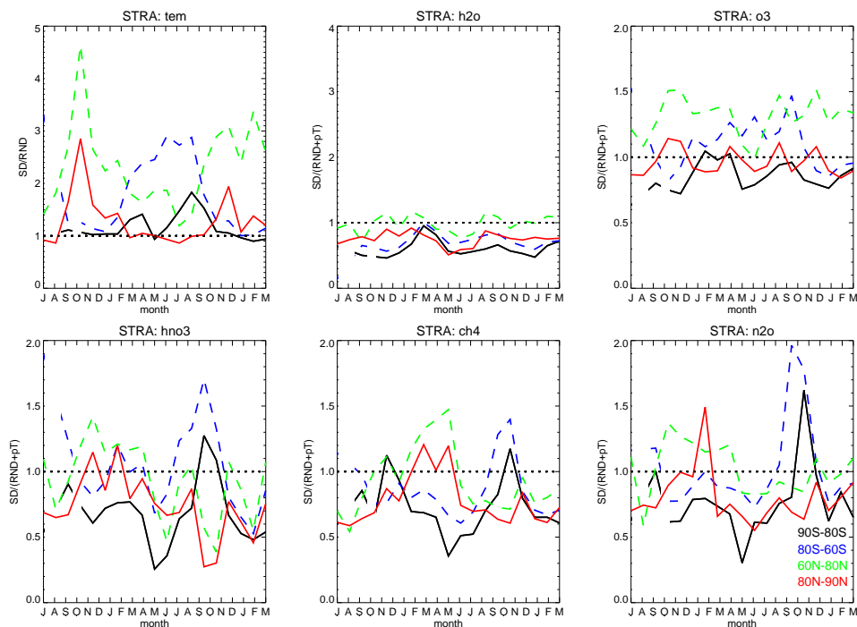
Fig. 7. Time series of the ratio standard deviation(SD)/precision for each species derived from the analysis of the matching ascending/descending profile pairs from July 2002 to March 2004. This ratio is computed averaging the whole standard deviation/precision profiles down to the nominal tangent height of 15 km (i.e. stratosphere). For each species, Black indicates 80S–90 S, Red 80,N–90 N, Blue 60 S–80 S and Green 60 N–80 N regions as a function of time. Solid lines indicate matching pairs within 6 h, while dashed lines within 12 h. The precision includes the precision values given in the MIPAS L2 data and the pT error propagation component for the VMR target species plots.
