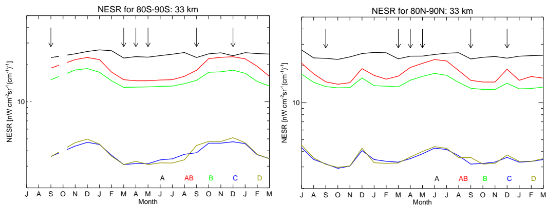
Fig. 4. Time series of NESR at 33 km tangent altitude for the 5 different spectral bands (A: 685\text{--}970\text{ cm}^{-1} , AB: 1020\text{--}1170\text{ cm}^{-1} , B: 1215\text{--}1500\text{ cm}^{-1} , C: 1570\text{--}1750\text{ cm}^{-1} , D: 1820\text{--}2410\text{ cm}^{-1} ). Southern Hemisphere gaps correspond to the missing Antarctic L2 profiles for July–August 2002 and October 2002. Arrows indicate decontamination events.
