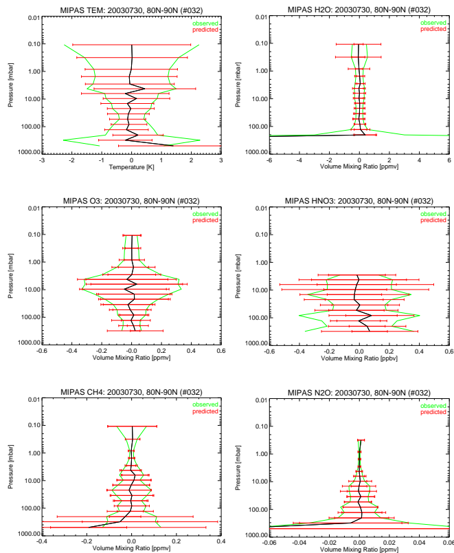
Fig. 6. Example of polar summer comparisons at 80N–90N latitudes for 30 July 2003. It shows comparisons for temperature (top left), H 2 O (top right) O 3 (middle left), HNO 3 (middle right), CH 4 (bottom left) and N 2 O (bottom right). The black line is the bias between the matched pairs profiles, the red bars are the precision values (for the VMR plots the pT induced error is included and shown as an additional contribution to the red bars) and the green line is the standard deviation of the ensemble of the matching profile pairs.
