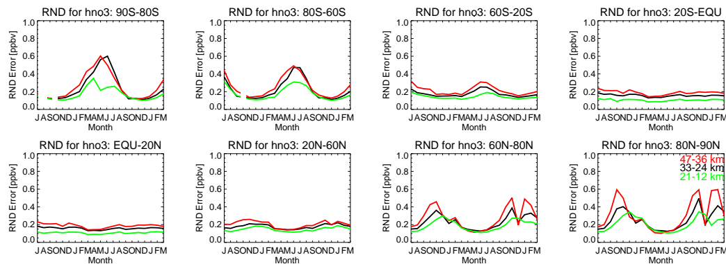
Fig. 2. As Fig. 1, except for \text{HNO}_3 [ppbv].
