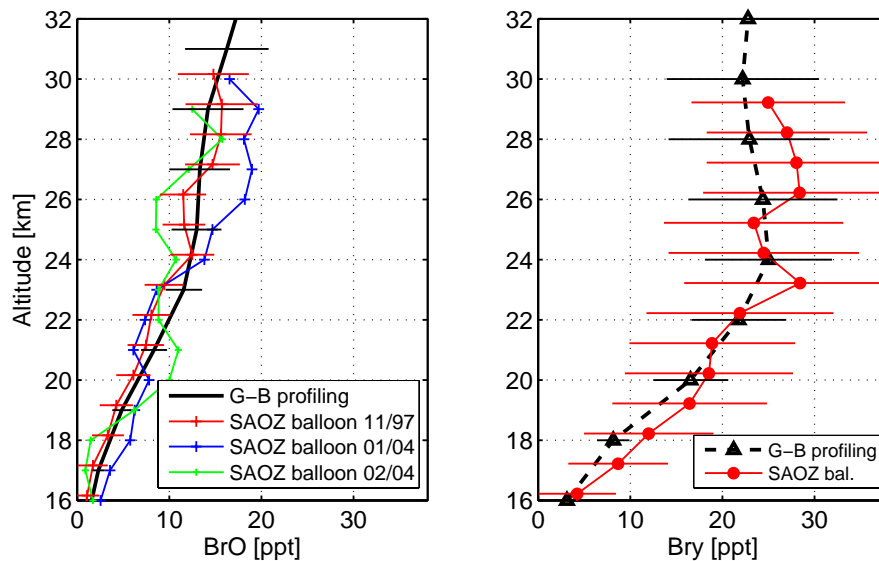
Fig. 9. Retrieved stratospheric BrO profile compared to tropical SAOZ balloon BrO profiles (left plot). Profile of Br y inferred from ground-based BrO profile compared to the SAOZ balloon Br y profile at 22° S, November 1997 (right plot).
