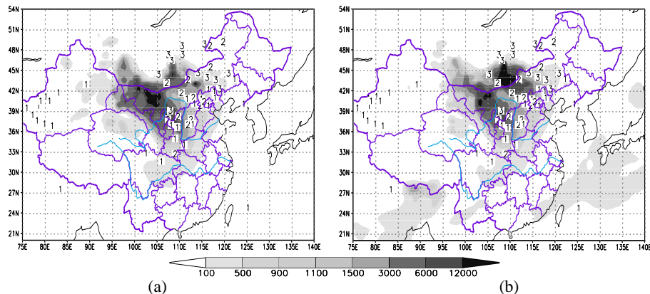
Fig. 4. Comparison of simulated dust concentration distribution (20 March 2002, 03:00 UTC) ( a: result from the original DOFS; b: result from our scheme; 1,2,3 represent actual floating dust, blowing sand and dust storm, respectively; simulated dust concentration is in \mu\text{g}/\text{m}^3 ).
