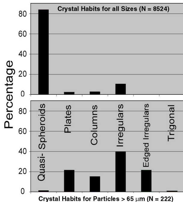
Fig. 8. Comparison of crystal habits for (top) all crystals and (bottom) crystals >65 \mu\text{m} in SVC. Particle habits were classified manually based on CPI images.
