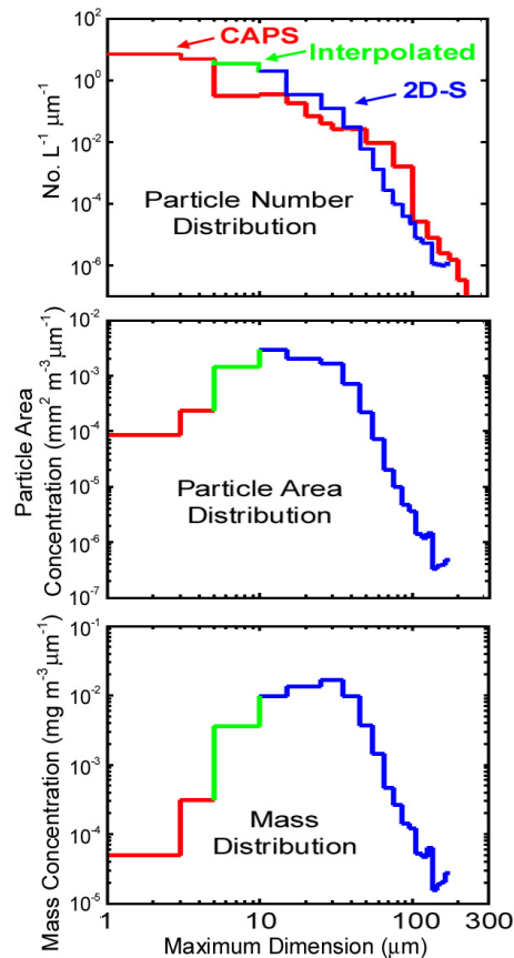
Fig. 9. PSD's of (top) number concentration, (middle) area and (bottom) mass based on \sim 1800 km of WB-57F 2D-S and CAPS measurements collected in SVC. Green trace is interpolated between 5 \mu\text{m} CAPS and 10 \mu\text{m} 2D-S size bins.
