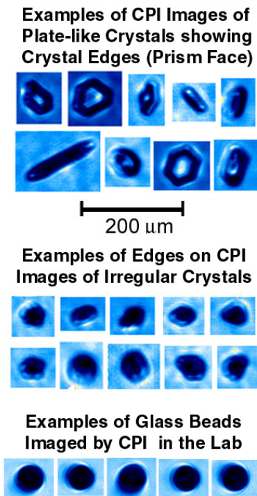
Fig. 7. Examples of CPI images in SVC that show edges (prism faces) of the larger plate-like and irregular crystals, and examples of images of glass beads taken in the laboratory for the sake of comparison.
