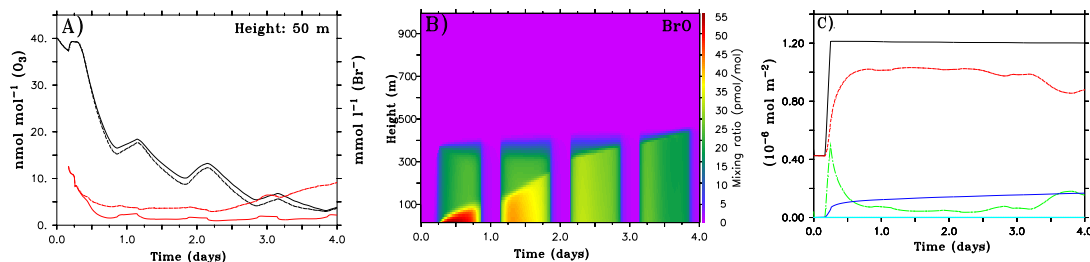
Fig. 16. Run 18 (no-HONO). (A) Comparison between run 18 (dashed lines) and the base run (solid lines) for gas phase \text{O}_3 (black lines in \text{nmol mol}^{-1} ) and FF aerosol bromide (red lines in \text{nmol l}^{-1} ) at an altitude of 50 m. (B) \text{BrO} in run 18, (C) same as Fig. 21 for run 18.
