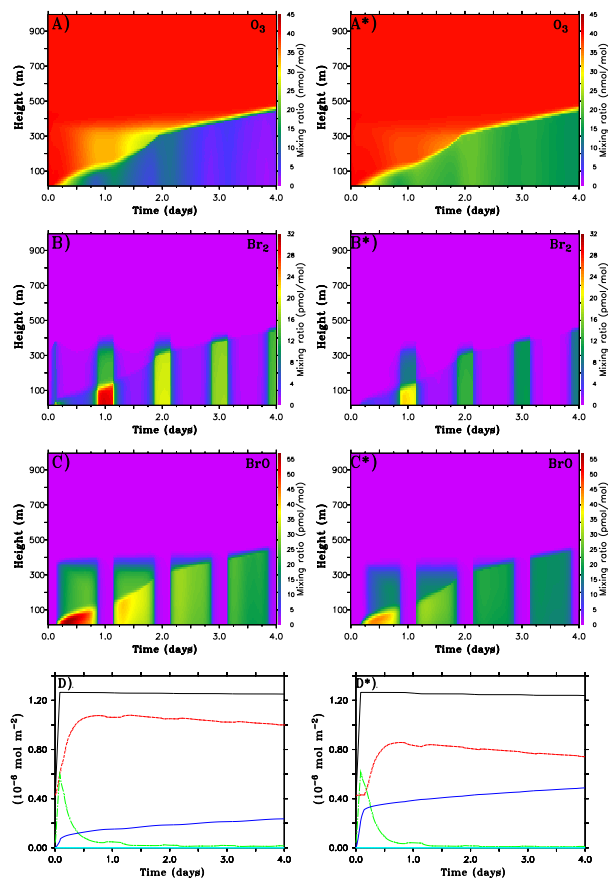
Fig. 7. Frost flowers at night (aerosols released the first day, 00:00 local time). Left (run 8): recycling of deposited bromine from the snow at night; right (run 9): no recycling at night. (A) \text{O}_3 , (B) \text{Br}_2 , (C) \text{BrO} , (D) same as in Fig. 2I.
