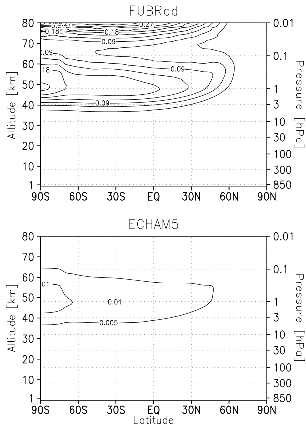
Fig. 2. Daily-mean, zonal-mean short-wave heating rate differences between solar maximum and minimum in K/day for 15 January. Top: FUB radiation scheme, contour interval 0.03 K/day. Bottom: Foucart and Bonnel radiation scheme, contour interval 0.005 K/day.
