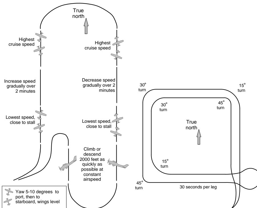
Fig. 4. Schematic diagram of the two airborne calibration procedures for the AIMMS sensor: (a) shows the flight plan for the aerodynamic calibration, whilst (b) shows the flight plan for the cross-axis calibration.
