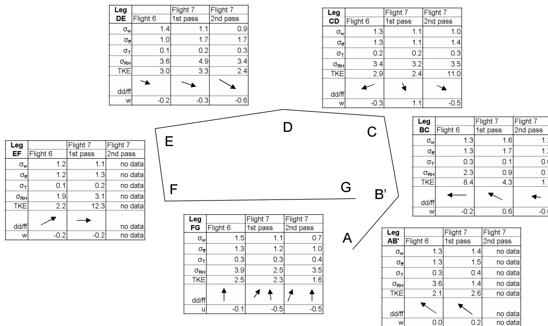
Fig. 8. Summary of standard deviations and means for Flights 6 and 7, to show relative variations as a function of flight path. \sigma_w , \sigma_{ff} and u are in \text{ms}^{-1} , \sigma_T is given in ^{\circ}\text{C} , \sigma_{RH} is given in %, and TKE is given in \text{m}^2 \text{s}^{-2} . dd/ff shows qualitatively the wind direction and strength.
