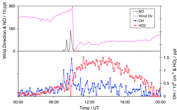
Fig. 3. HO x perturbation due to base pollution event of 30th January. Time series of OH (red circles, 10^6 molecule \text{cm}^{-3} ) and HO 2 (blue circles, ppt) (lower panel), together with NO (black line, ppt/10) and local wind direction (pink line) (upper panel).
