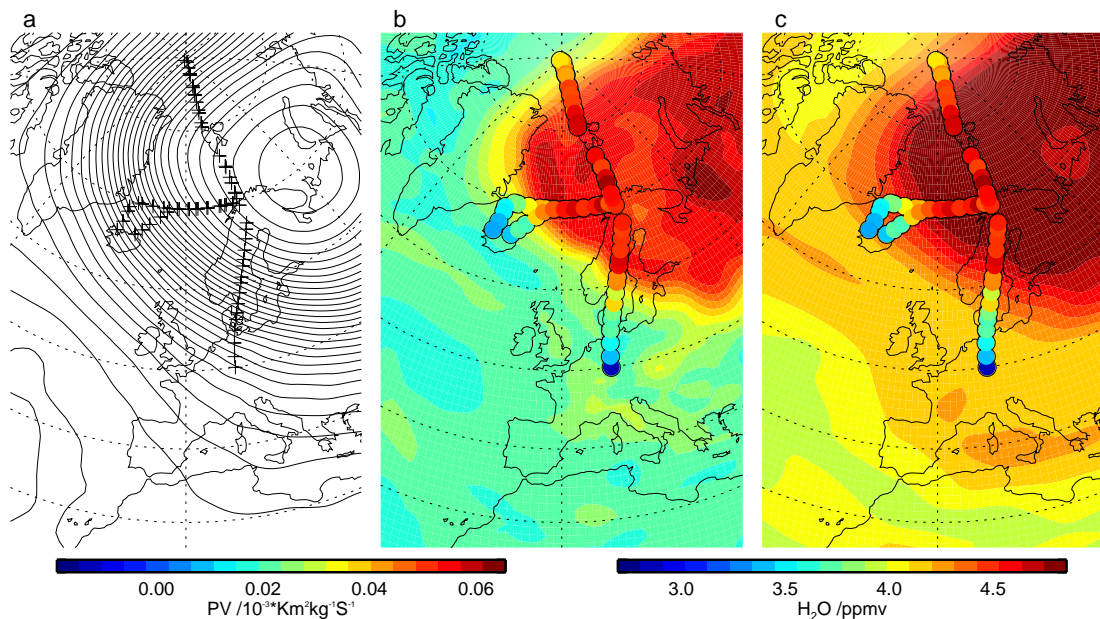
Fig. 10. ECMWF analyses for 12:00:00 UT 9 March 2000: (a) Geopotential height on a 50 hPa surface with AMSOS observation points; (b) Potential vorticity on the 475 K isentrope with AMSOS water vapour overlaid; (c) Water vapour mixing ratio on the 475 K isentrope with AMSOS water vapour overlaid. AMSOS observations from 8 March 2000 to 10 March 2000 are shown.
