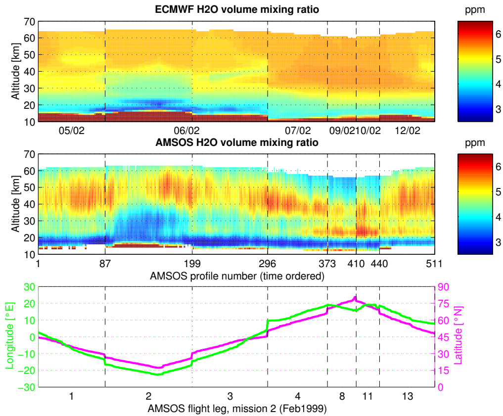
Figure 2: Overview of the complete AMSOS Mission 2 (February 5-12, 1999). The top plot shows ECMWF ERA-40 humidity profiles that correspond to the measured AMSOS profiles in the centre plot. The bottom plot shows the position of the measurements. The AMSOS profiles are ordered by time and numbered. Measurements from different days are separated by vertical dashed lines, while dotted lines separate different flight legs.
