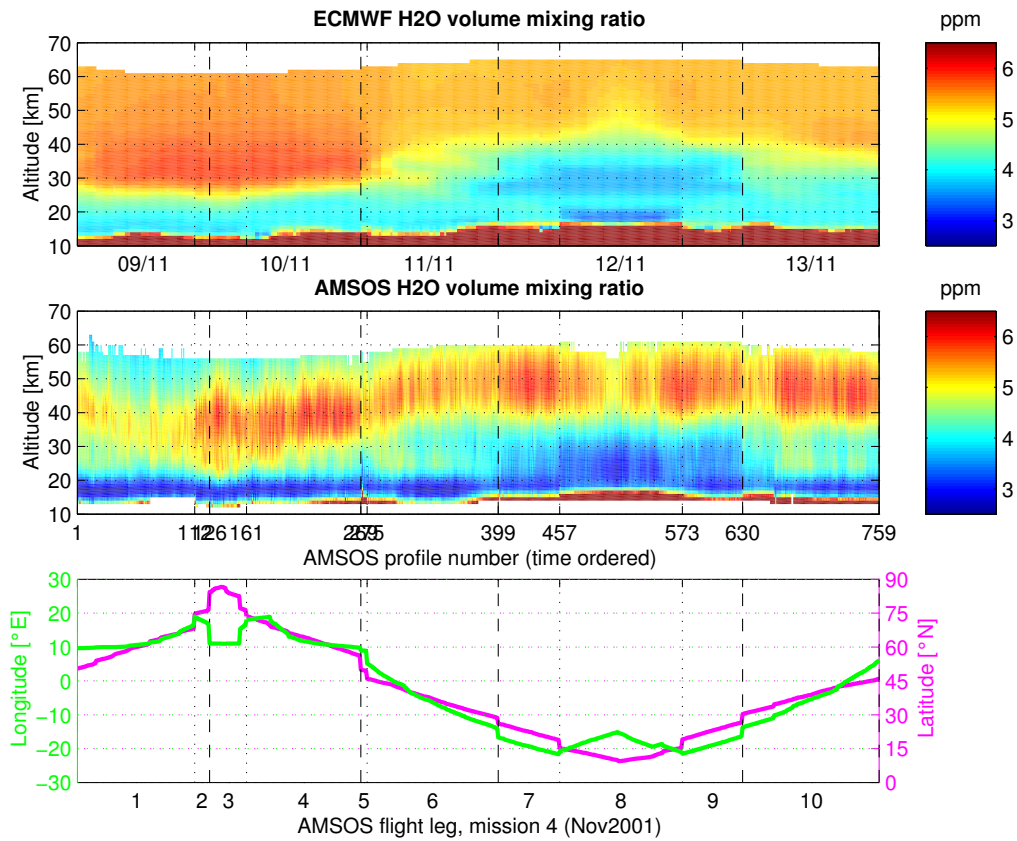
Figure 3: Overview of the complete AMSOS Mission 4 (November 9-13, 2001). The top plot shows ECMWF ERA-40 humidity profiles that correspond to the measured AMSOS profiles in the centre plot. The bottom plot shows the position of the measurements. The AMSOS profiles are ordered by time and numbered. Measurements from different days are separated by vertical dashed lines, while dotted lines separate different flight legs.
