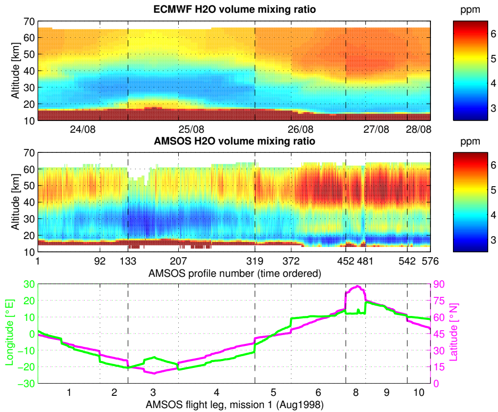
Figure 1: Overview of the complete AMSOS Mission 1 (August 24-28, 1998). The top plot shows ECMWF ERA-40 humidity profiles that correspond to the measured AMSOS profiles in the centre plot. The bottom plot shows the position of the measurements. The AMSOS profiles are ordered by time and numbered. Measurements from different days are separated by vertical dashed lines, while dotted lines separate different flight legs.
