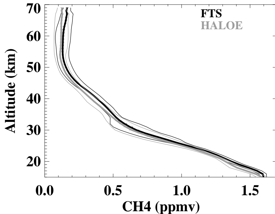
Fig. 5. Average profiles (thick lines) for all coincident measurements between ACE-FTS (black) and HALOE (gray). Thin lines are the profiles of standard deviations ( 1\sigma ) of the distributions, while error bars (often too small to be seen) represent the uncertainty in the mean ( \sigma divided by the square root of the number of comparisons).
