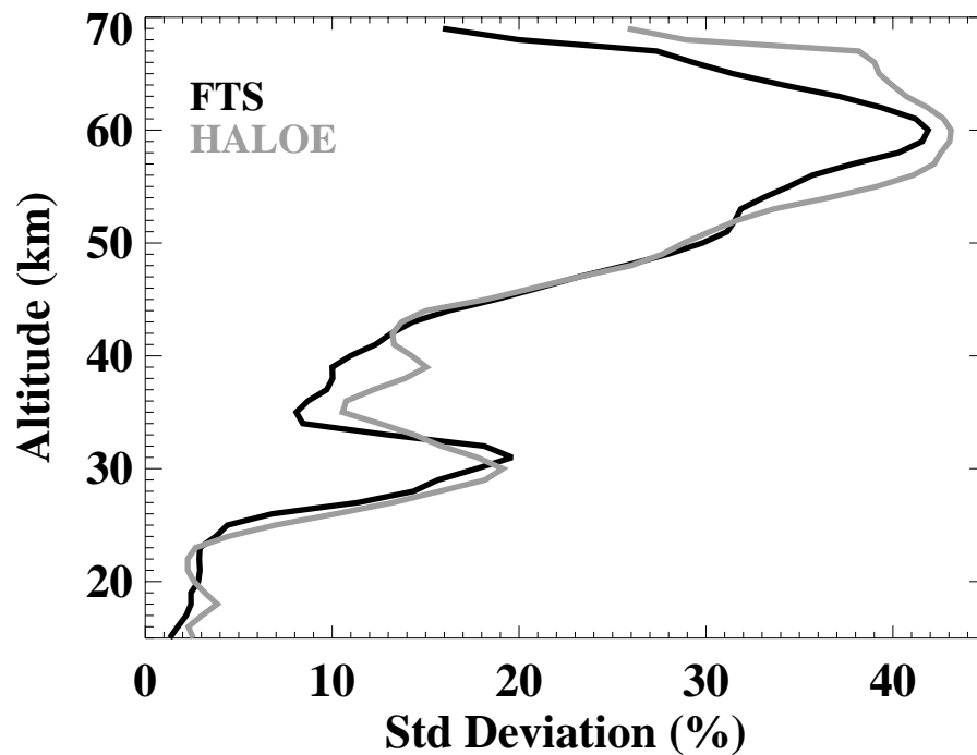
Fig. 6. Standard deviations of the distributions, 1\sigma , relative to the mean \text{CH}_4 mixing ratio at each altitude, for all coincident events, for ACE-FTS (black) and HALOE (gray).
