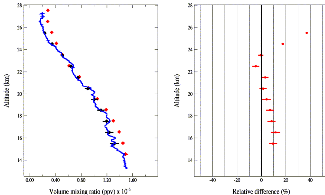
Fig. 1. Left plot: Methane vertical profiles obtained by ACE-FTS sr13151 (in red) and SPIRALE (in black and blue). The solid blue line corresponds to the SPIRALE measurements (very fine resolution) and the black diamonds correspond to the SPIRALE profile smoothed with a triangular convolution function (see Sect. 4). Error bars are reported on both profiles but, at several altitudes, they are so small that they are indiscernible. Right plot: The relative differences between the two profiles in percent, calculated as (200 \cdot (\text{ACE} - \text{SPIRALE}) / (\text{ACE} + \text{SPIRALE})) and the corresponding error bars.
