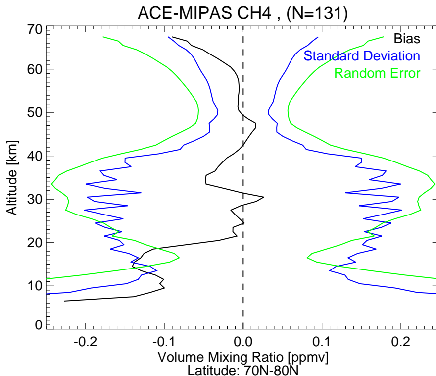
Fig. 3. VMR difference between ACE-FTS and MIPAS profiles of CH 4 : mean ACE-FTS minus MIPAS (black solid line) and associated 1 \sigma standard deviation (blue solid line) for a sample of 131 coincident profiles in the 70 to 80° N latitude band. The random error of the difference profile, combining the MIPAS and ACE-FTS random errors, is shown as the green solid line.
