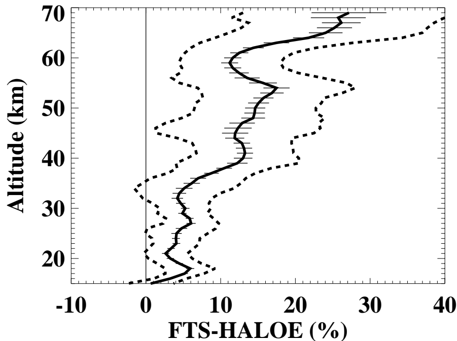
Fig. 7. Average percent differences (solid) between ACE-FTS and HALOE relative to the average of the two instruments, for all coincidences. Dashed lines represent the 1\sigma standard deviation of the distribution of differences while the error bars represent the uncertainty in the mean difference, i.e., \sigma/\sqrt{N} where N is the number of coincidences.
