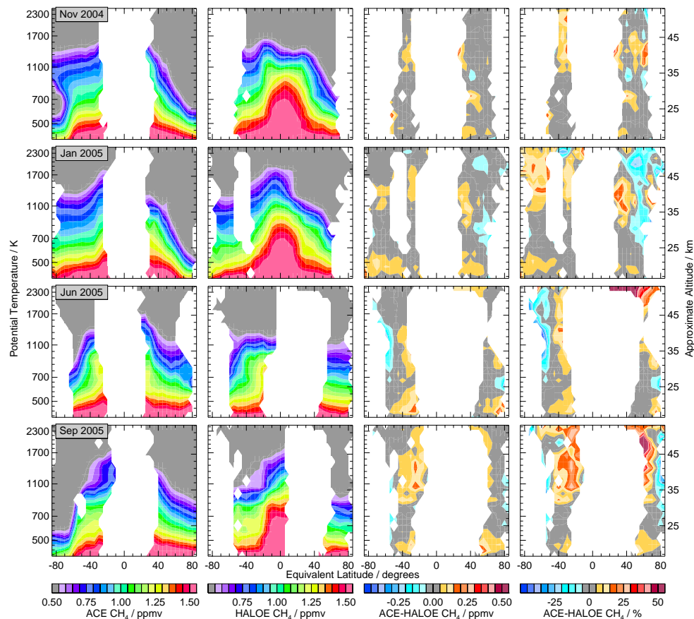
Fig. 9. Equivalent latitude/potential temperature (see text) sections of (left to right) ACE-FTS CH 4 , HALOE CH 4 , ACE-FTS–HALOE CH 4 in ppmv, and ACE-FTS–HALOE CH 4 in percent, for the months (from top to bottom) November 2004, January, June and September 2005. Vertical range is 400 K to 2500 K (15 to 50 km).
