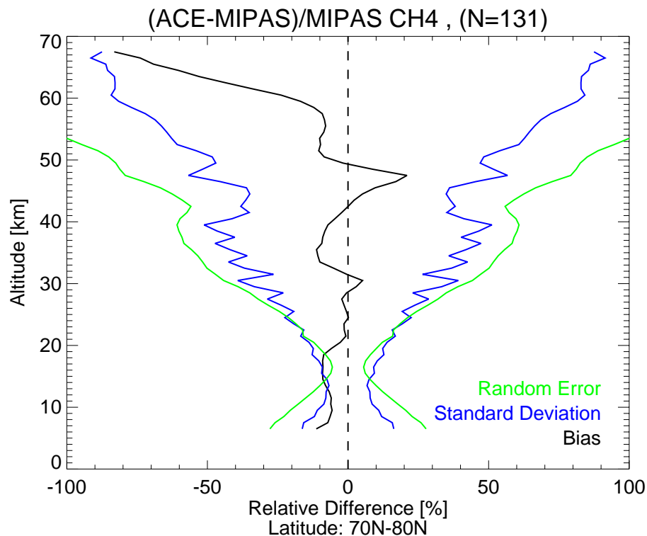
Fig. 4. Percentage relative difference between ACE-FTS and MIPAS profiles of CH 4 : mean ACE-FTS minus MIPAS divided by MIPAS (black solid line) and associated standard deviation (blue solid line) for a sample of 131 coincident profiles in the 70 to 80° N latitude and ACE-FTS errors, is shown as the green solid line.
