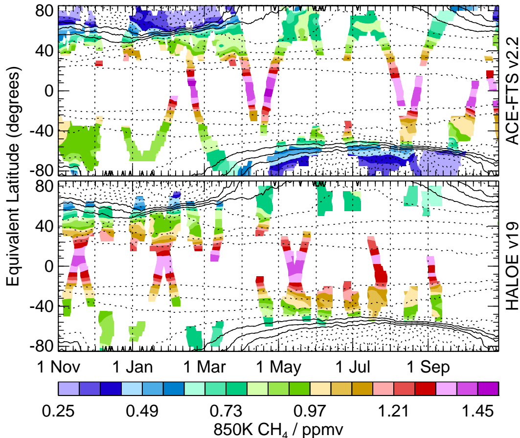
Fig. 8. ACE-FTS (top) and HALOE (bottom) CH 4 VMR (ppmv) on the 850 K potential temperature surface as a function of equivalent latitude and time (see text) for November 2004 through October 2005. Overlaid contours are scaled PV from the Met Office meteorological analyses, with solid line showing contours demarking the polar vortex edge region.
