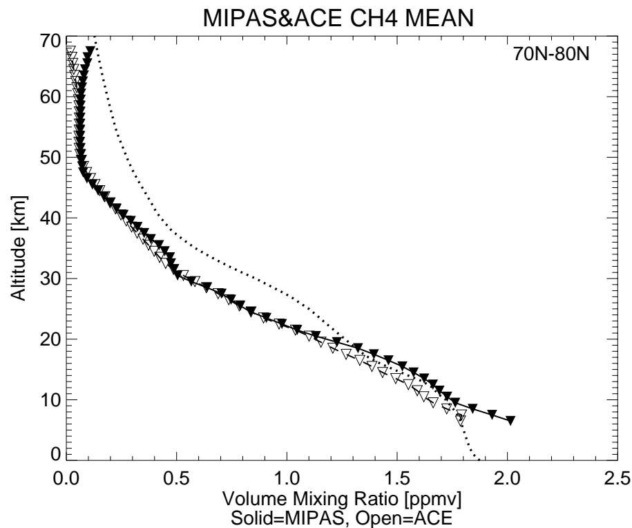
Fig. 2. Mean ACE-FTS (open triangles) and MIPAS (filled triangles) profiles of the 131 matching pairs in the 70–80° N latitude band, included in the comparison. The dotted line shows the MIPAS climatology (initial guess) for this latitude band.
