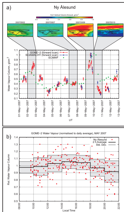
Fig. 7. Local time variations of water vapour over Ny Ålesund. (a) GOME-2, SCIAMACHY and ECMWF water vapour total columns 1–12 May 2007. For four selected days the spatial distribution of water vapour over the Spitsbergen area as seen by GOME-2 (daily gridded data) is shown. (b) Relative variation of GOME-2 water vapour columns over Ny Ålesund in May 2007 as function of local time. The black line shows averages of the Ny Ålesund data over two hours of local time, the grey lines and the underlying shaded area mark the corresponding standard deviations.
