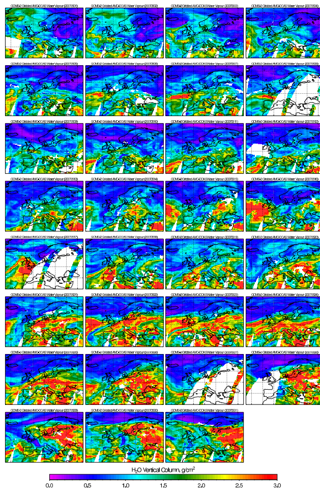
Fig. 6. GOME-2 daily water vapour data over Europe (gridded to 0.5^\circ \times 0.5^\circ in latitude/longitude) for May 2007.
