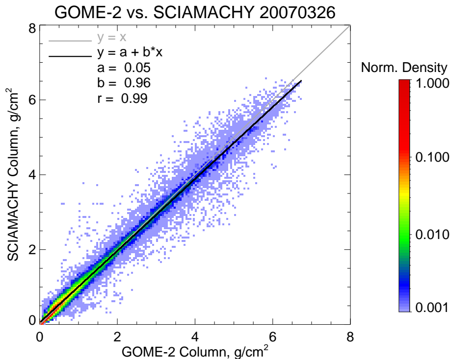
Fig. 2. Comparison of water vapour columns derived from preliminary GOME-2 spectral data from 26 March 2007 with corresponding SCIAMACHY results. The different colors give the density of collocated data points (normalised to the maximum value of 6561).
