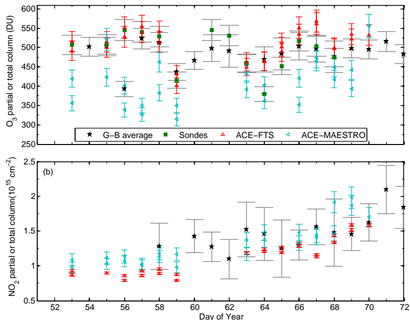
Fig. 16. Afternoon (a) ozone and (b) NO 2 vertical column densities from the campaign instruments, ozonesondes, and partial columns from ACE-FTS, and ACE-MAESTRO for 2004. For both species, the ground-based measurements have been averaged. Error bars for the ground-based VCDs are the sum in quadrature of the relevant percentage errors given in Table 2. For the ozonesondes, the errors are 5%. For ACE-FTS, the error bars represent only spectral fitting error, while for the ACE-MAESTRO the error bars are a combination of fitting error, errors in the cross-sections, and errors arising from unaccounted-for temperature effects in the cross-sections. For the satellite measurements, the partial columns are taken between 0 and 40 km for ozone and between 22 and 40 km for NO 2 .
