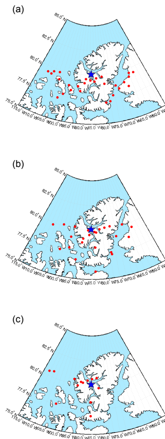
Fig. 2. Location of ACE occultations at 30 km altitude within 500 km of PEARL in February and March (a) 2004, (b) 2005, and (c) 2006. The blue star indicates the location of PEARL.
