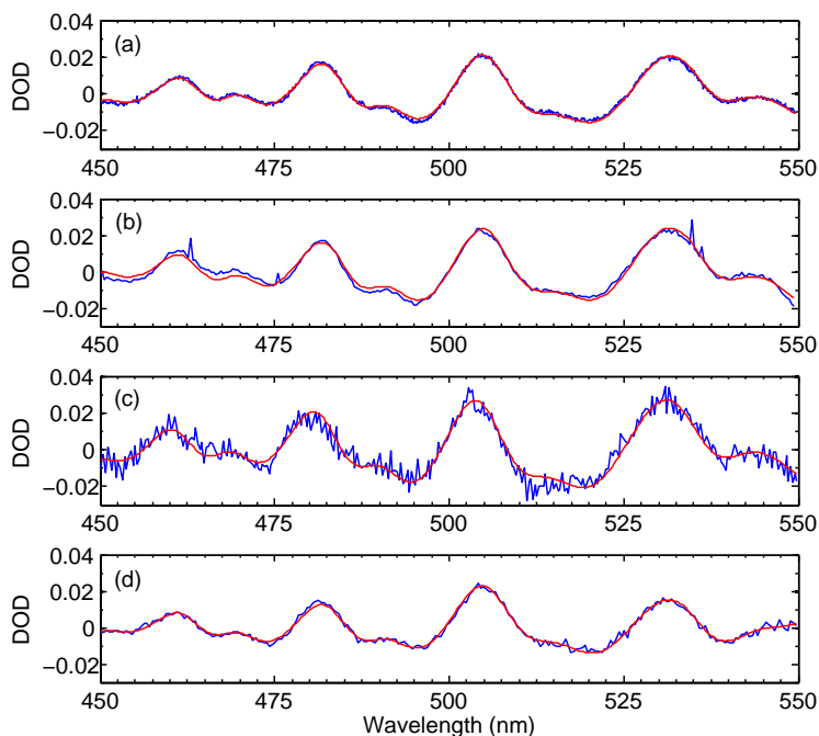
Fig. 3. Typical differential optical depth (DOD) ozone fits for (a) UT-GBS, (b) SAOZ, (c) MAE-STRO, and (d) SPS. All fits are for the afternoon of 4 March 2005 at a SZA of approximately 90°. In all plots, the blue line is the data, while the red line is the fit to the data.
