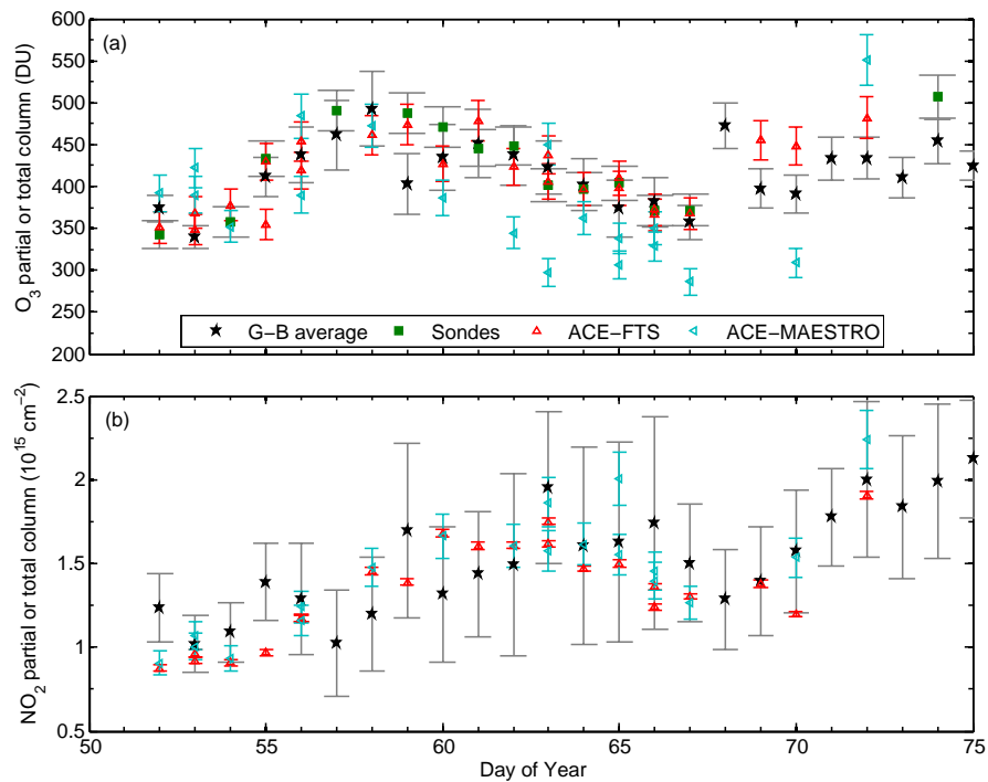
Fig. 18. Same as Fig. 16, but for 2005.
