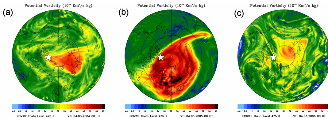
Fig. 1. ECMWF potential vorticity on the 475 K potential temperature layer for 4 March ( \sim 19 km, lower stratosphere) (a) 2004, (b) 2005, and (c) 2006. The location of PEARL is indicated by the white star.
