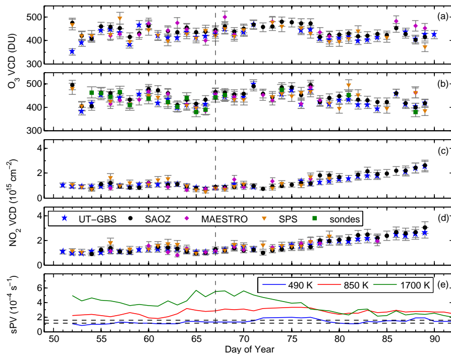
Fig. 19. Same as Fig. 15, but for 2006.
