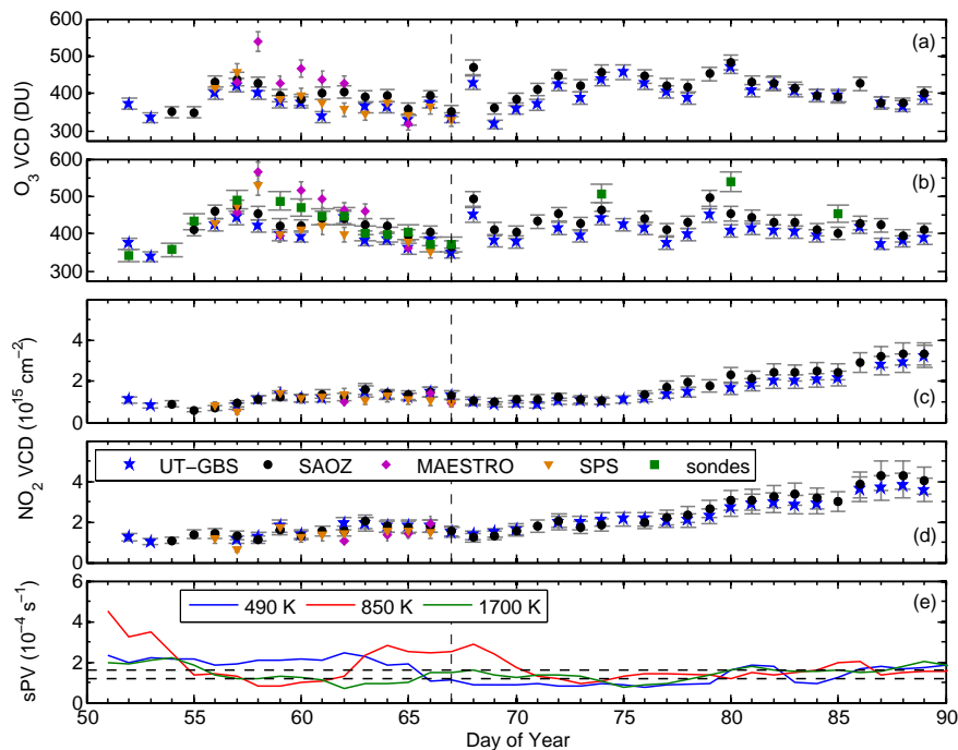
Fig. 17. Same as Fig. 15, but for 2005.
