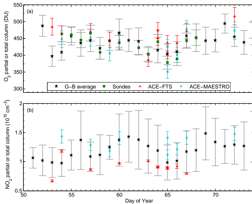
Fig. 20. Same as Fig. 16, but for 2006.
