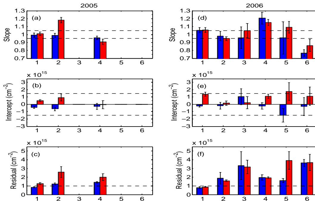
Fig. 11. NO 2 DSCD Type 1 results for (a–c) 2005, and (d–f) 2006. Dashed lines indicate the NDACC standards. In all figures, blue represents the morning comparisons, while red represents the afternoon. Error bars indicate the standard error. The numbers represent the comparisons between the different instruments: 1 – UT-GBS vs. SAOZ, 2 – UT-GBS vs. SPS, 3 – UT-GBS vs. MAESTRO, 4 – SPS vs. SAOZ, 5 – MAESTRO vs. SAOZ, 6 – MAESTRO vs. SPS.
