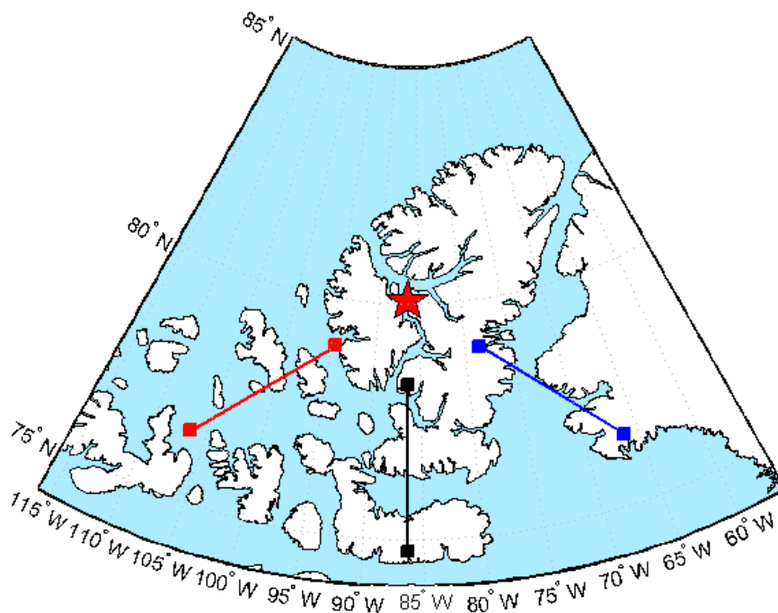
Fig. 14. Spatial extent of the DSCD measurements for 4 March 2005, calculated as the geometrical projection of the ozone maximum (18 km) for 86° (noon) and 91°. The blue and red lines indicate the geometrical projection of the ozone maximum at 91° for sunrise and sunset, respectively. The black line indicates the projection at 86°, which is the solar maximum on this day. The red star indicates the location of PEARL.
