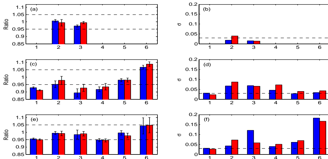
Fig. 9. Ozone Type 2 ratio results for (a) 2004, (c) 2005, and (e) 2006. The error bars represent the standard error. The standard deviation results for (b) 2004, (d) 2005, and (f) 2006. The dashed lines indicate the NDACC standards. Colours and numbers represent the same comparisons as Fig. 8.
