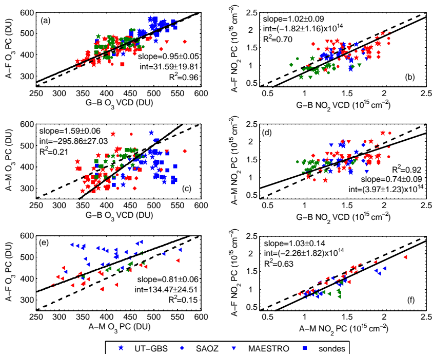
Fig. 21. Scatter plot of (a) ACE-FTS (A-F) ozone partial columns (PC) vs. ground-based (G-B) total columns and total columns from the ozonesondes. (b) Same as (a), but for NO 2 . (c–d) Same as (a–b), but for ACE-MAESTRO (A-M) partial columns. (e–f) Same as (a–b) but for ACE-FTS vs. ACE-MAESTRO. In all figures, the solid line shows the fitted relationship between the two data sets being compared. The slope, intercept, and R 2 for the comparisons are given on the figure. The dotted line shows the one-to-one line relationship for comparison. The blue points are for 2004, the red points are for 2005, and the green points are for 2006. The satellite partial columns are between 0 and 40 km for ozone and between 22 and 40 km for NO 2 .
