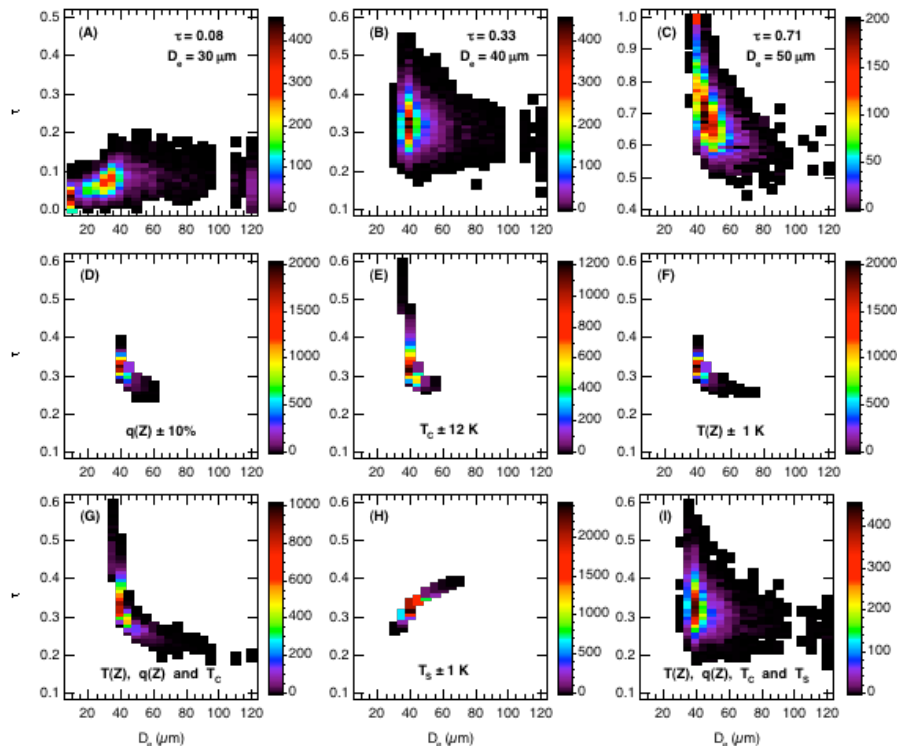
Fig. 4. Sensitivity of \tau and D_e to uncertainties in forward model inputs T(z), q(z), T_c, T_s, \varepsilon and \rho using normally-distributed 1\sigma errors of \pm 1 K, 10%, 12 K, 1 K, 0.01, and 0.01, respectively. Both T(z) and q(z) errors are uniformly applied to all levels in the vertical profile. (A) Probability density function of \tau and D_e retrievals after addition of normally-distributed errors in all forward model inputs for \tau=0.08 and D_e=30\ \mu\text{m} , for granule 134, footprint (scan line) number 40 (97), on 9 April 2003. (B) same as (A) except for \tau=0.33 and D_e=40\ \mu\text{m} , footprint (scan line) number 41 (84). (C) Same as (A) except for \tau=0.71 and D_e=50\ \mu\text{m} , footprint (scan line) number 73 (110). (D-I) Errors for single and multiple quantities for retrieval described in (B); see Figs. for quantities used in calculation.
