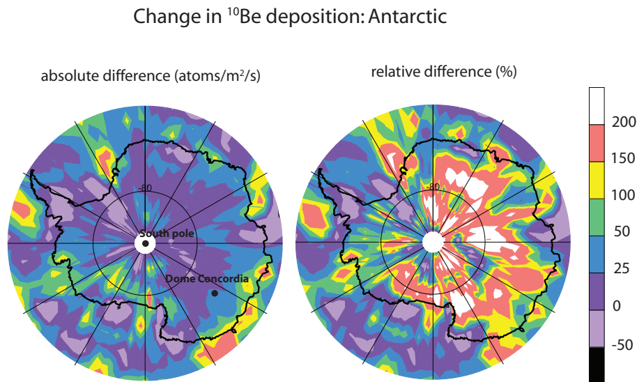
Fig. 9. The change of modeled ^{10}\text{Be} deposition between Maunder Minimum and Present Day in Antarctica in absolute (left) and relative (right) units.
