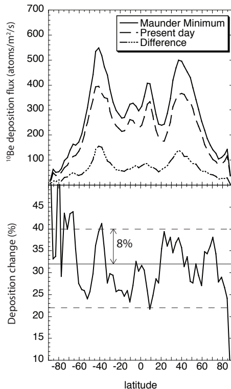
Fig. 7. 10 Be zonal mean deposition flux during Maunder Minimum and Present Day, and the change in absolute (atoms/m 2 /s, upper panel) and in relative (% , lower panel) units. The zonal mean deposition change is 32±8%. Polewards of 80° the relative difference is higher than this because the deposition fluxes are extremely low in these areas (see upper panel).
