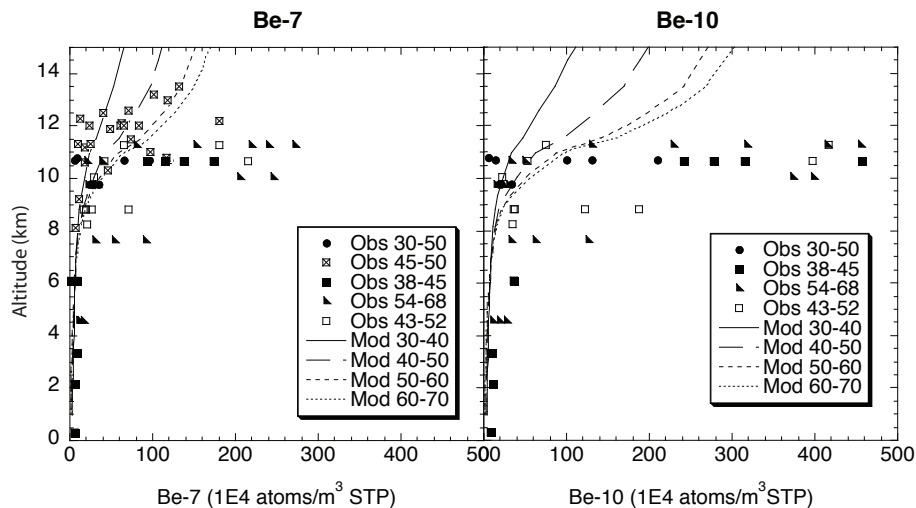
Fig. 6. Zonal mean modeled 7 Be (left) and 10 Be (right) concentrations in air against altitude for different latitude bands, compared with observations.
