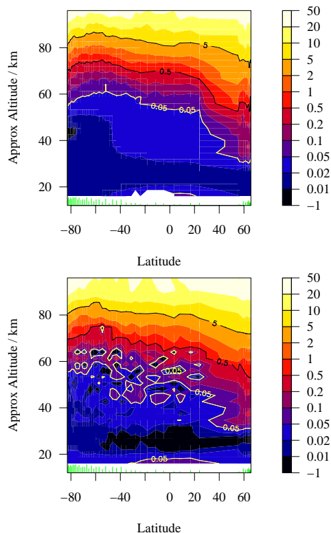
Fig. 19. ACE-FTS (top) and MLS (bottom) CO mixing ratios (ppmv) for 2 September–13 October 2006. For ACE-FTS the sunset latitude moves northwards during this period, so 2 September is at the left-hand side of the figure. The ticks near the bottom of the Figure show the mean ACE-FTS latitude for each of the days plotted; the length of each tick is proportional to the number of ACE-FTS sunset profiles on that day. For each ACE-FTS sunrise profile we took the 5 closest collocated MLS profiles and average together all such profiles for the day, in order to reduce noise. The data have been smoothed in latitude, with a smoothing length of 3^\circ .
