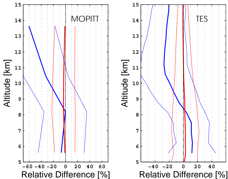
Fig. 15. Averaged percent difference ( \text{CO}_{\text{ACE}} - \text{CO}_{\text{nadir}} / \frac{1}{2} (\text{CO}_{\text{ACE}} + \text{CO}_{\text{nadir}}) ), calculated using all the coincident observations (thick blue line), along with the corresponding standard deviation (thin blue lines) for the years 2004, 2005 and 2006 (left, MOPITT) and 2005-2006 (right, TES). The red lines are for the ACE-FTS profiles which are smoothed by the nadir sounder averaging kernel functions. For both instruments, the number of coincident profiles ranges between \sim 850 (at 6 km) to \sim 3400 (above 12 km).
