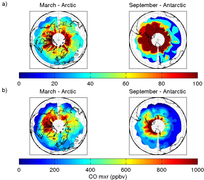
Fig. 6. ACE-FTS CO polar measurements in March and September 2005 at (a) 49.5 km and (b) at 59.5 km. The data are interpolated to a 6^\circ latitude \times 8^\circ longitude grid. We used polar projections over the Arctic (left plots) and the Antarctic (right plots) to illustrate the descent of CO-rich air masses in polar vortex situations.
