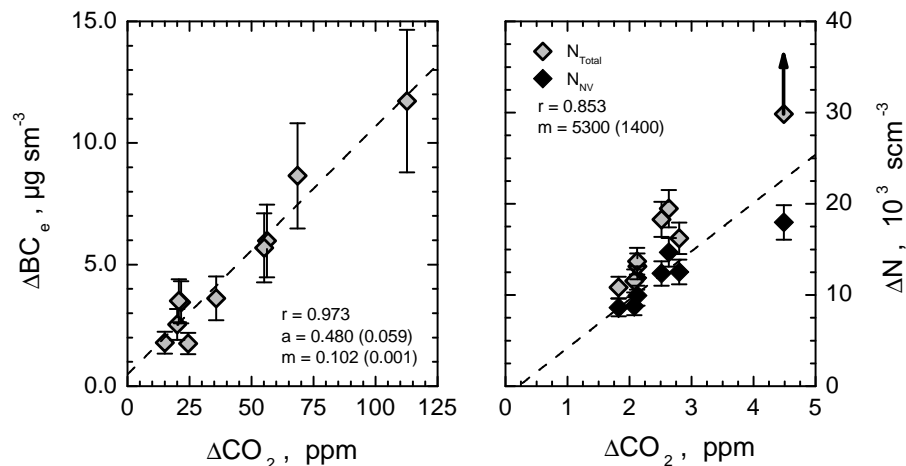
Fig. 10. Emission factors derived from the MAERSK vessel plume: BC_e from near field data with BC_e > \text{LOD} ; N_{NV} from far field data with N_{NV} below the CPC coincidence level of 20\,000 \text{ cm}^{-3} . Intercept a , slope m , and correlation coefficient r of the regression lines are added to the panels (uncertainties in parentheses).
