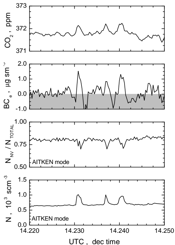
Fig. 4. Aerosol properties in aged ship plumes: CO 2 , equivalent BC e mass concentration (grey shaded area indicates unphysical negative BC e values < limit of detection), non-volatile fraction of the Aitken mode aerosol, and number concentration of the Aitken mode during three distinct plume encounters.
