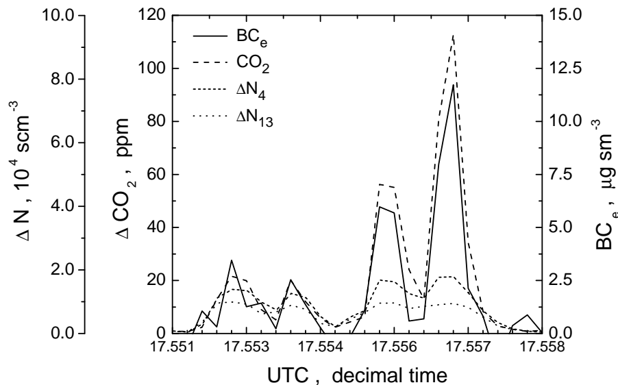
Fig. 8. Raw data of the closest plume encounter: equivalent black carbon from aerosol light absorption measurement ( BC_e ; solid line), excess CO_2 ( \Delta CO_2 ; dashed line), and excess number densities of particles with D > 4 \text{ nm} ( \Delta N_4 ; short dotted line) and D > 13 \text{ nm} ( \Delta N_{13} ; dotted line).
