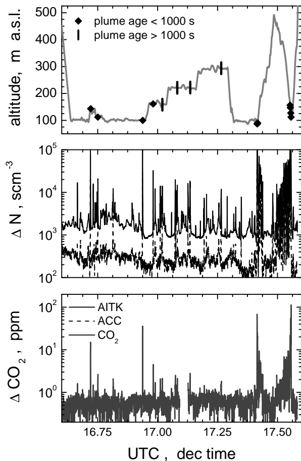
Fig. 7. Time series of flight altitude in m above sea level (a.s.l.): excess number concentration \Delta N for Aitken (AITK) and accumulation (ACC) mode particles, and excess CO_2 ( \Delta CO_2 ) during the Single Plume Study.
