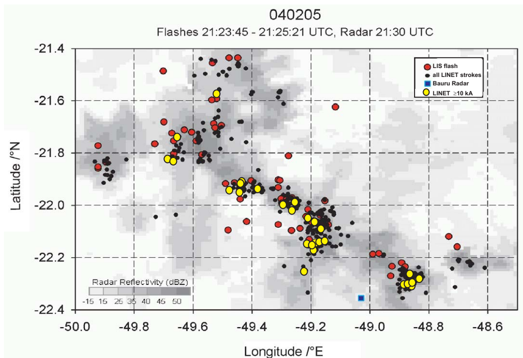
Fig. 12. Vertical maximum of the radar reflectivity (max CAPPI frame, unit dBZ) on 4 February 2005 at 21:30 UTC measured by the Bauru (22.4° S, 49.0° W) and Presidente Prudente (22.1° S, 51.4° W) radars. Superimposed are the horizontal distributions of LIS flashes (in red) and LINET strokes (black and yellow) for the time period 21:23:45 UTC–21:25:21 UTC
