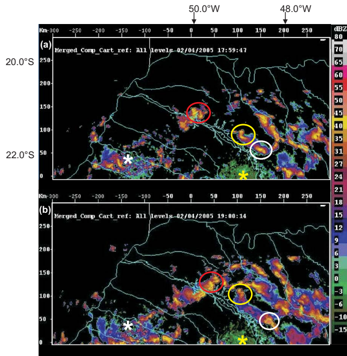
Fig. 9. Vertical maximum of the radar reflectivity (max CAPPI frame, unit dBZ). Composite from the Bauru (22.4° S, 49.0° W) and Presidente Prudente (22.1° S, 51.4° W) radars for the 4 February 2005 thunderstorms at (a) 17:59:47 UTC, and (b) 19:00:14 UTC. Selected thunderstorms are marked (tropical: yellow circle anvil 1a, white circle anvil 5a and red circle anvil 2b). The change in location of each of these circles between (a) and (b) indicates the storm motion, which can be compared with the storm motion indicated by arrows in Fig. 4a. The Bauru and Presidente Prudente radar sites are indicated with a yellow and white *, respectively. The left and upper axes give the distance in km, and the latitude and longitude are indicated in (a) . (TITAN Software, installed at IPMet in collaboration with NCAR.)
