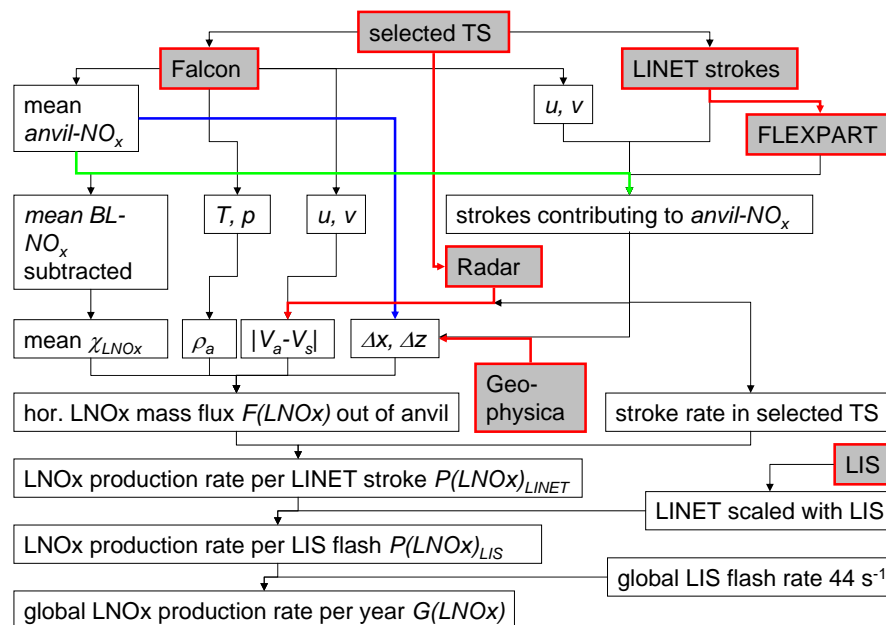
Fig. 3. Flow chart showing the introduced method to estimate the annual global LNOx production rate from TROCCINOX field measurements (Falcon, Geophysics, LINET, Radar) combined with LIS data and model simulations (FLEXPART) of the selected thunderstorms (TS) all indicated with grey background. Different line colours are used to avoid misunderstanding of the flow direction at line intersections.
