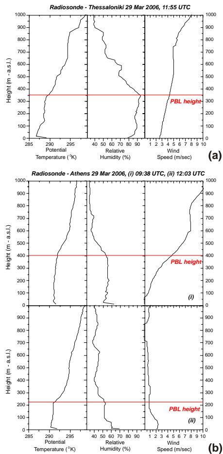
Fig. 3. Potential Temperature, relative humidity and wind speed measured with radiosondes on 29 March 2006, at 11:55 UTC for Thessaloniki (a) and at 09:38 UTC (b-top panel-(i)) and 12:03 UTC for Athens (b-bottom panel-(ii)).
