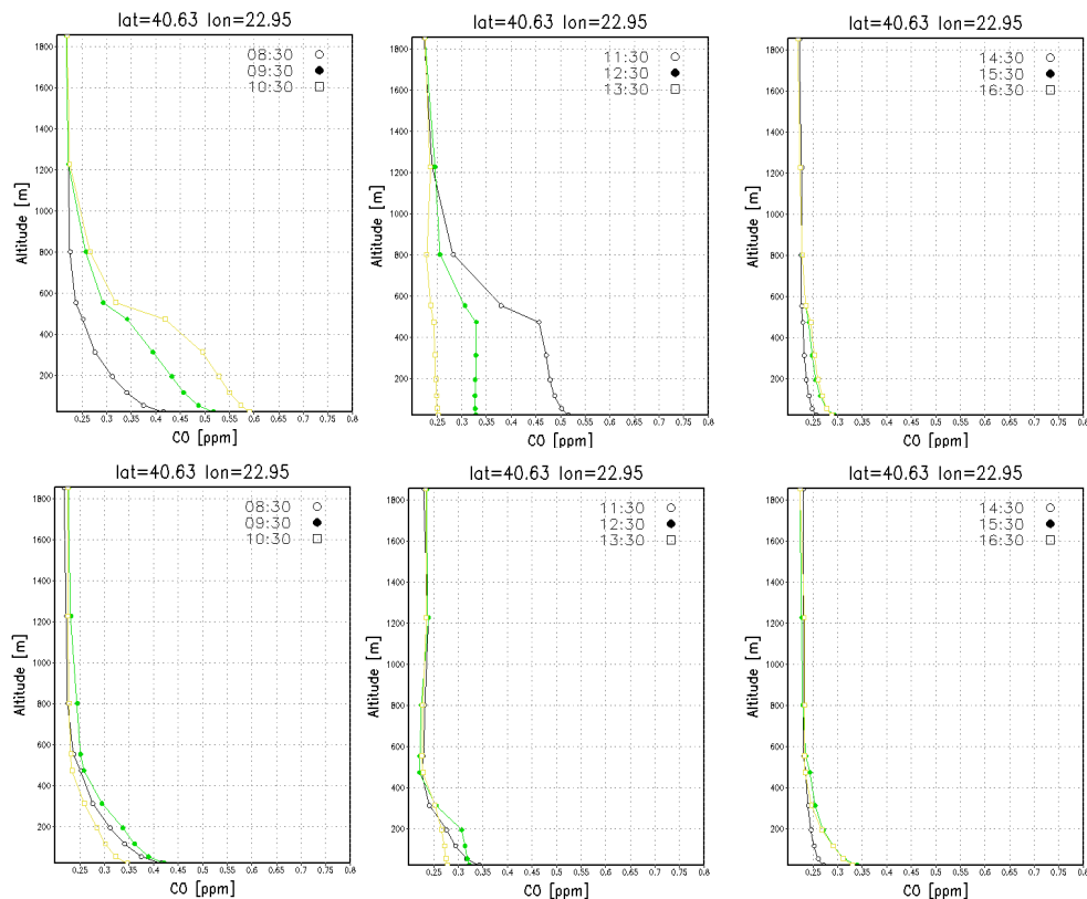
Fig. 6. Temporal evolution of modeled CO vertical profiles for the eclipse (bottom panel) and non-eclipse case (top panel) for the site in Thessaloniki.
