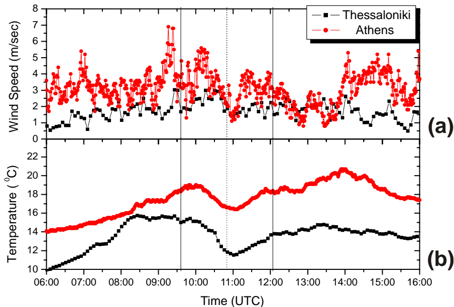
Fig. 2. Surface wind speed (a) and temperature (b) timeseries for Thessaloniki (black dotted line) and Athens (red dotted line). Vertical lines correspond to the first contact-maximum-last contact of the eclipse.
