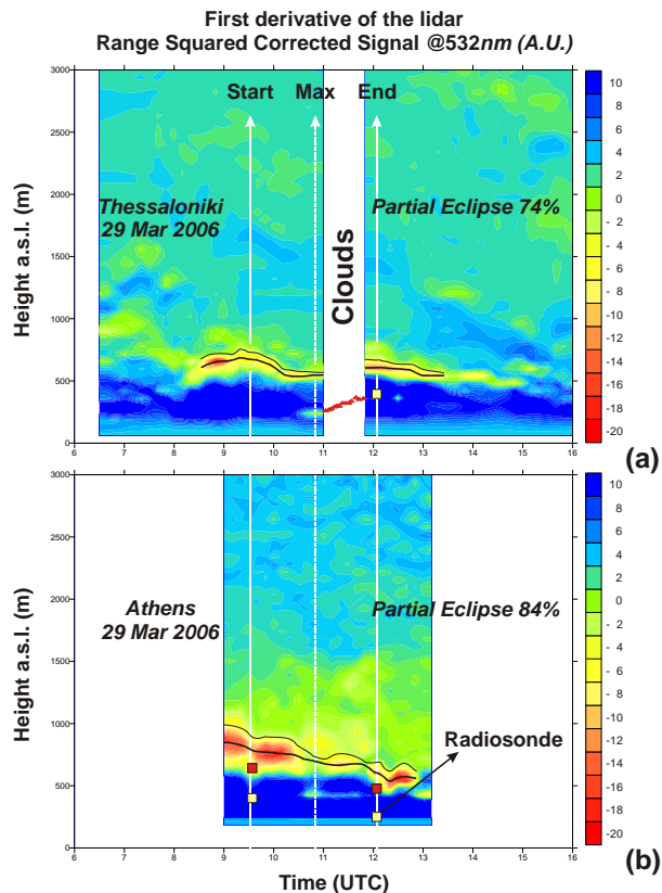
Fig. 1. Time-height cross section of the first derivative of the range squared corrected lidar signal at 532 nm (in arbitrary units – A.U.) at Thessaloniki (a) and Athens (b) measured on 29 March 2006. The upper and lower limits of the entrainment zone are demonstrated with the thin and bold solid line, respectively, the latter representing the evolution of the ML height. Red triangles correspond to lidar retrieved cloud base height. Squares represent PBL heights calculated from radiosonde meteorological profiles.
