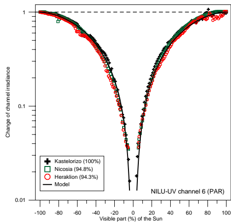
Fig. 3. Change of solar irradiance for NILU-UV channels 5 (380 nm, upper panel) and 6 (PAR, lower panel) for sites 6–8. For each site the maximum eclipse percentage is provided.
