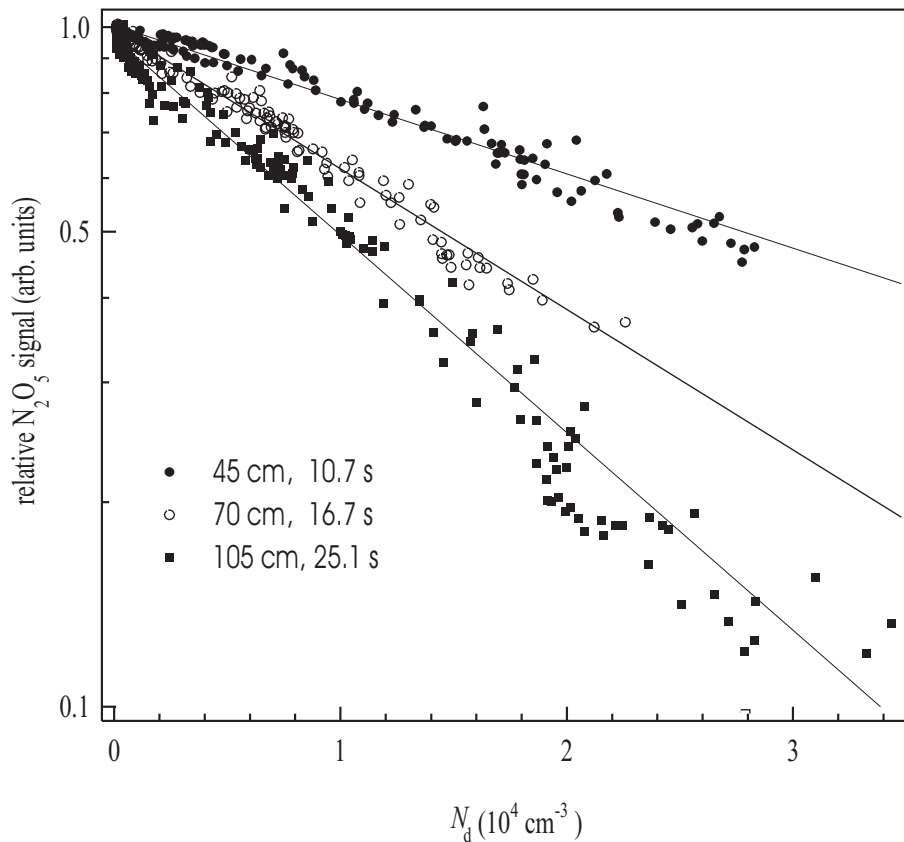
Fig. 6. Dependence of the \text{N}_2\text{O}_5 signal on the dust concentration at three different injector positions. The slope of the exponential fits (solid lines) is equal to 1/4\gamma\bar{c}A_d t . The statistical errors on each single data points are within the symbol size.
