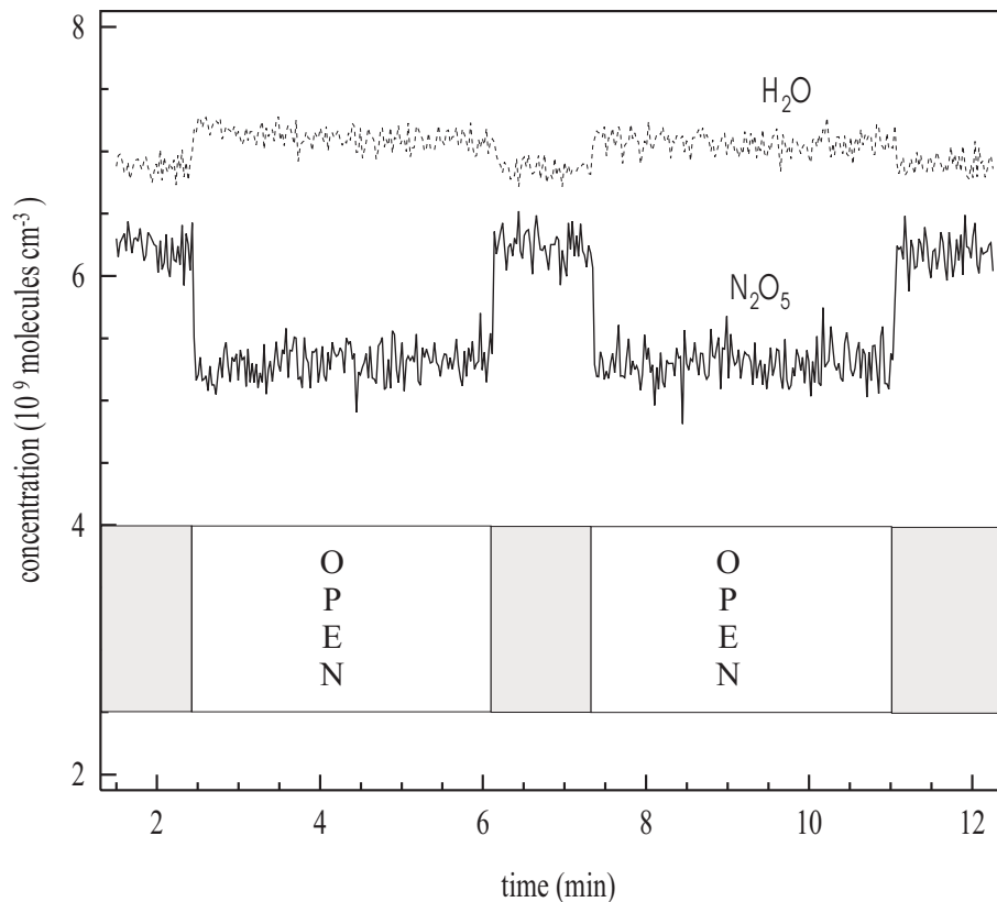
Fig. 10. Knudsen reactor data for the uptake of \text{N}_2\text{O}_5 to 21.6 mg of SDCV. The release of \text{H}_2\text{O} from the dust sample upon opening the lid to the sample chamber (multiplied by a factor of 3 for clarity) and the times of opening and closure of the sample chamber (open) are also indicated.
