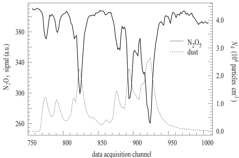
Fig. 3. Response of \text{N}_2\text{O}_5 (solid line, left y-axis) to the addition of a mineral dust pulse (dotted line, right y-axis) to the flow reactor. The time between acquisition of neighbouring data points was \approx 1.7 s.
