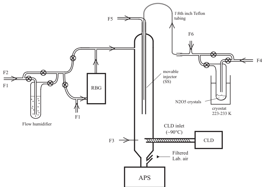
Fig. 1. Aerosol flow tube set-up. RGB = rotating brush generator, CLD = chemiluminescence NO detector, APS = aerodynamic particle sizer spectrometer, SS = stainless steel. The total flow ( \text{N}_2 unless otherwise stated) was 3000 sccm with (typically) F4 + F6 = 500 sccm; F5 = 10 sccm; F3 = 20 sccm (0.001% NO in \text{N}_2 ); F1 + F2 = 2500 sccm (with a variable proportion through the humidifier to obtain RH of 0, 29 and 58%).
