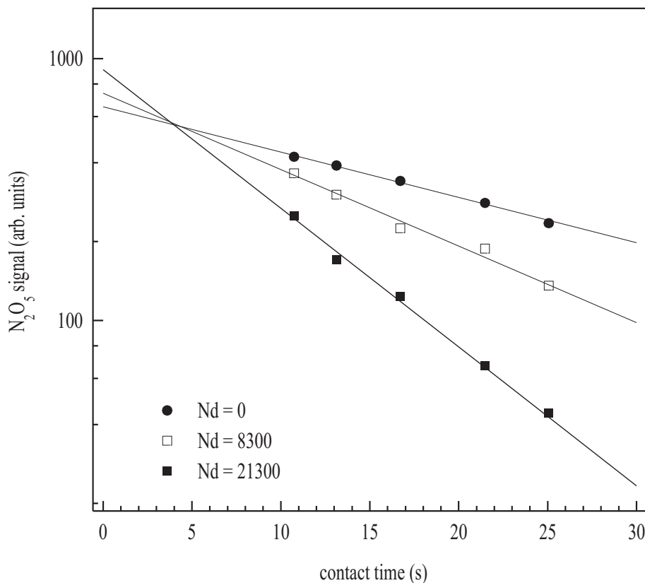
Fig. 4. N_2O_5 signal versus contact time for three dust concentrations. N_d is the number of dust particles per cm^3 . The decay of N_2O_5 in the absence of aerosol ( N_d=0 ) is due to loss to the reactor wall. Experimentally determined pseudo first-order loss coefficients were: (4.0\pm 0.3)\times 10^{-2} , (6.7\pm 1.0)\times 10^{-2} and (12.2\pm 1.6)\times 10^{-2} for N_d=0 , 8300 and 21 300 cm^{-3} , respectively. The errors quoted are 2\sigma statistical.
