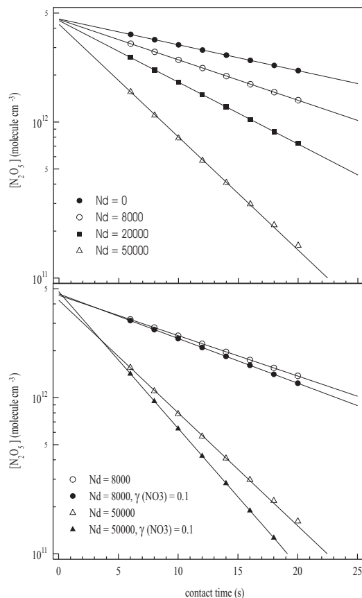
Fig. 8. Simulated \text{N}_2\text{O}_5 profiles, for details see text. Upper panel: Effect of \text{N}_2\text{O}_5 + \text{NO}_2 + \text{NO}_3 equilibrium on the uptake kinetics of \text{N}_2\text{O}_5 . N_d is the dust particle number density ( \text{cm}^{-3} ). Lower panel: Effect of \text{NO}_3 uptake to dust (assuming \gamma(\text{NO}_3) = 0.1 ) on the \text{N}_2\text{O}_5 profiles. The open symbols are simulations without loss of \text{NO}_3 , the closed symbols represent the effect of \gamma \text{NO}_3 = 0.1 with two different dust concentrations.
