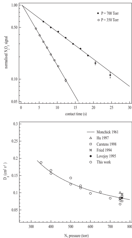
Fig. 9. Upper panel: Exponential decay profiles of \text{N}_2\text{O}_5 due to loss at the reactor wall at experimental pressures of 350 and 700 Torr. The error bars are derived from propagation of errors in the NO difference signal. Lower Panel: Pressure dependent diffusion coefficients from the present study compared to experimental results (Carstens, 1998) and theoretical calculations: Hu 1997 = Hu and Abbatt (1997), Fried 1994 = Fried et al. (1994), Monchick 1961 = Monchick and Mason (1961), Lovejoy 1995 = Lovejoy and Hanson (1995). For the present data set, statistical errors (from e.g. data sets as shown in the upper panel) were smaller than the symbol size.
