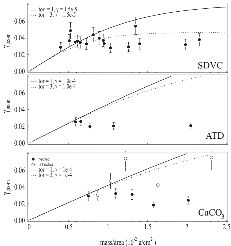
Fig. 11. Uptake coefficients ( \gamma_{\text{geom}} ) for interaction of \text{N}_2\text{O}_5 with Saharan dust (SDCV), Arizona test dust (ATD) and calcite. For SDCV and ATD all samples were dried by heating prior to the experiment. For \text{CaCO}_3 the solid circles indicate uptake coefficients obtained using heated samples. The open circles are data points from unheated samples. The smooth lines represent calculations using a pore diffusion model to take into account the interstitial surface area of the sample. The full line was calculated with a tortuosity factor ( \text{tor} ) of 1, the dashed line with a value of 3 (see text for details).
