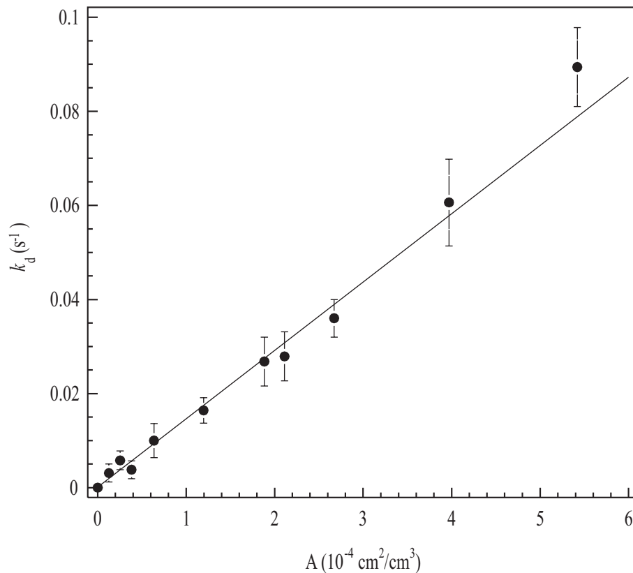
Fig. 5. Dependence of the pseudo first-order decay constant ( k_d ) of \text{N}_2\text{O}_5 on the dust surface area. The error bars are 1 \sigma as obtained from unweighted fitting to data sets similar to those shown in Fig. 4.
