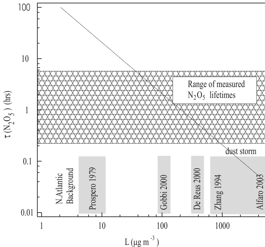
Fig. 13. \text{N}_2\text{O}_5 lifetime versus dust loading. The smooth line is the lifetime with respect to uptake to mineral aerosol based on the uptake coefficient measured in this work. Illustrative measurements of dust loadings and \text{N}_2\text{O}_5 lifetimes are also given. References are: Prospero 1979 = (Prospero, 1979), Gobbi 2000 = (Gobbi et al., 2000), De Reus 2000 = (Reus et al., 2000), Zhang 1994 = (Zhang et al., 1994), Alfaro 2003 = (Alfaro et al., 2003). The literature source of the \text{N}_2\text{O}_5 lifetimes is given in the text.
