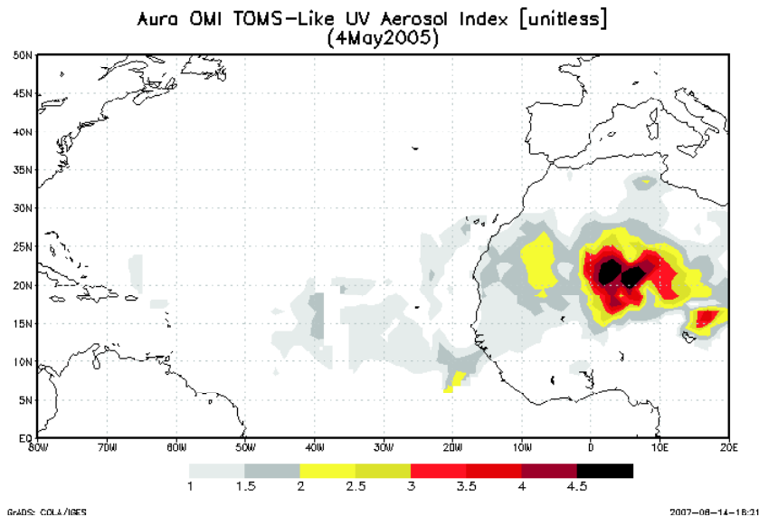
Fig. 2. OMI Aerosol Index for 4 May 2005.
