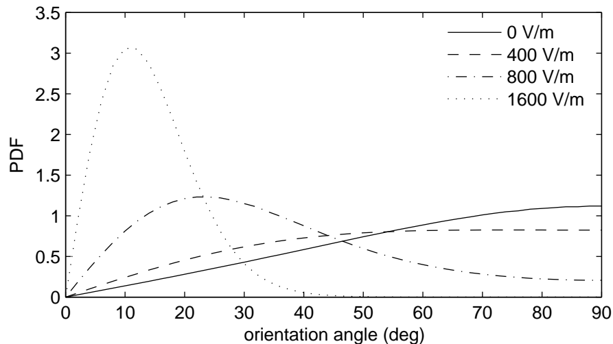
Fig. 8. Normalized probability distribution function of orientation angle of prolate ellipsoids with a long axis of 10\ \mu\text{m} , aspect ratio of 1.5 and density is 2.6\ \text{g/cm}^3 , falling under gravity and subjected to a vertical electric field (strength shown in the legend).
