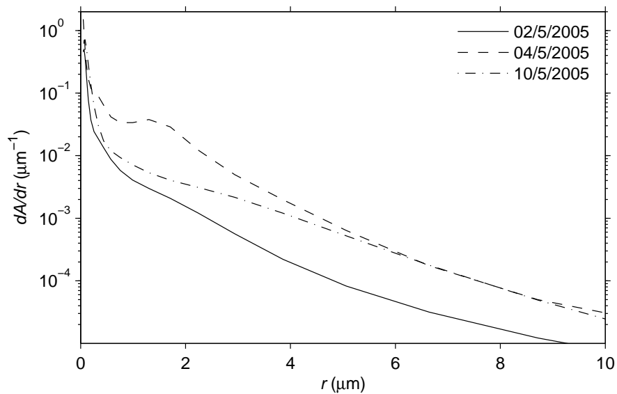
Fig. 5. As Fig. 4 but the columnar size distributions are in terms of the projected area for equal width size bins ( dA/dr ).
