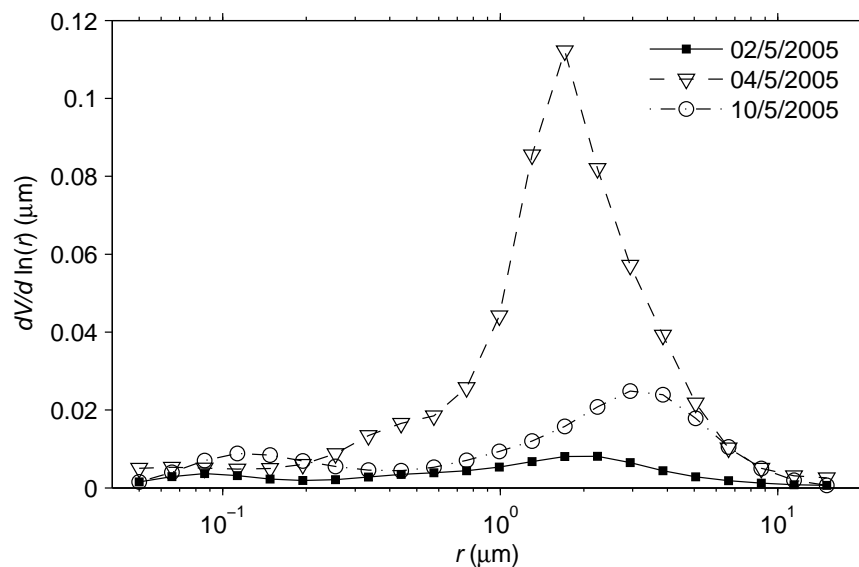
Fig. 4. Example columnar aerosol size distributions retrieved from the sun photometer at Santa Cruz, just before, during and just after the dust episode. The distributions are in terms of particle volume, i.e. dV/d \ln(r) , where r is the radius of the volume-equivalent sphere.
