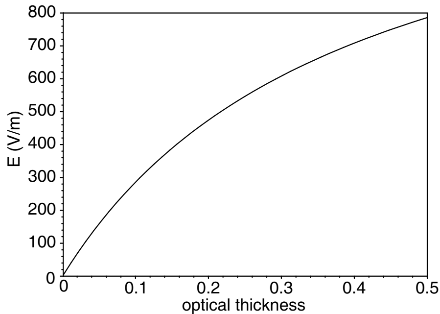
Fig. 7. Electric field gradient as a function of aerosol optical depth calculated from Eq. (12) for an aerosol layer 400 m thick.
