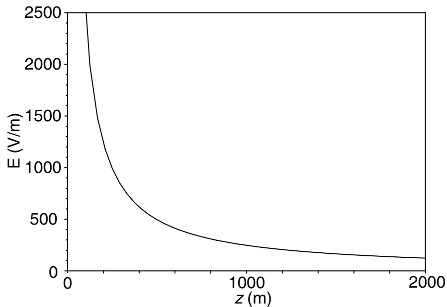
Fig. 6. Electric field gradient as a function of aerosol layer thickness for optical depth of 0.31, calculated from Eq. (12) with the topographic enhancement factor of two.
