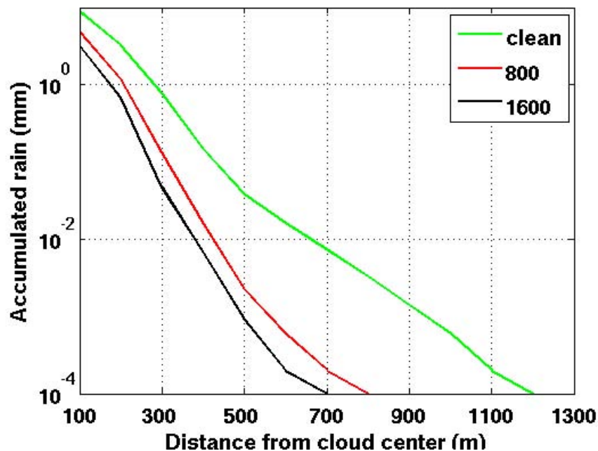
Fig. 13. Accumulated rain (mm) as a function of the distance from cloud center (100 m resolution) for cloud 1 (clean) – green columns, cloud 2 ( 800 \text{ cm}^{-3} ) – red columns, cloud 3 ( 1600 \text{ cm}^{-3} ) – black columns.
