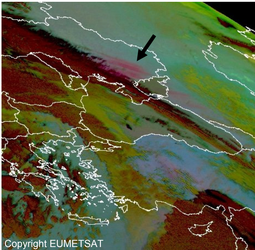
Fig. 4. Dust source activation on 23 March 11:00 UTC over the southern Ukraine (arrow). The image shows MSG dust index images, based on BTD using the 8.7\ \mu\text{m} , 10.8\ \mu\text{m} and 12.0\ \mu\text{m} wavelength bands of the SEVIRI instrument (cf. Sect. 2.1). Magenta colour indicates dust, green colour low-level clouds, brown colour thick mid-level clouds and dark red colour thick high-level clouds. Copyright (2007) EUMETSAT, Darmstadt, Germany.
