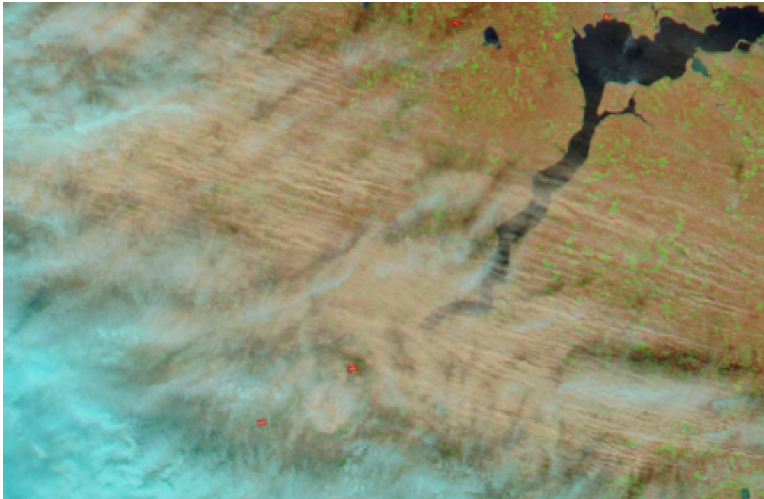
Fig. 5. MODIS-Aqua composite image of Southern Ukraine on 23 March 2007, 10:50 UTC reveals the large scale emission of agricultural dust. The reservoir lake of Kakhovskaya on the Dnieper River can be seen in dark blue, ice clouds in light blue. Red boxes indicates thermal anomalies, caused in most cases by fire or even flares from a gas well. The dimensions of the area shown is 210×146 km.
