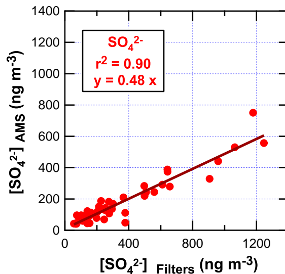
Fig. 2. Comparison of the SO 4 2- (PM 1 ) concentrations measured with Q-AMS and on filters over 24 h averaging intervals in March 2004.
