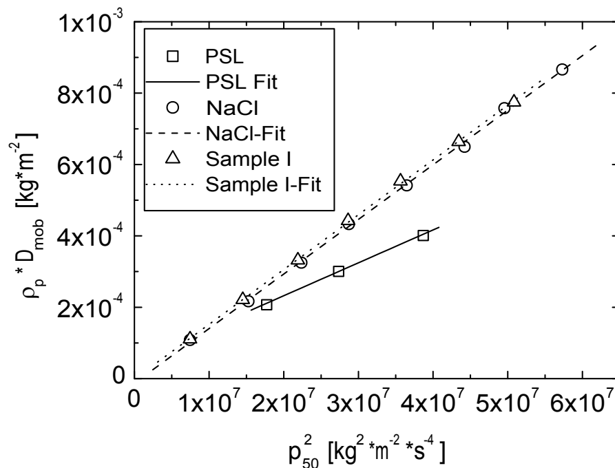
Fig. A2. The product \rho_p D_{mob} is plotted against p_{50}^2 for the PSL, NaCl and sea-salt (sample I) particles, to determine the shape factor of the different sea-salt particles.
