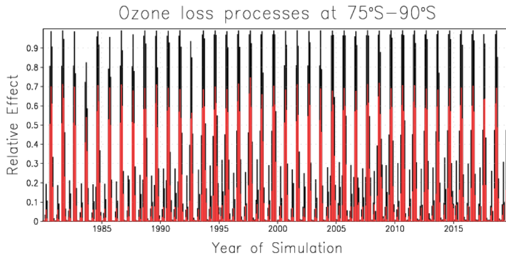
Fig. 5. Proportions of the total ozone loss chemistry due to the two main catalytic ozone loss cycles during the 40-year FinROSE integration. The red portions of the bars show the effect of ClO x processing, and the black portions show the effect of combined BrO x -ClO x chemistry, respectively. The values are averaged within the 75° S latitude, and between 146 and 31 hPa.
