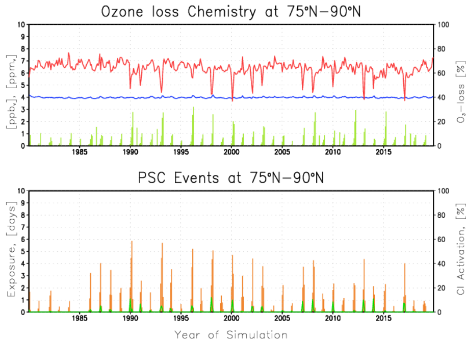
Fig. 6. Simulated monthly average time-series for 1980–2019 of the main constituents affecting ozone within 75^\circ\text{N} , and between 146 and 31 hPa. In the upper frame the total nitrogen is shown by the red line (in \text{ppb}_v ), water vapour (in \text{ppm}_v ) by the blue line, and the relative difference between the passive ozone tracer and regular model ozone by the green bars. In the lower frame the chlorine activation is shown by the orange bars, the PSC type-I tracer is given by the green line and the PSC type-II tracer by the black line.
