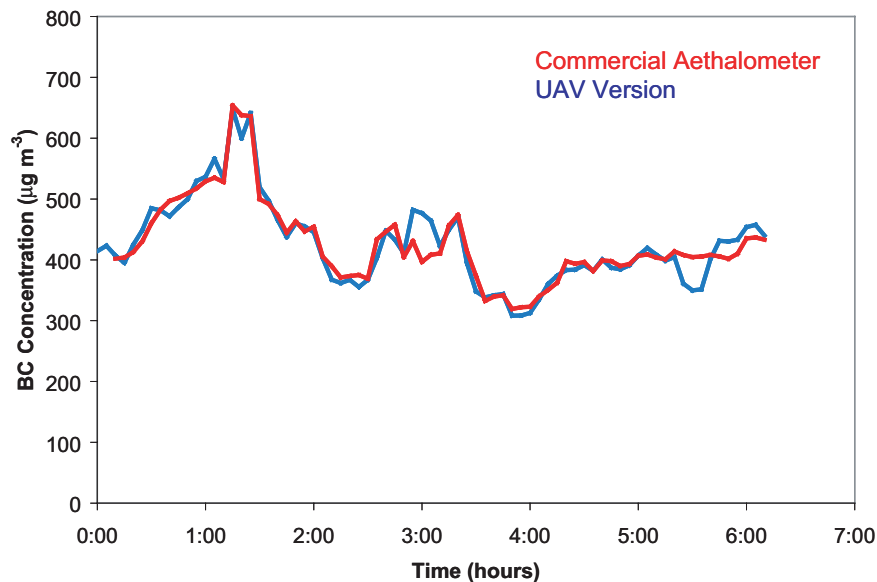
Fig. 6. Laboratory comparison at 880 nm of the AUAV absorption photometer with an original Magee Scientific AE-31 aethalometer.
