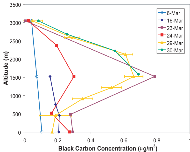
Fig. 13. Black carbon concentration altitude profiles during MAC experiment (March 2006). Error bars are only shown for a single flight to keep the plot legible.
