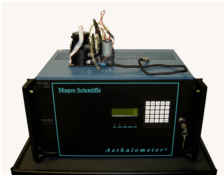
Fig. 3. Absorption photometer developed for deployment on AUAVs sitting atop the original commercial instrument (Magee Scientific AE-31 Aethalometer).
