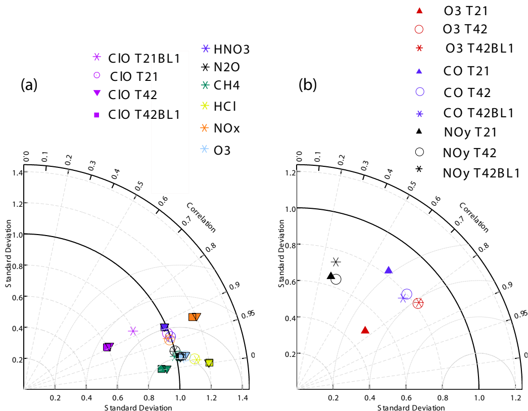
Fig. 21. Taylor type plot of modeled mixing ratios from the T21, T21BL1, T42 and T42BL1 simulations: (a) in the stratosphere 100-1 hPa against the Gross and Russel (2005) and Randel et al. (1998) climatologies. (b) in the UTLS, 340–350 K layer against MOZAIC data. (c) in the troposphere against the Logan (1999a) climatology, over various latitude bands, latitudes higher than 60 S or 60 N (H), latitudes between 30 N and 30 S (T), and mid-latitudes (M), and for two pressure layers, 1000–800 hPa and 800–400 hPa.
