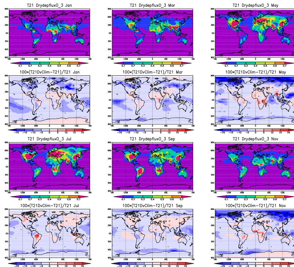
Fig. 22. MOCAGE-Climat T21 O 3 dry deposition fluxes (gm -2 month -1 ), and relative differences (100 × ((T21DvClim - T21) / T21)), in January (left, 2 upper panels), March (middle, 2 upper panels), May (right, 2 upper panels), July (left, 2 bottom panels), September (middle, 2 bottom panels), and November (right, 3 bottom panels).
