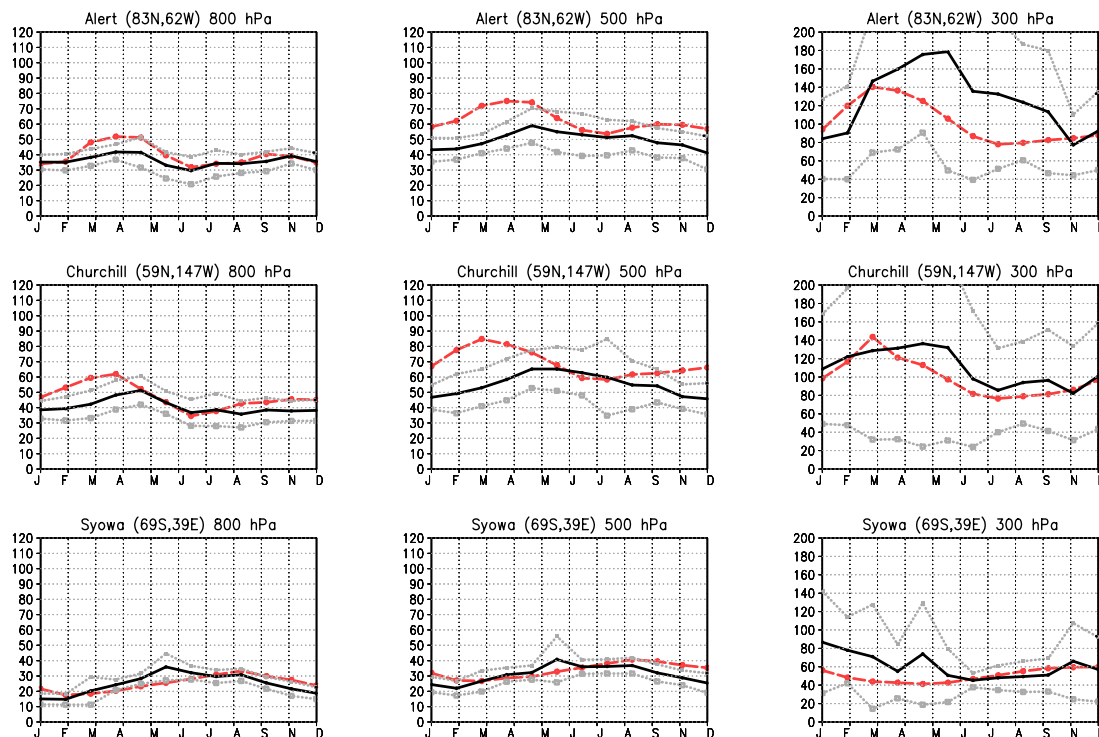
Fig. 19. MOCAGE-Climat monthly O 3 mixing ratios (ppbv) at three different pressure levels, 800 (left), 500 (middle), and 300 hPa (right), against Logan (1999a) observations (black curve, \pm 1 standard deviation as grey curves). MOCAGE-Climat T21 simulations appear as the red curves.
