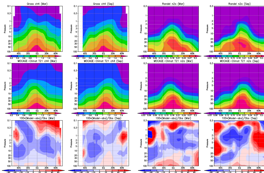
Fig. 3. First two columns: MOCAGE-Climat T21 zonal monthly mixing ratios of \text{CH}_4 (ppmv) against the Gross and Russel (2005) climatology, and relative differences ( 100 \times (\text{Model} - \text{Obs}) / \text{Obs} ), between 100 and 0.1 hPa, in March (left panels) and September (right panels). Last two columns: MOCAGE-Climat T21 zonal monthly mixing ratios of \text{N}_2\text{O} (ppmv) against the Randel et al. (1998) climatology, and relative differences ( 100 \times (\text{Model} - \text{Obs}) / \text{Obs} ), between 100 and 0.3 hPa, in March (left panels) and September (right panels).
