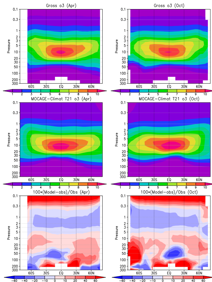
Fig. 16. MOCAGE-Climat T21 zonal monthly mixing ratios of \text{O}_3 (ppmv) against the Gross and Russel (2005) climatology, and relative differences ( 100 \times ((\text{Model} - \text{Obs}) / \text{Obs}) ), between 300 and 0.1 hPa, in April (left panels) and October (right panels).
