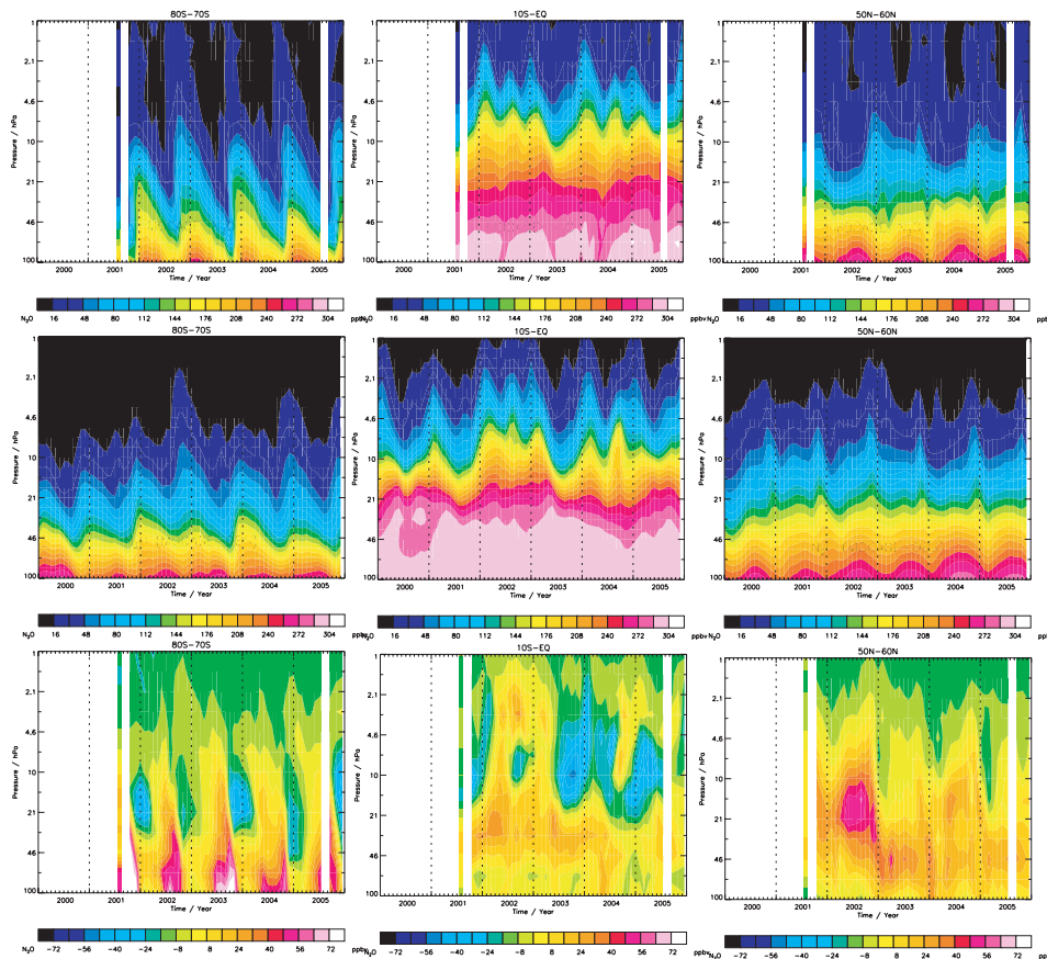
Fig. 7. Time/pressure series for N_2O zonally averaged bands of 10 degrees, 80 S–70 S (left panels), 10 S-EQ (middle panels) and 50 N–60 N (right panels), for ODIN observations (upper line, in white no observations), simulated by MOCAGE-Climat (middle line) and absolute differences (model - observations) (ppbv) (bottom line).
