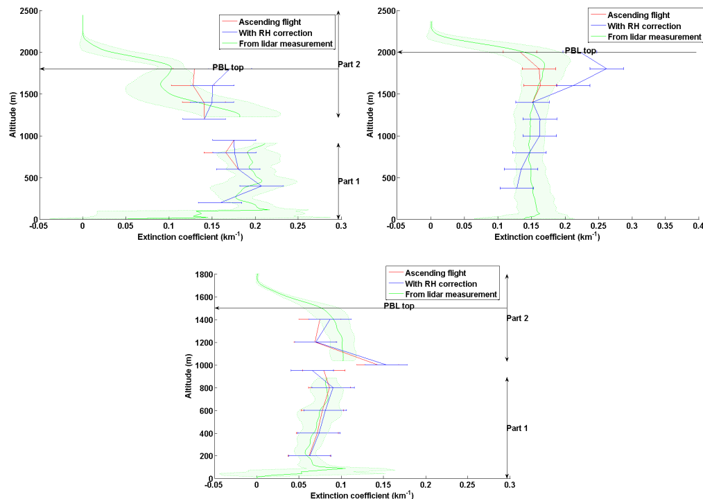
Fig. 7. Vertical profiles of extinction coefficient on 19 (a), 20 (b) and 31 (c) July 2000 over Paris area. Red solid lines represent the mean profile obtained during the ascending part of the flight and horizontal lines give the uncertainties determined by a Monte-Carlo method. Blue solid lines represent the mean profile obtained by a simulation combining in situ retrievals and relative humidity profiles together with their uncertainties. Green solid line represents the mean lidar profile obtained on the leg located over the ascending parts of the flight; shaded areas show the standard deviation on lidar measurements.
