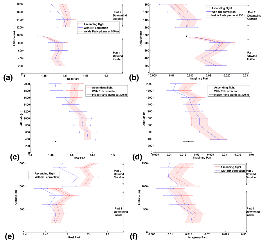
Fig. 3. Vertical profiles of the complex refractive index (real (a, c and e) and imaginary (b, d and f) parts), on 19 (a, b), 20 (c, d) and 31 (e, f) July 2000 over Paris area. Red solid lines represent the mean profile obtained during the ascending parts of the flight, shaded areas show their respective standard deviation and horizontal lines give the uncertainties determined by a Monte-Carlo method. Blue solid lines represent the mean profile obtained by a simulation combining in situ retrievals and relative humidity profiles, and horizontal lines show the uncertainties determined by a Monte-Carlo method.
