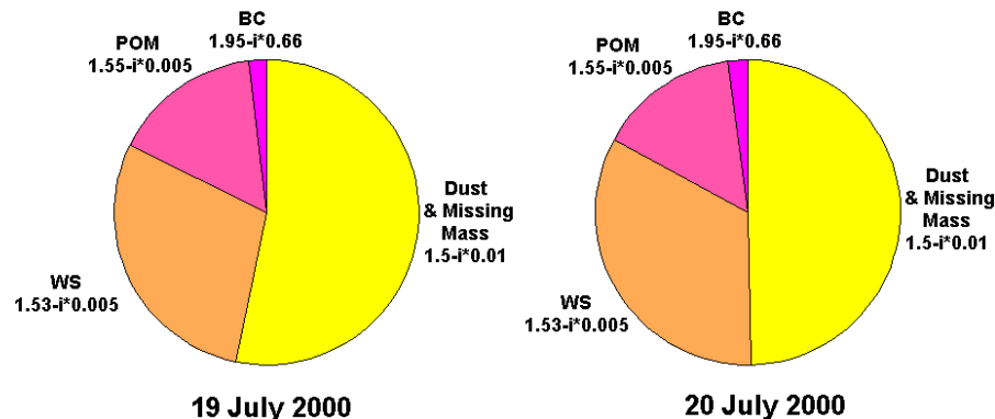
Fig. 6. Mass apportionment and the corresponding values of ACRI derived from chemical analyses on filters for 19 and 20 July 2000. ACRI for black carbon (BC) are from Ackerman and Toon (1981), Faxvog and Roessler (1978), particulate organic matter (POM) from Sloane (1984), Holben et al. (1991), Anderson et al. (1996), Von Hoyningen et al. (1998), water soluble fraction (WS) from Sloane (1984), Volz (1973), Dust from d'Almeida et al. (1991).
