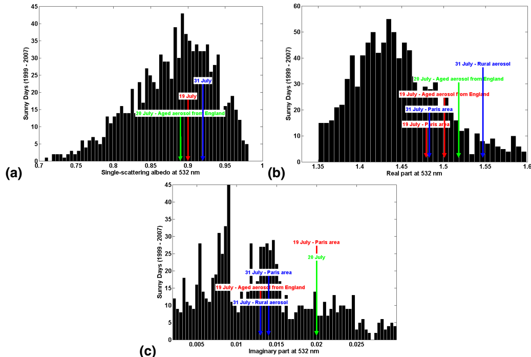
Fig. 5. Histogram of the 532 nm single-scattering albedo (a) , real part (b) and imaginary part (c) of the ACRI for clear-sky conditions during summertime between 1999 and 2007 in the Paris area and retrieved from AERONET Almucantar measurements. The mean values of the present study for 19, 20 and 31 July 2000 are indicated.
