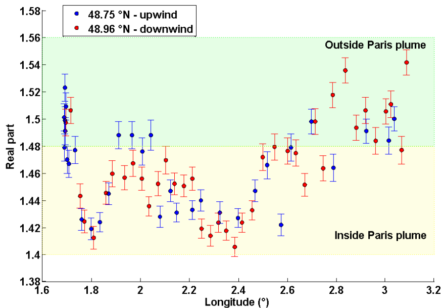
Fig. 4. Evolution of the real part of the ACRI during the leg performed at 950 m as a function of longitude for 31 July 2000. Blue dots correspond to measurements at the latitude of 48.75° N (upwind of Paris) and red dots to measurements at 48.96° N (downwind of Paris). Vertical bars show the uncertainties.
