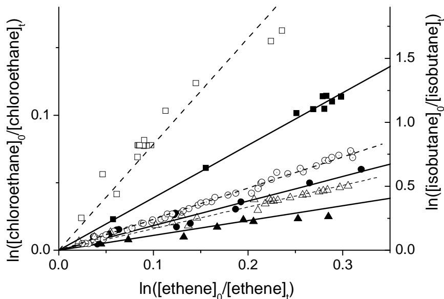
Fig. 11. Plots of \ln([\text{reference}]_0/[\text{reference}]_t) versus \ln([\text{ethene}]_0/[\text{ethene}]_t) obtained with the FTIR. Dashed lines (with open symbols), and solid lines (with filled symbols) indicate measurements using chloroethane, and isobutane as the reference, respectively. Triangles, circles, and squares correspond to measurements at 1000, 400, and 100 mbar, respectively.
