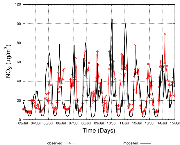
Fig. 11. Observed and modelled NO 2 time series at Olkusz; 2–14 July, hourly values.
