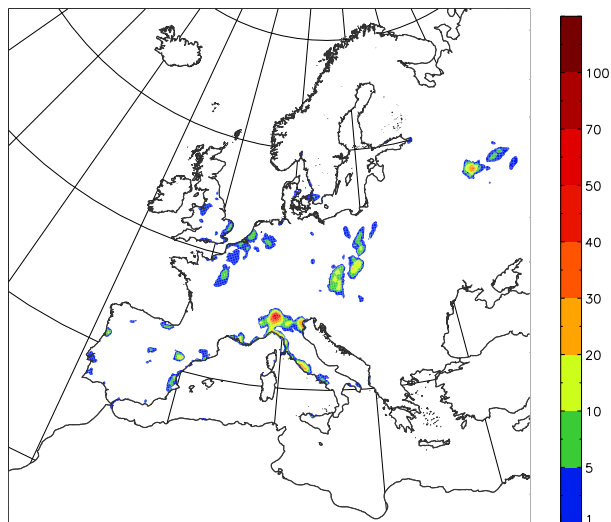
Fig. 18. Number of hours with ozone concentrations exceeding the information threshold ( 180 \mu\text{g m}^{-3} ).
