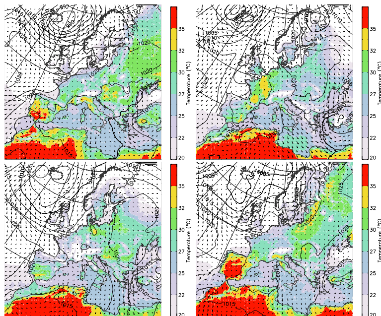
Fig. 1. Synoptic situations: (a) 4 July, 12:00 UTC, (b) 6 July, 12:00 UTC, (c) 10 July, 12:00 UTC, (d) 12 July, 12:00 UTC
