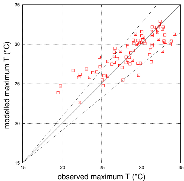
Fig. 10. Scatter plot of observed and modelled daily maximum temperature.
