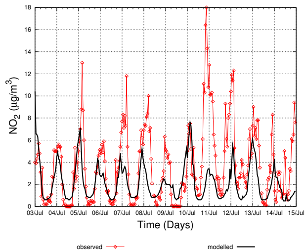
Fig. 12. Observed and modelled NO 2 time series at Mscigniew; 2–14 July, hourly values.
