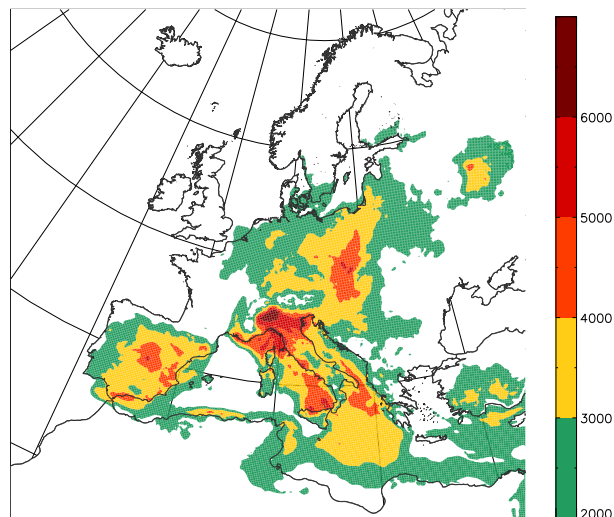
Fig. 21. AOT40 index [ppb days] calculated for the simulation period.
