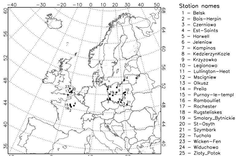
Fig. 3. Monitoring stations used for analysis.
