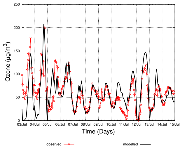
Fig. 4. Observed and modelled ozone time series at Rochester; 3–14 July, hourly values.
