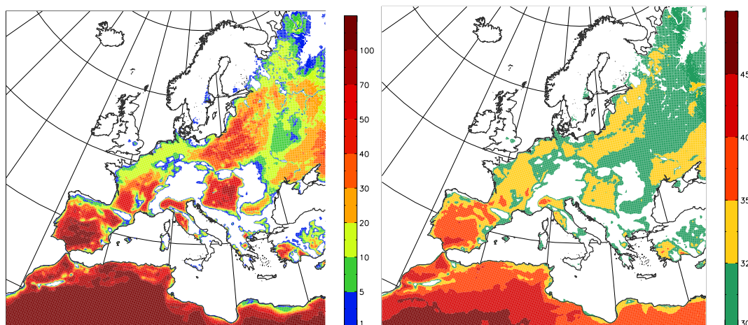
Fig. 17. Heat wave exposure; (a) number of hours with temperature exceeding 30°C over the simulation period, (b) maximum modelled air temperature over the simulation period.
