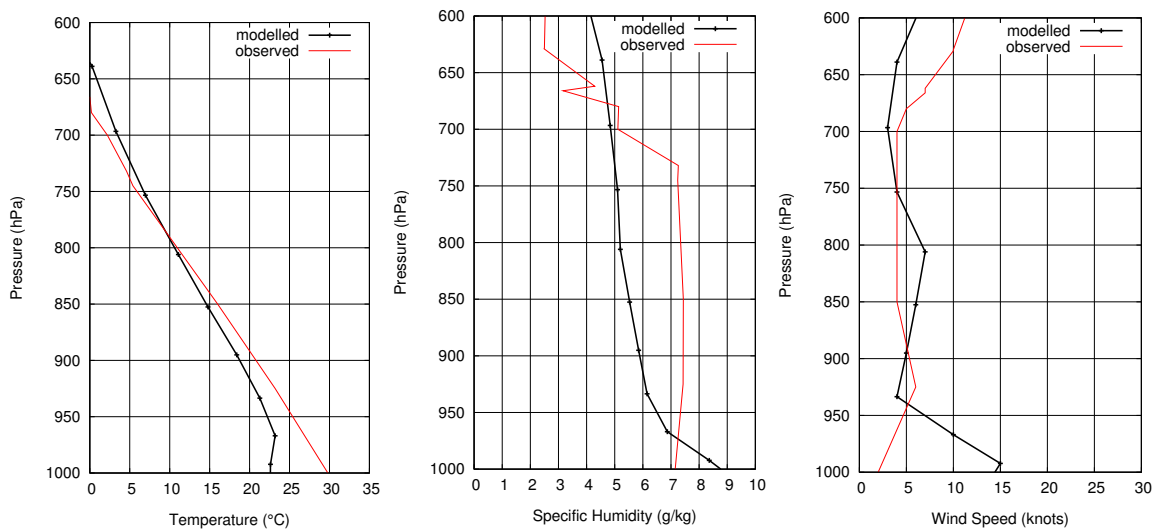
Fig. 15. Observed and modelled vertical profiles for Legionowo on 12 July, 12:00 UTC; (a) temperature, (b) specific humidity, (c) wind speed.
