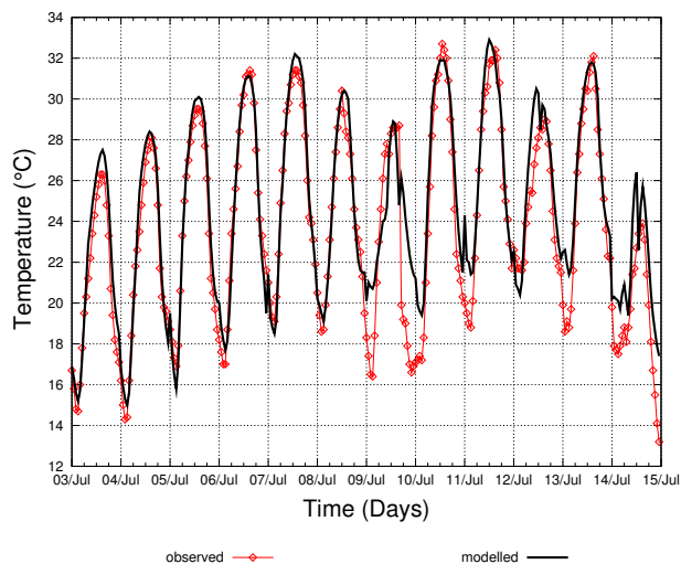
Fig. 9. Observed and modelled temperature time series at Mscigniew; 2–14 July, hourly values.
