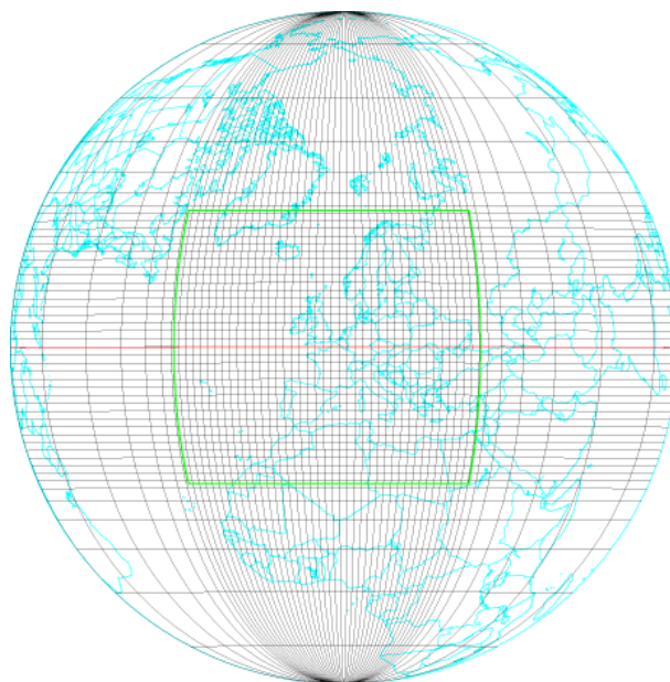
Fig. 2. Global variable resolution model domain (every 10th grid line is plotted).
