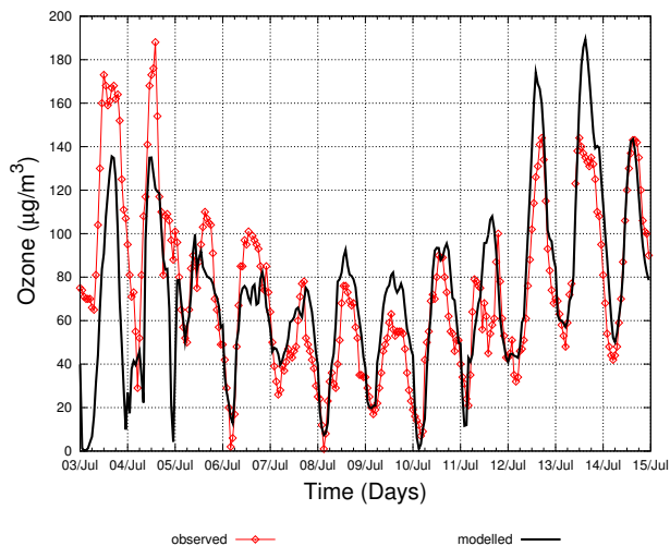
Fig. 5. Observed and modelled ozone time series at Rambouillet; 3–14 July, hourly values.
