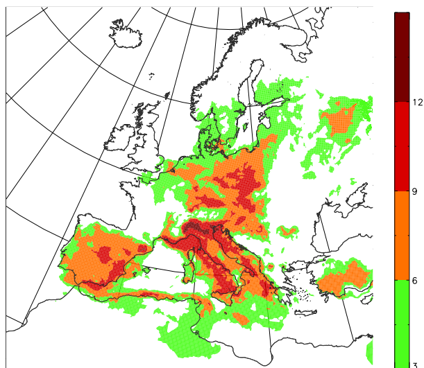
Fig. 19. Number of days with maximum 8-h ozone average exceeding 120 \mu\text{g m}^{-3} .
