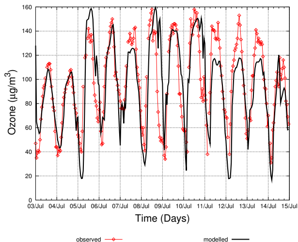
Fig. 7. Observed and modelled ozone time series at Zloty Potok; 3–14 July, hourly values.
