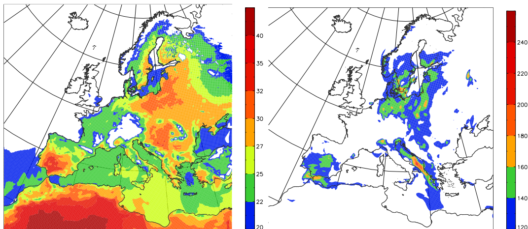
Fig. 16. Heat wave indicators; (a) 8-h averaged temperature for 8 July, (b) maximum 8-h average ozone concentrations for 8 July.
