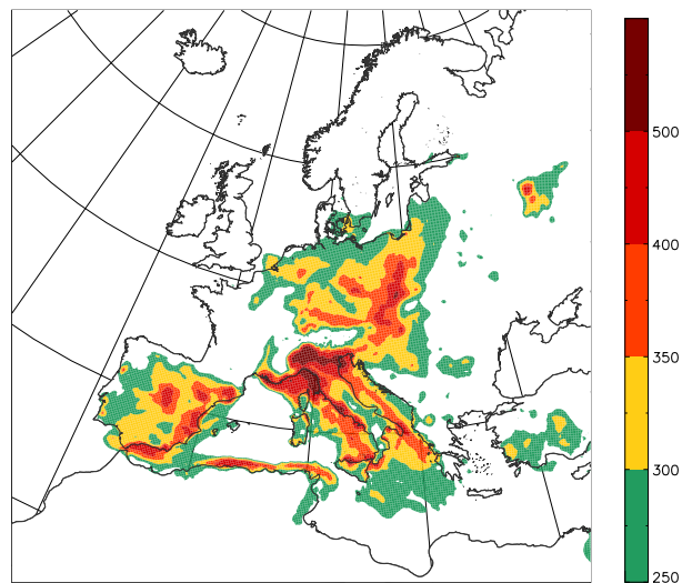
Fig. 20. SOMO35 index [ppb days] calculated for the simulation period.
