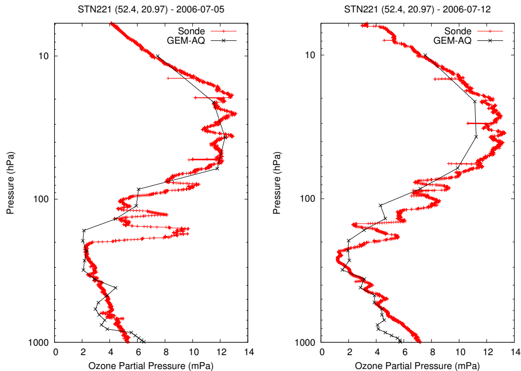
Fig. 13. Observed and modelled ozone vertical soundings from Legionowo; (a) 5 July, 12:00 UTC, (b) 12 July, 12:00 UTC.
