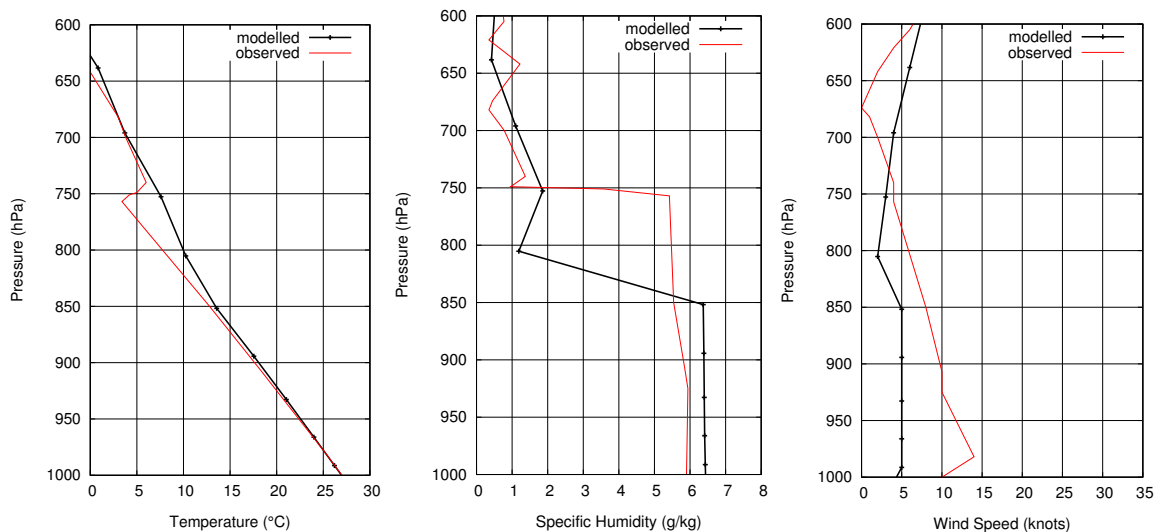
Fig. 14. Observed and modelled vertical profiles for Legionowo on 5 July, 12:00 UTC; (a) temperature, (b) specific humidity, (c) wind speed.
