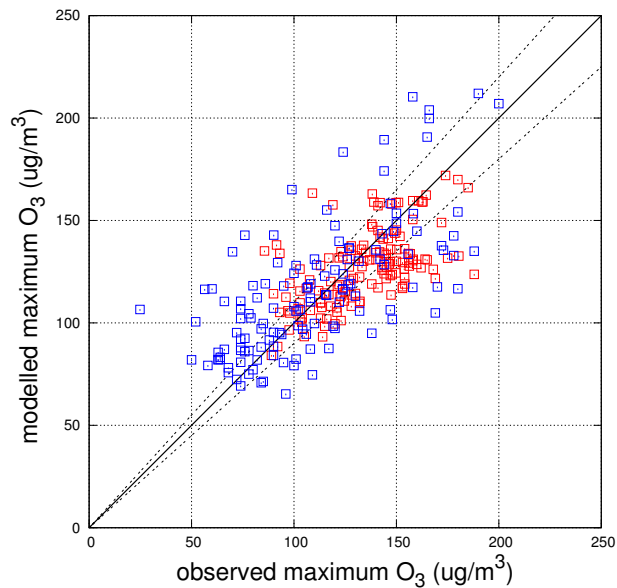
Fig. 8. Scatter plot of observed and modelled ozone maximum concentrations (red – Central Europe; blue – Western Europe).
