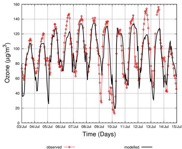
Fig. 6. Observed and modelled ozone time series at Mscigniew; 3–14 July, hourly values.
