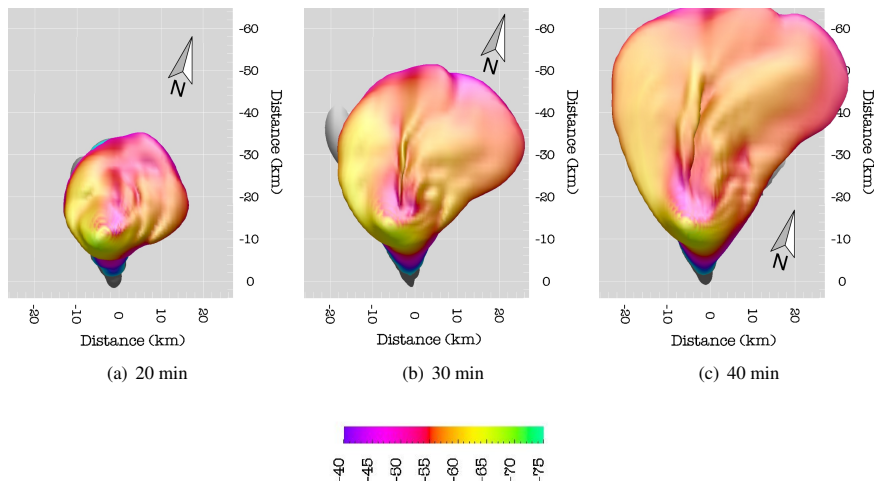
Fig. 5. Cloud top temperatures in °C on the 0.5 \text{ g kg}^{-1} hydrometeor concentration isosurface as simulated by ATHAM for three instances in time.
