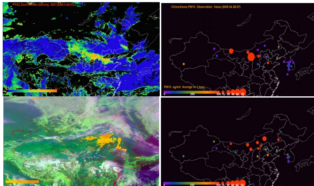
Fig. 5. FY-2C IDDI comparison with PM10 value 28–29 April 2005.
