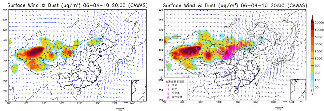
Fig. 6. Comparisons of CUACE/Dust forecasting results for 10 April 2006 with and without data assimilation.
