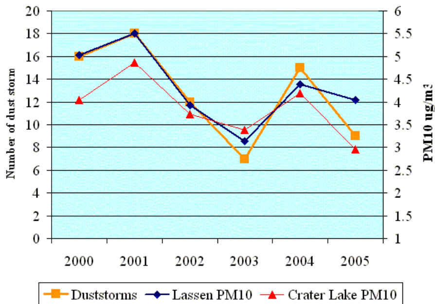
Fig. 3. Relationship between the annual spring (March-May) mean PM10 concentration at 2 sites in the western U.S. and SDS process numbers in China from 2000 to 2005. The 2 sites are Lassen, CA; Crater Lake, OR.
