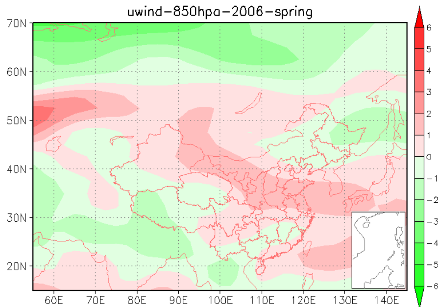
Fig. 2. Zonal wind anomalies at 850 hPa for spring 2006.
