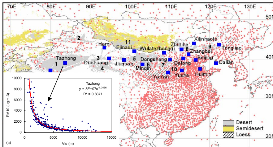
Fig. 4. SDS observation stations in CMA. The red dots are meteorological stations with visual visibility measurements and the blue squares are SDS observation stations with PM10 and instrumental visibility measurements. Insert: Relationship between hourly-averaged PM10 concentration and visibility during SDSMI events in the springtime at Tazhong station.
