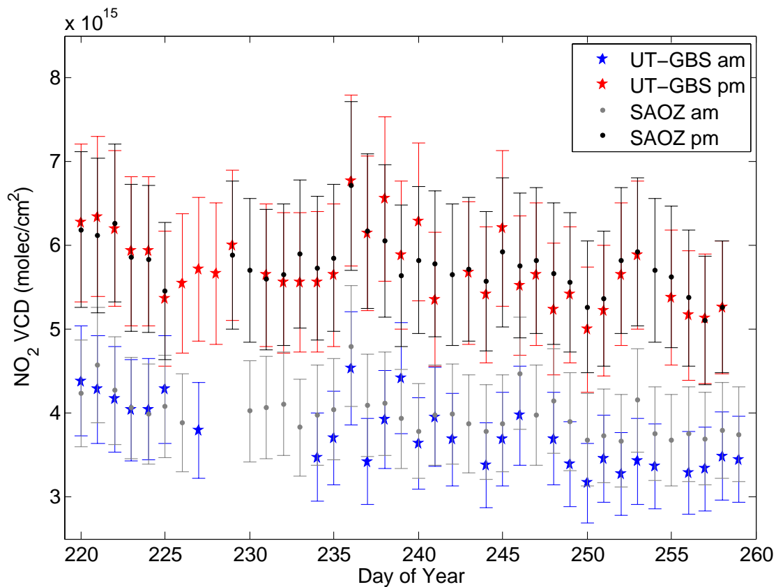
Fig. 6. NO 2 vertical column densities as measured by the UT-GBS and SAOZ.
