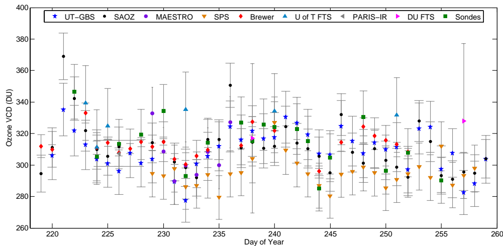
Fig. 5. Daily-averaged ozone vertical column densities as measured by the UT-GBS, SAOZ, MAESTRO, SPS, the Brewer, the U of T FTS, the DU FTS, PARIS-IR, and ozonesondes.
