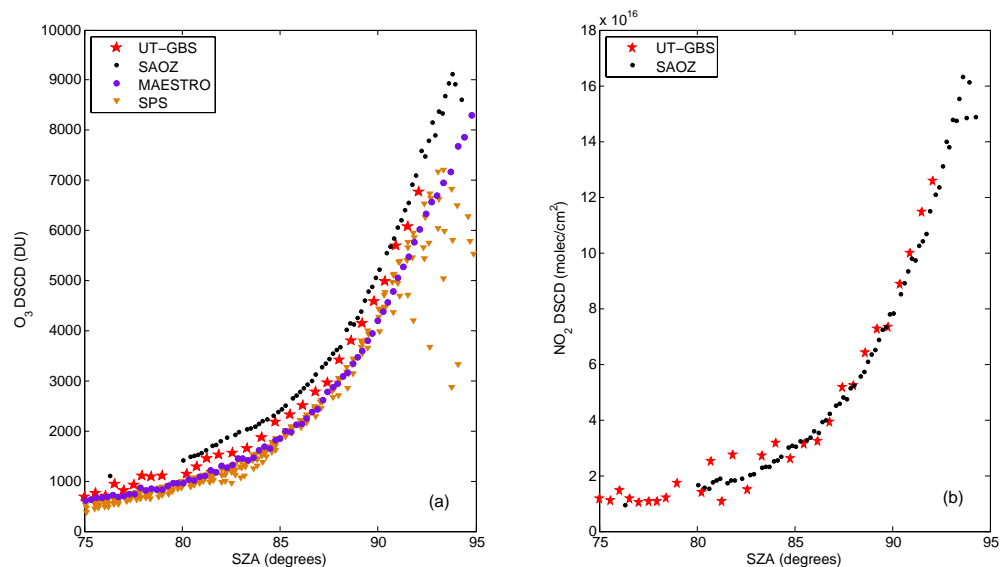
Fig. 1. (a) Ozone differential slant column densities for the UT-GBS, SAOZ, MAESTRO, and SPS for sunset of 20 August 2004. (b) As (a), but NO 2 and for SAOZ and the UT-GBS.
