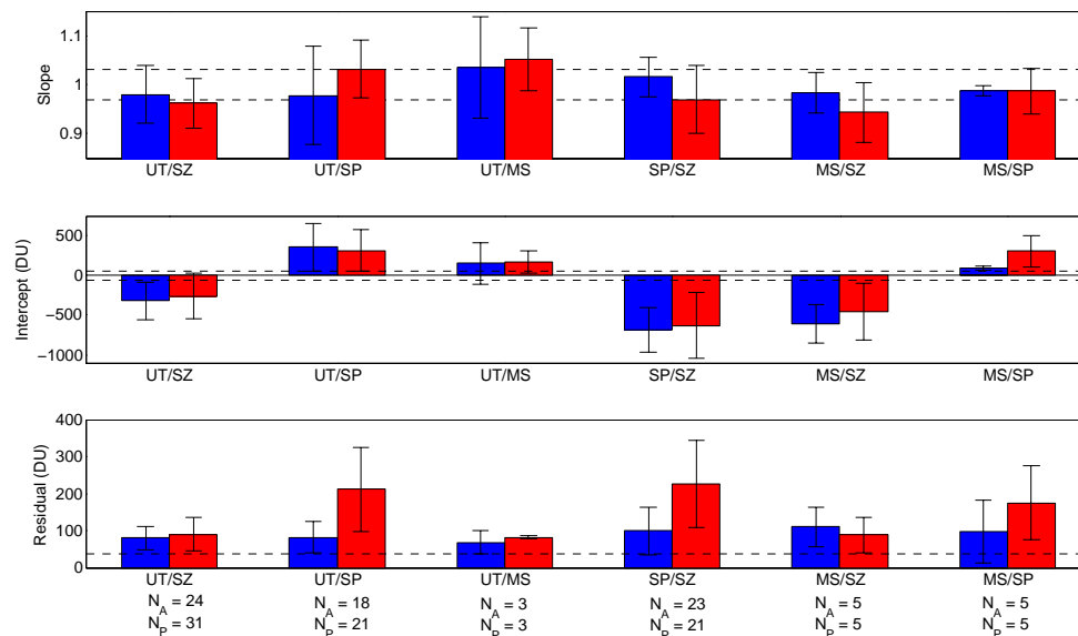
Fig. 3. Type 1 regression analysis results for ozone for all pairs of UV-visible zenith-sky instruments. Dashed horizontal lines indicate the required accuracies set by the NDACC. Blue is for the morning comparisons, red is for the afternoon. UT indicates the UT-GBS, SZ is SAOZ, SP is SPS, and MS is MAESTRO. N_A and N_P are the number of days used in calculating the morning and afternoon averages.
