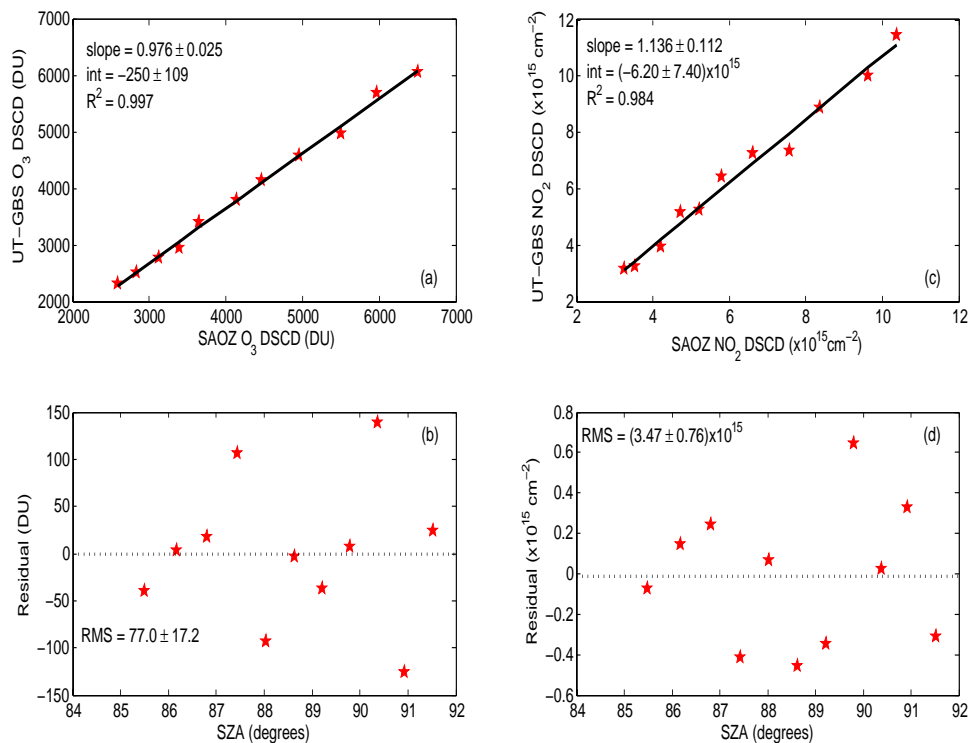
Fig. 2. (a) Type 1 regression analysis for ozone between UT-GBS and SAOZ for sunset, 20 August, (b) residuals of the fit in (a), (c) same as (a) but for NO 2 , (d) same as (b) but for NO 2 .
