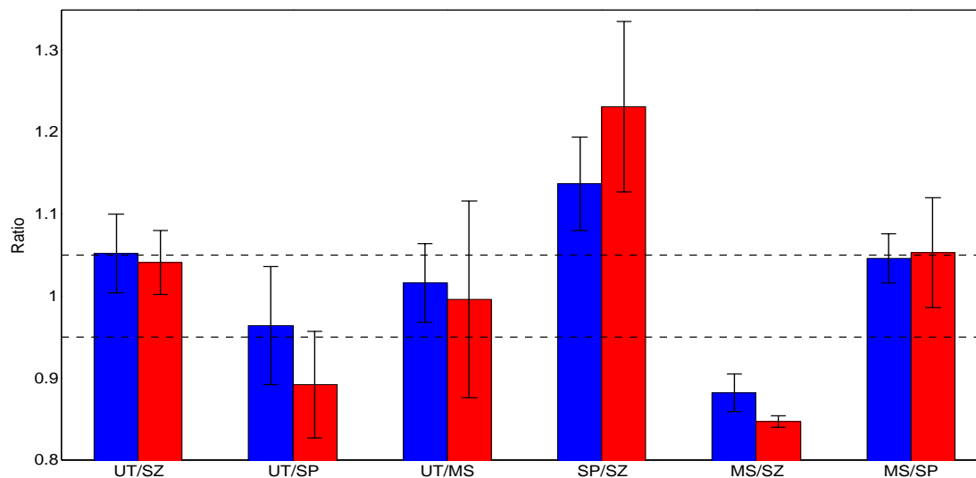
Fig. 4. Type 2 regression analysis results for ozone for all pairs of UV-visible zenith-sky instruments. Dashed horizontal lines indicate the required accuracy set by the NDACC. Blue is for the morning comparisons, red is for the afternoon. The number of days used in the average is the same as for the Type 1 comparisons (Fig. 3).
