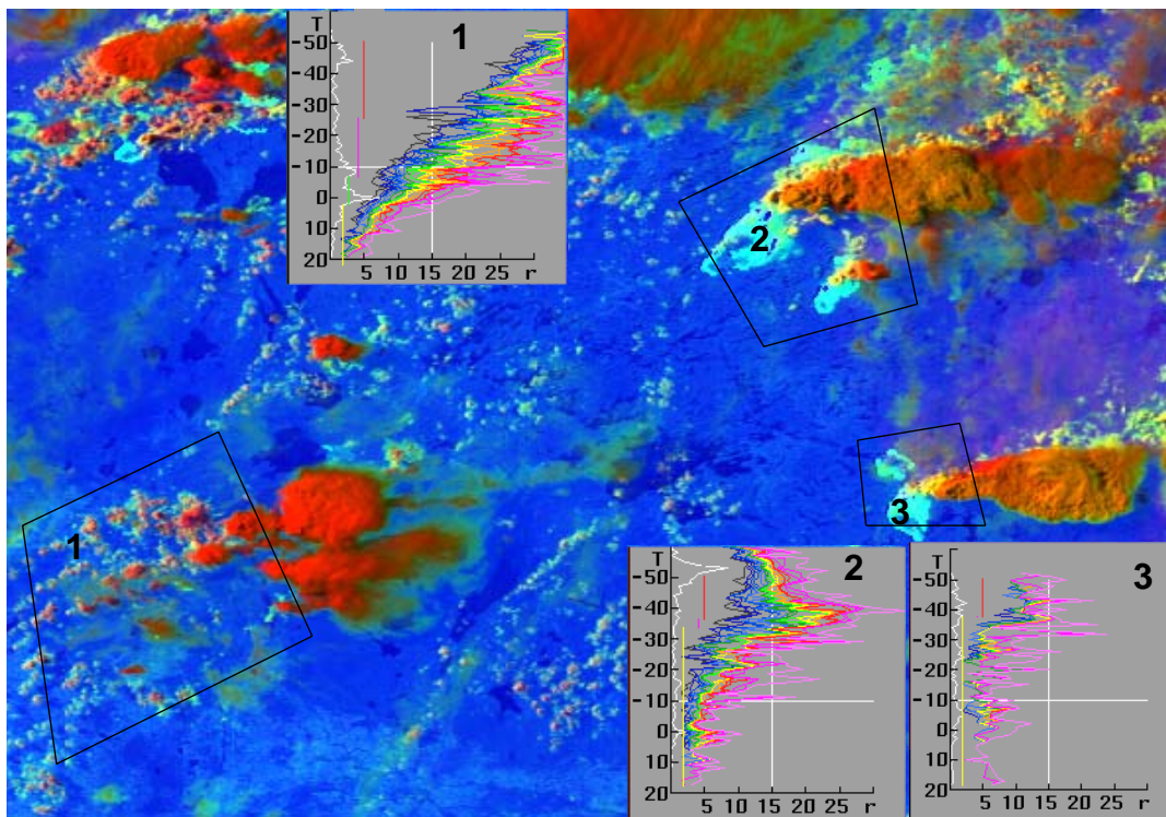
Fig. 11. Analysis of cloud top structure of two pyro-Cbs in Canada at 55^{\circ}\text{N} 105^{\circ}\text{W} and at 57^{\circ}\text{N} 105^{\circ}\text{W} and adjacent clouds, based on the NOAA-AVHRR overpass on 27 June 2002, 23:59 UTC. The T - r_e of a natural Cb (Area 1) and of the two pyro-Cb clouds (Areas 2 and 3) show a similar microstructure as for the clouds in the Chisholm event. Cloud 3 is capped at -50^{\circ}\text{C} and is apparently not overshooting at the time of the image. However it does have extremely small r_e up to the homogeneous freezing level of -38^{\circ}\text{C} , where the drops must freeze into ice particles with apparently very small indicated r_e . The r_e of the unperturbed cloud exceeds the precipitation threshold of \sim 15\ \mu\text{m} at the -10^{\circ}\text{C} isotherm level.
