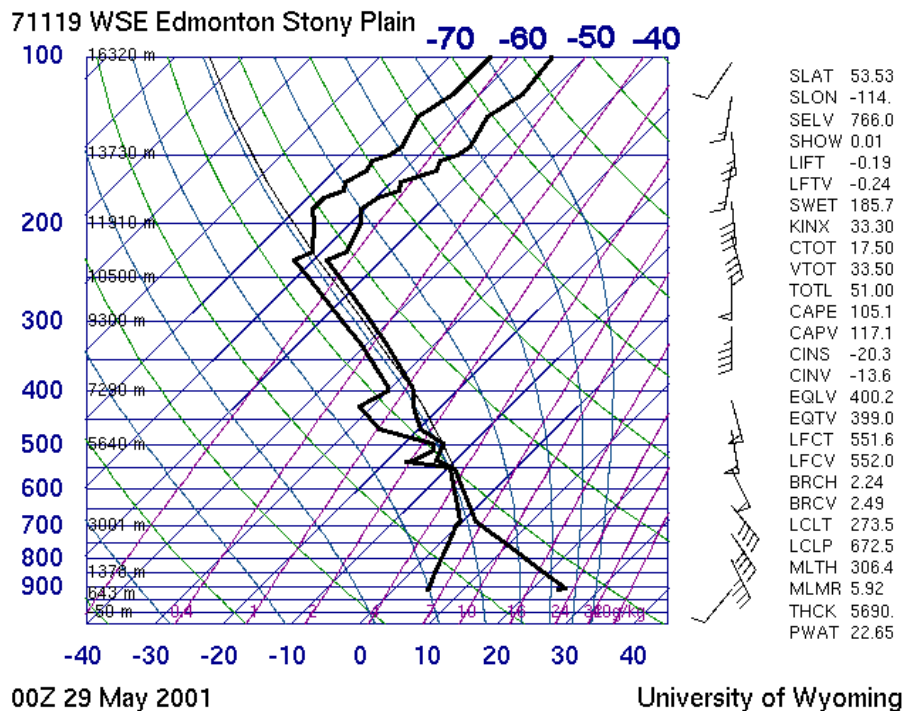
Fig. 3. The Edmonton sounding on 29 May 2001, 00:00 UTC.
