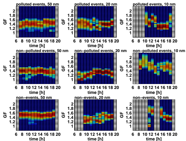
Fig. 11. Daytime median growth factor spectra during new particle formation event days and non-event days for 50 nm, and 20 nm and 10 nm particle sizes at Thrakomakedones, Athens. Events days were divided into polluted and non-polluted days based on meteorological conditions.
