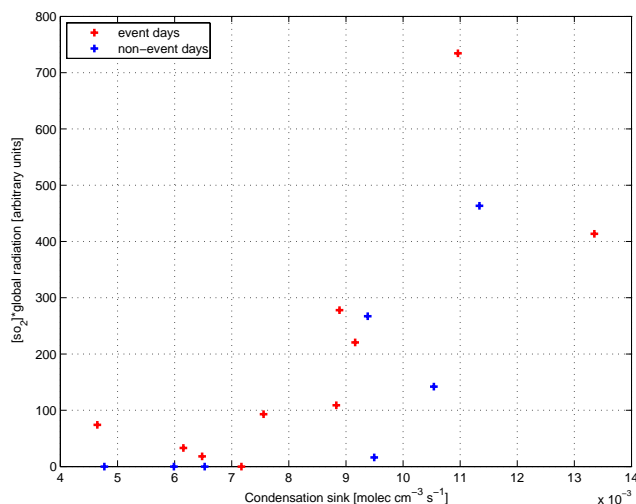
Fig. 9. A product of global radiation and sulphur dioxide as a function of condensation sink as an 4 h average (10:00–14:00) at Plan d'Aups. The product is a proxy for sulphuric acid produced from SO 2 in photochemical reactions.
