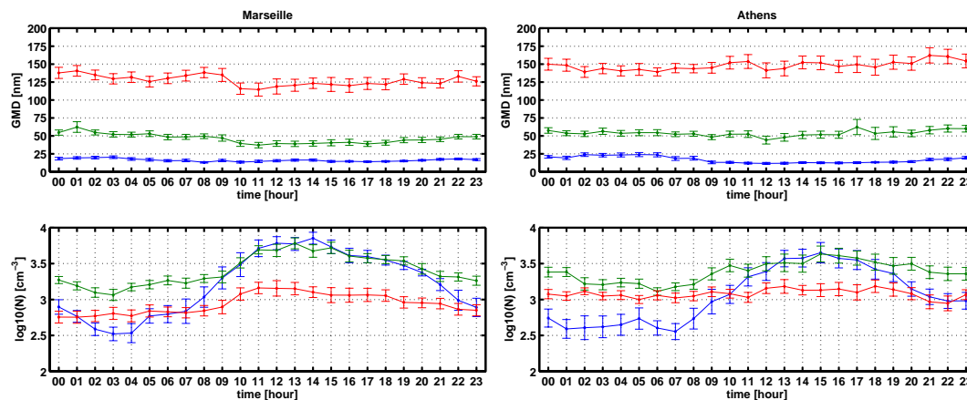
Fig. 3. Average diurnal variation of modal geometric mean diameter (top) and modal concentrations (bottom) at Marseille (left) and at Athens (right). Whiskers in the data points indicate 95% confidence intervals of the averages.
