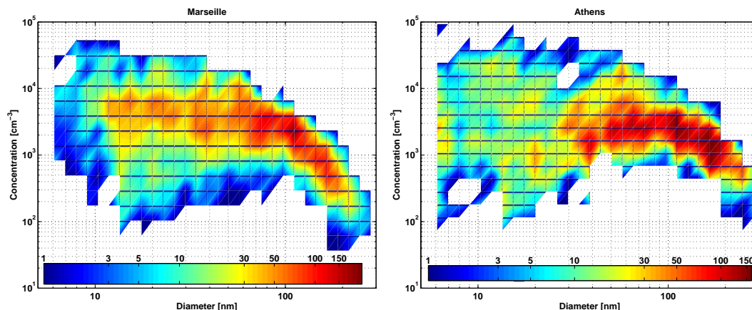
Fig. 4. A histogram plot of fitted modal concentrations as a function of geometric mean diameters for Marseille (left) and Athens (right) field campaigns. Red colors indicate larger frequency of observations at a certain size bin. A persistent accumulation mode at 100–200 nm is present at both sites. Aitken mode (20–80 nm) was, on average, slightly larger at Marseille. Nucleation mode (<20 nm) concentration and size are more variable at Marseille.
