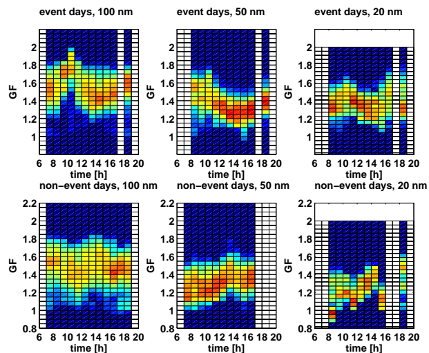
Fig. 10. Daytime median growth factor spectra during new particle formation event days and non-event days for 100 nm, 50 nm and 20 nm particle sizes at Plan d'Aups, Marseille.
