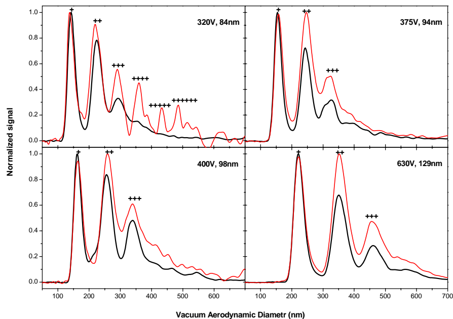
Fig. 4. The effect of conditioning after atomizing on different size selected ( V , 84–129 nm) ABS particles vacuum aerodynamic diameter spectrum. The black full line presents the vacuum aerodynamic diameter of size selected ABS particles which have undergone conditioning followed atomizing. For each size selected figure the red dashed line shows the spectrum without conditioning. Multiply charged particles are indicated by +.
