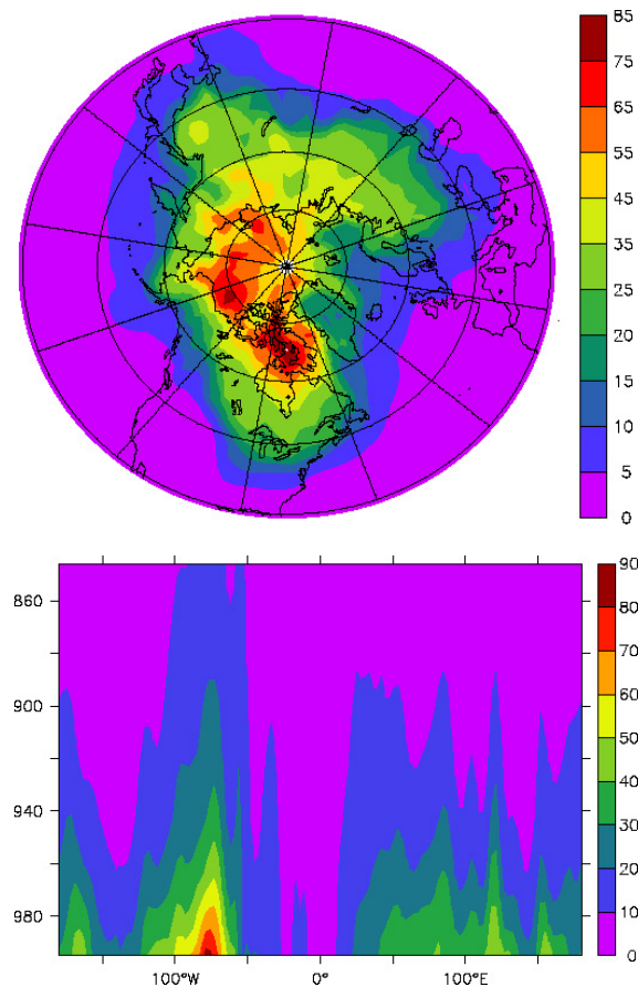
Fig. 5. Relative increase in the mean January Northern Hemisphere surface ozone mixing ratio (%) (a) and up to 850 hPa along 65° N (b) resulting from the decrease of the default ozone deposition velocity of v_{dO_3} \leq 0.05 \text{ cm s}^{-1} to a lower value of v_{dO_3} \leq 0.01 \text{ cm s}^{-1} over snow covered landscapes and sea-ice.
