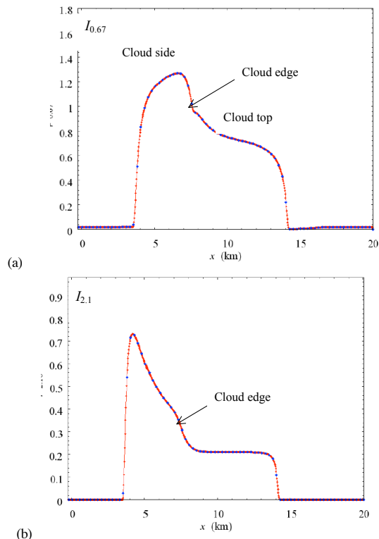
Fig. 2. Reflectance from a single cloud with a variable droplet effective radius. Cloud height h = 4 km, cloud size L = 6.5 km, flat cloud top, \tau = 80 , \theta_o = 60^\circ , \theta = 45^\circ . Droplet effective radius r_e increases linearly with height from 5 to 25 \mu\text{m} . (a) 0.67 \mu\text{m} ; (b) 2.1 \mu\text{m} . Cloud edge is indicated by arrow at x = 7.5 km. Reflectance from cloud top is at the right side from the cloud edge while reflectance from cloud side is at the left. Dots indicate “measurements” at s = 0.25 km resolution.
