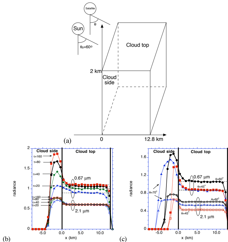
Fig. 1. Reflectance from a single cloud at two wavelengths: 0.67 \mu\text{m} (solid symbols) and 2.1 \mu\text{m} (empty symbols). Cloud height h=2 \text{ km} , cloud width L=12.8 \text{ km} , droplet effective radius, r_e=10 \mu\text{m} , SZA \theta_0=60^\circ (a) A schematic illustration of illumination and viewing angles. Negative x correspond to reflectances from “cloud side” while positive x correspond to reflectances from “cloud top”; (b) \theta=60^\circ ; cloud optical thickness \tau=160, 80, 40 and 20 ; (c) \tau=80 , \theta=70^\circ, 60^\circ and 45^\circ .
