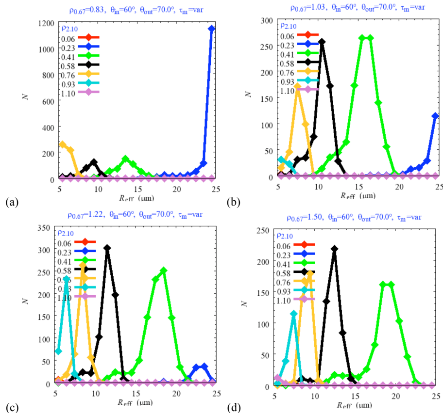
Fig. 7. Histograms (number of cases vs. effective radius) obtained from Fig. 6. Values of reflectance at 0.67 \mu\text{m} were set to 0.83, 1.03, 1.22, and 1.50 with a \pm 0.03 window, on panels (a), (b) (c) and (d) respectively. Values of reflectance at 2.1 \mu\text{m} have a \pm 0.02 window.
