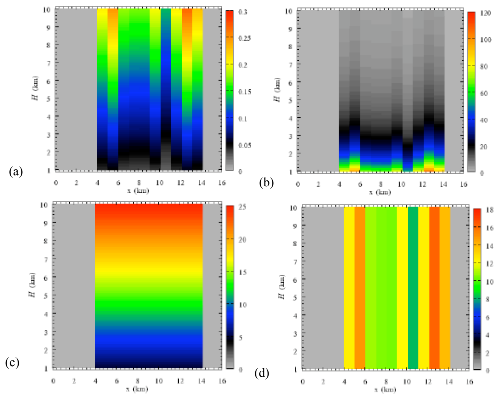
Fig. 4. An example of cloud microphysics. (a) liquid water content, LWC; (b) number of drops, N ; (c) droplet effective radius, r_e ; (d) extinction coefficient, \sigma_{\text{ext}} .
