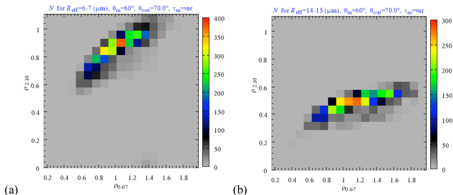
Fig. 8. Histograms of reflectances at 0.67 \mu\text{m} and 2.1 \mu\text{m} conditional the effective radius equal to (a) 6–7 \mu\text{m} and (b) 14–15 \mu\text{m} . Plot is based on 20 realizations of the stochastic cloud model described in Sect. 3. Parameters of the model are the same as in Fig. 6.
