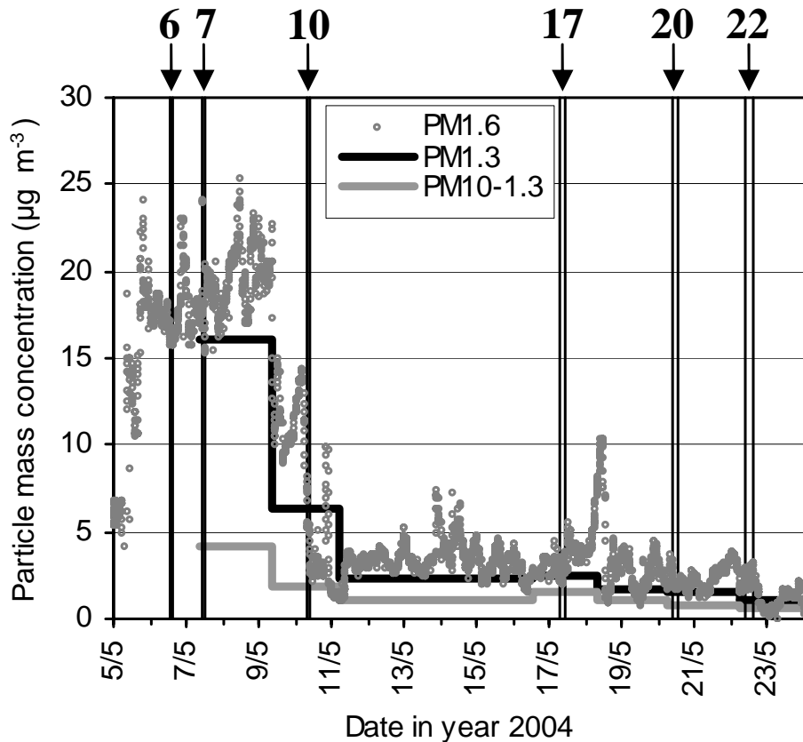
Fig. 1. Particle mass concentrations ( PM_{1.6} measured with ELPI, and PM_{1.3} and PM_{1.3-10} with VI) in Hyytiälä in May 2004. The six sampling periods with the Battelle impactor for TEM/EDX analysis are marked with vertical lines and arrows (sample numbers above).
